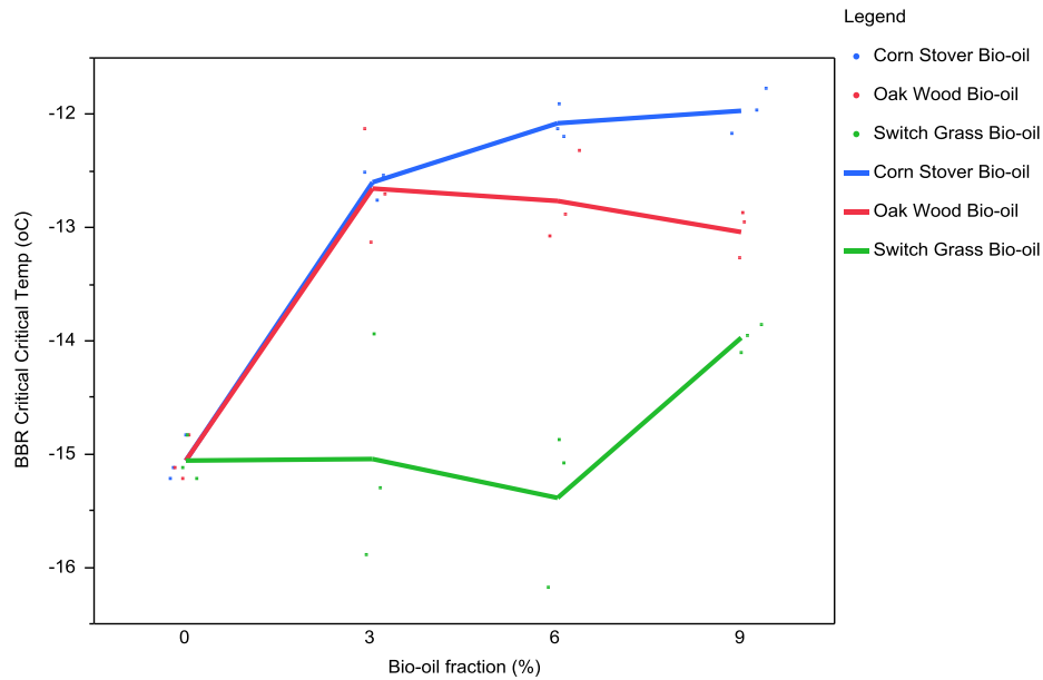
Figure 13. Low Critical Temp for AAM-1 vs. Bio-oil fraction (%) by Bio-oil types
