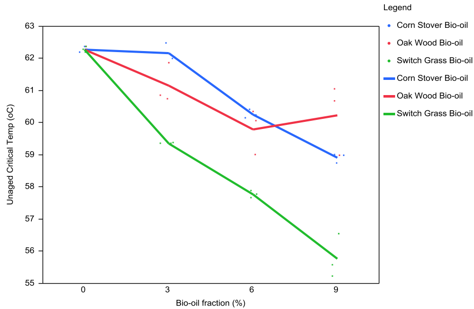
Figure 6. Unaged Critical Temp for AAD-1 vs. Bio-oil fraction (%) by Bio-oil types
