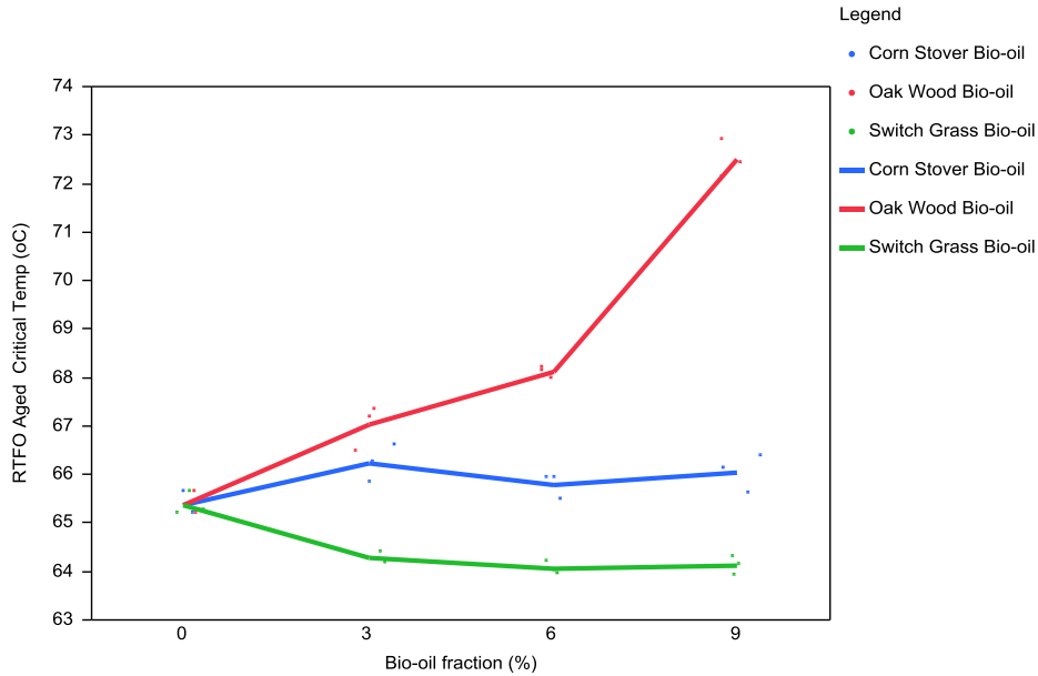
Figure 9. RTFO Critical Temp for AAD-1 vs. Bio-oil fraction (%) by Bio-oil types
