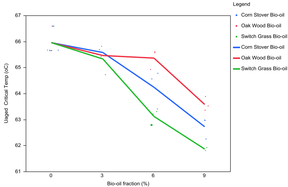
Figure 8. Unaged Critical Temp for LPMB vs. Bio-oil fraction (%) by Bio-oil types
