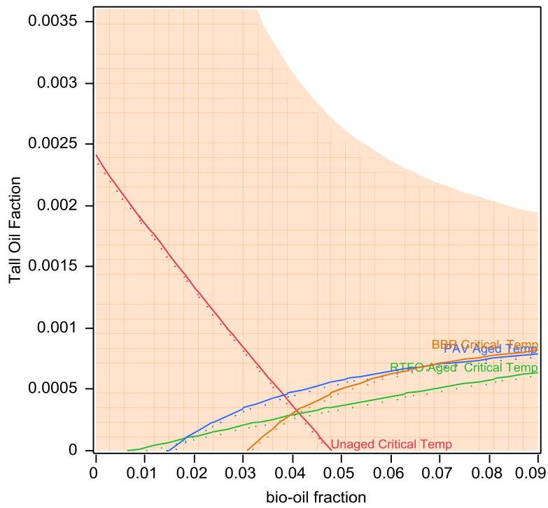
Figure 57. Constraint shading map for AAD-1 with corn stover bio-oil and tall oil
