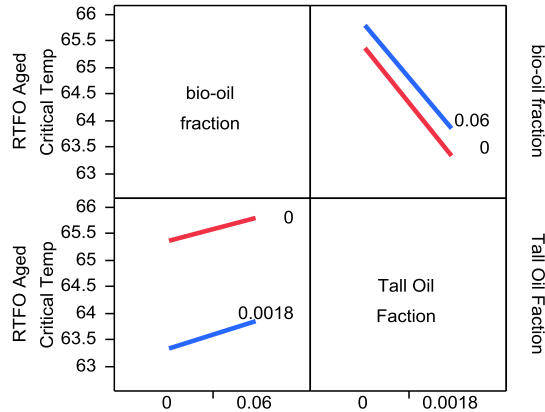
Figure 28. Interaction plots for oak wood bio-oil and tall oil in AAM-1 binder
