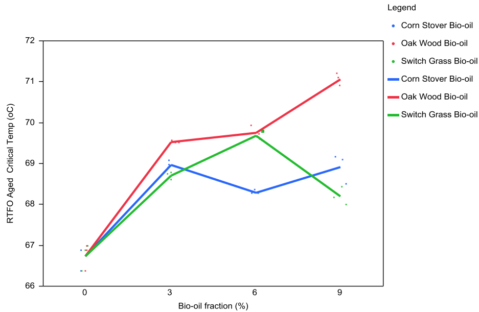
Figure 11. RTFO Critical Temp for LPMB vs. Bio-oil fraction (%) by Bio-oil types
