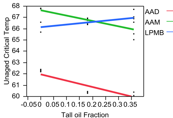
Figure 22. Tendency for unaged critical temperature by varying tall oil treatments
