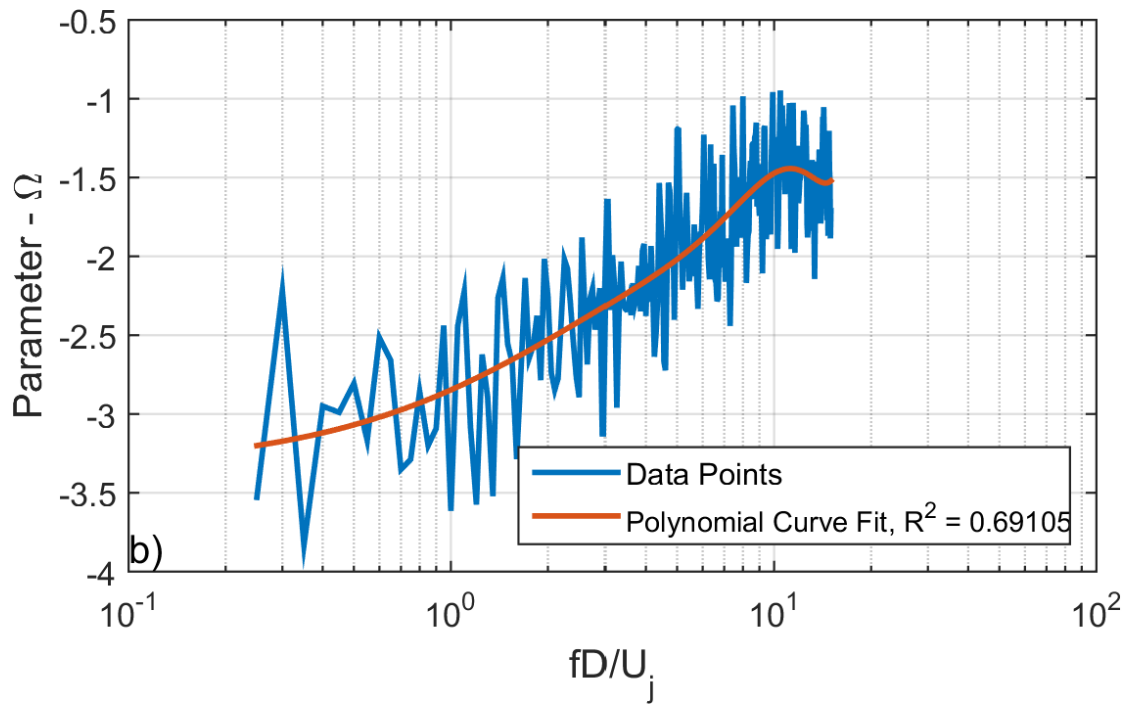
Figure 5.22: Empirically derived curve fits for the \Omega and \Gamma parameters in the \Gamma H^\Omega function.
