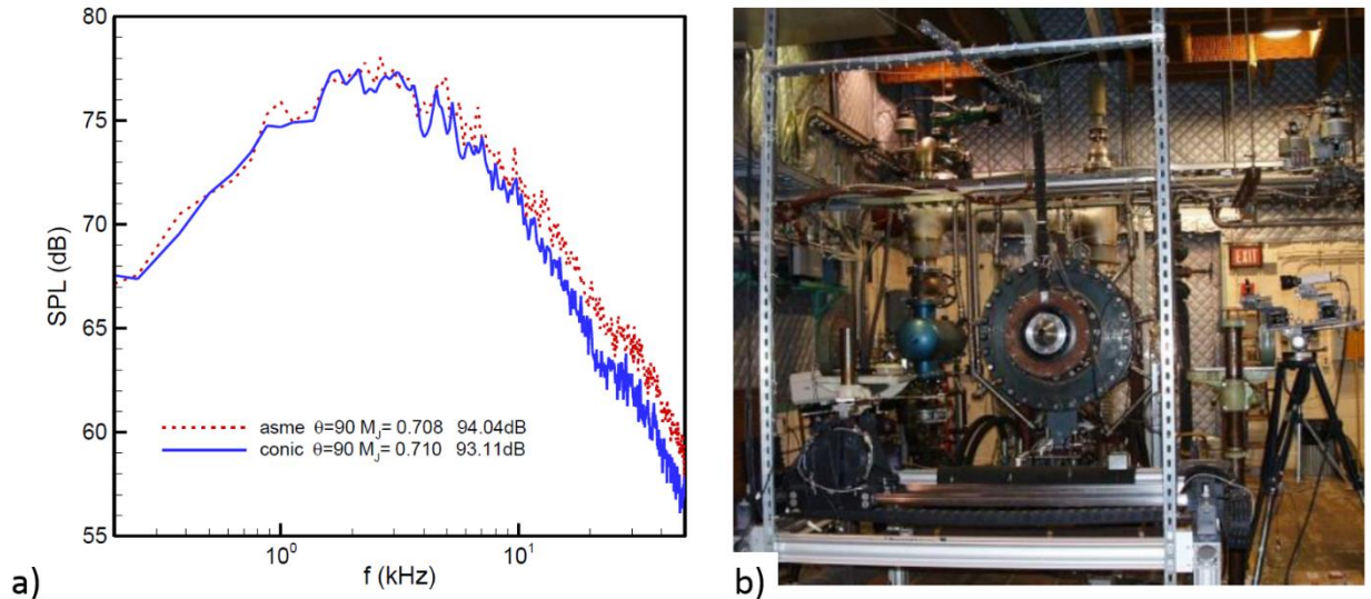
Figure 6.8: (a) Example of jet noise spectra acquired by Zaman 16 and (b) the facility used to acquire the data. (The facility might have been treated for acquiring the acoustic data.)
