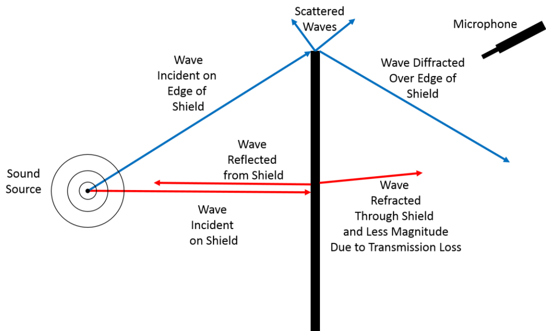
Figure 6.3: Physical mechanisms behind acoustic shielding.
