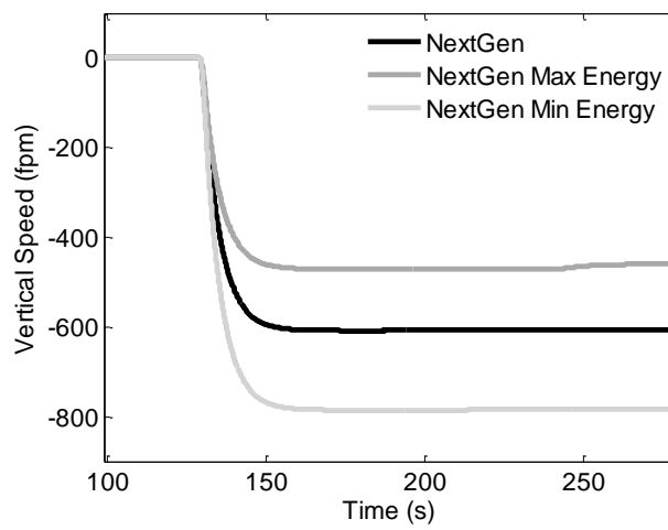
Figure 24. Times Histories for Altitude, Airspeed, and Vertical Speed During the Initial Descent in the NextGen Arrivals
