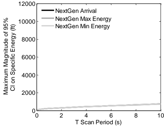
(a) Specific Energy with a T Scan
