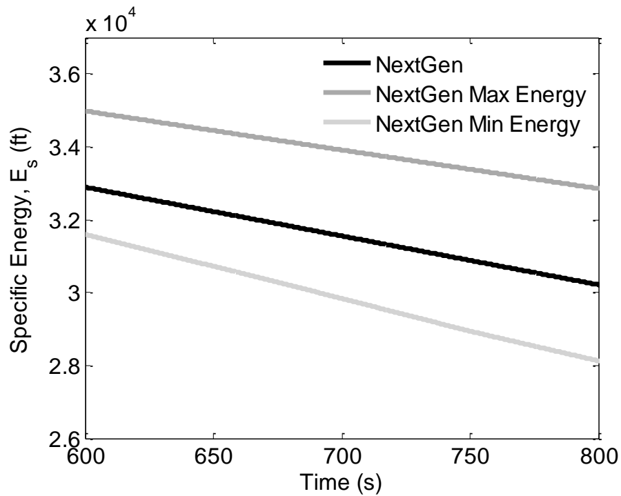
Figure 46. Time History of Specific Energy in an Aircraft Specific Energy Comparison for Each NextGen Arrival
