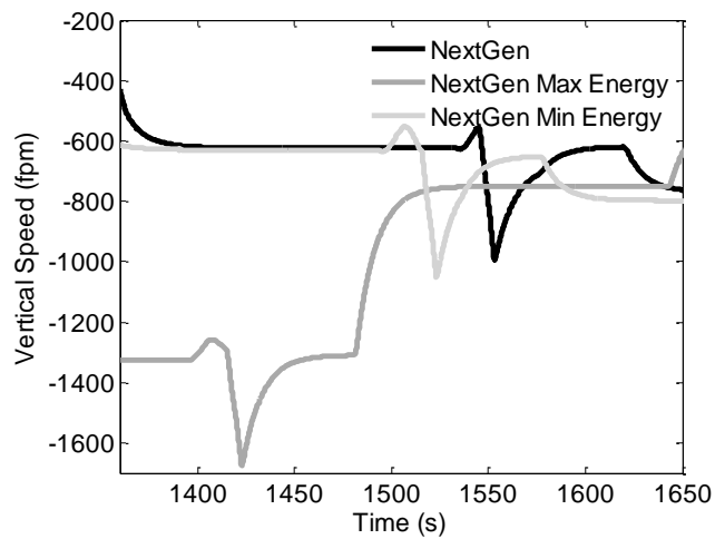
Figure 39. Time Histories of Altitude, Airspeed, and Vertical Speed During a Speed Up Near Landing in the NextGen Arrivals
