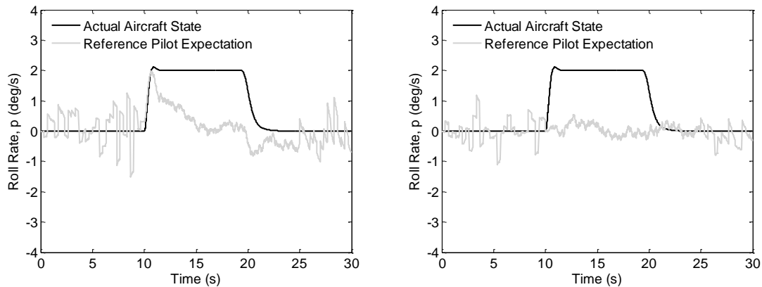
Figure 21. Comparison of the Reference Pilot Expectation of Roll Rate with (left) and without (right) Awareness of Control Surface Deflections with a 15-second Distraction during a Sub-threshold Roll
