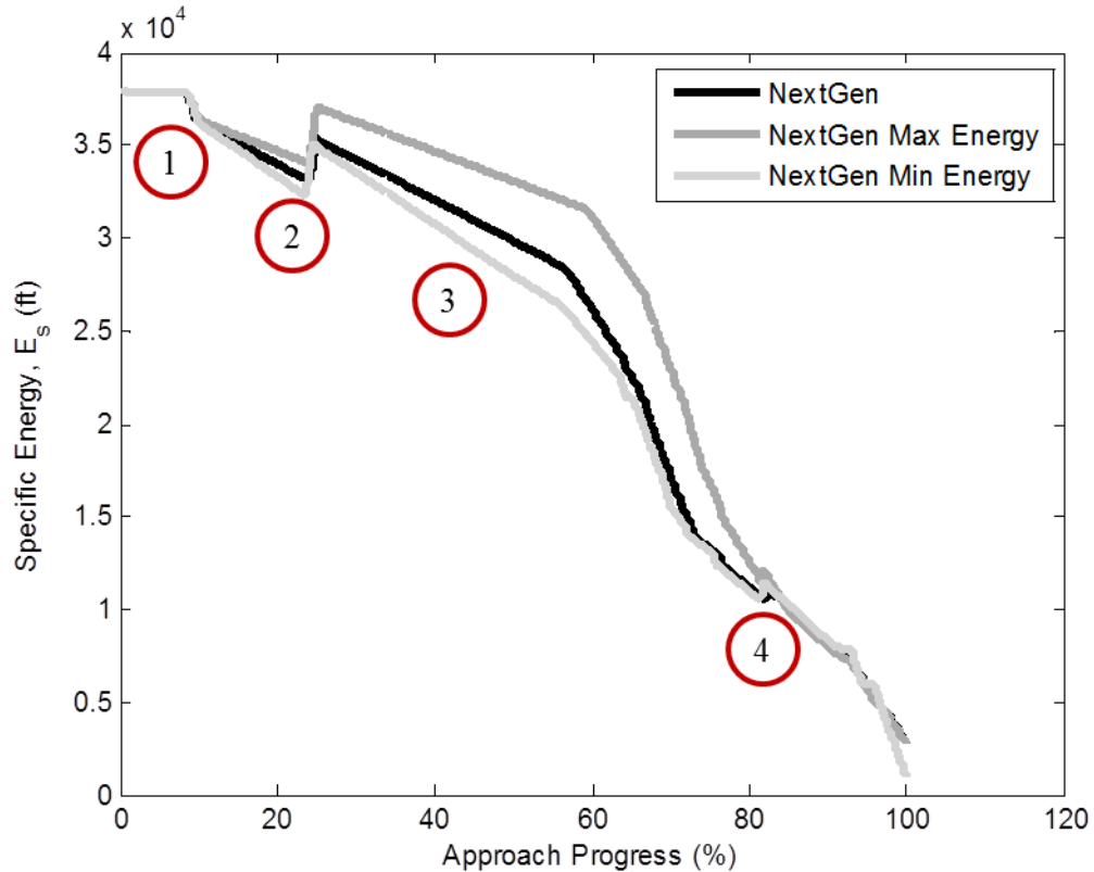
Figure 23. The Four Points of Descent to be Examined in the Energy Profiles of the Three NextGen Arrival Variants
