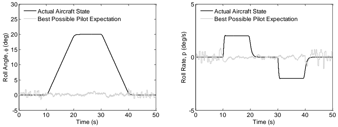
Figure 7. Reference Pilot Expectation of Roll and Roll Rate During a Sub-threshold Bank Maneuver with No Awareness of Control Surface Deflections
