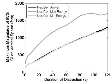
Figure 40. Maximum 95% Confidence Interval of Error in RPE of Altitude, Indicated Airspeed, and Vertical Speed in a Speed Up Near Landing
