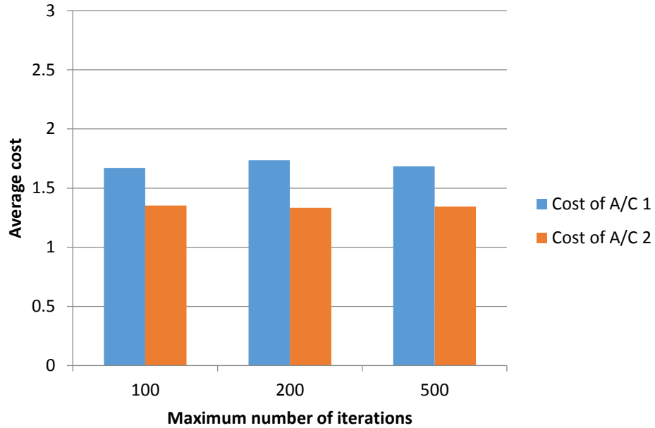
FIGURE 26: AVERAGE COSTS OF THE NEGOTIATED TRAJECTORIES FOR BOTH AIRCRAFT VERSUS THE MAXIMUM NUMBER OF ITERATIONS
