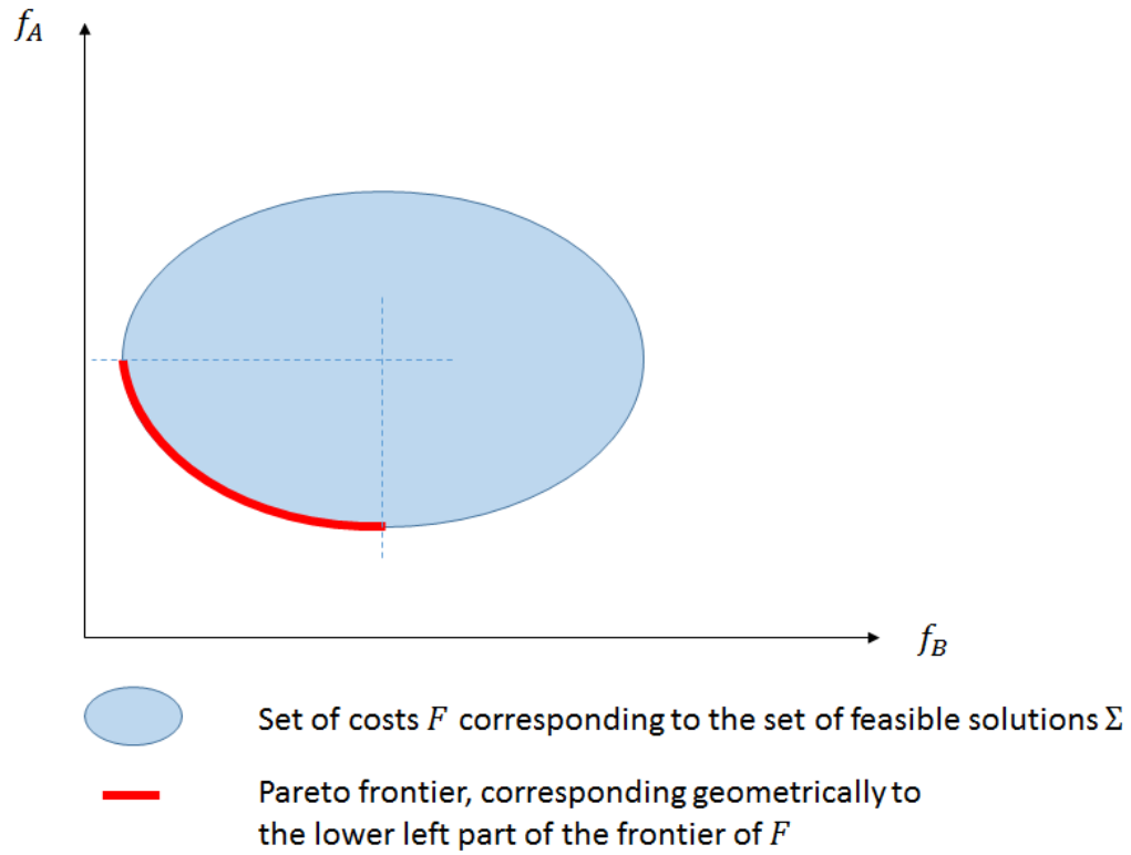
FIGURE 3: PARETO FRONTIER ILLUSTRATION
