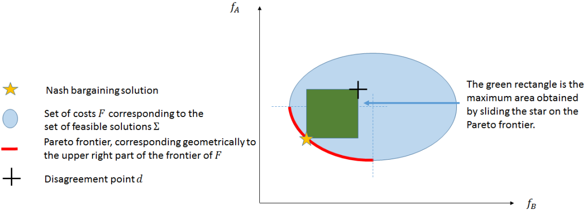
FIGURE 5: NASH BARGAINING SOLUTION
