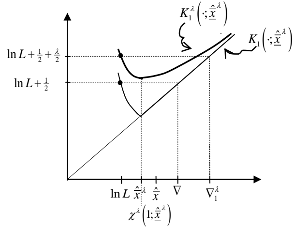
Figure 3.2 Mixed norm boundary solution at \hat{x}^\lambda = \ln L + \frac{\hat{x}^\lambda}{x}
