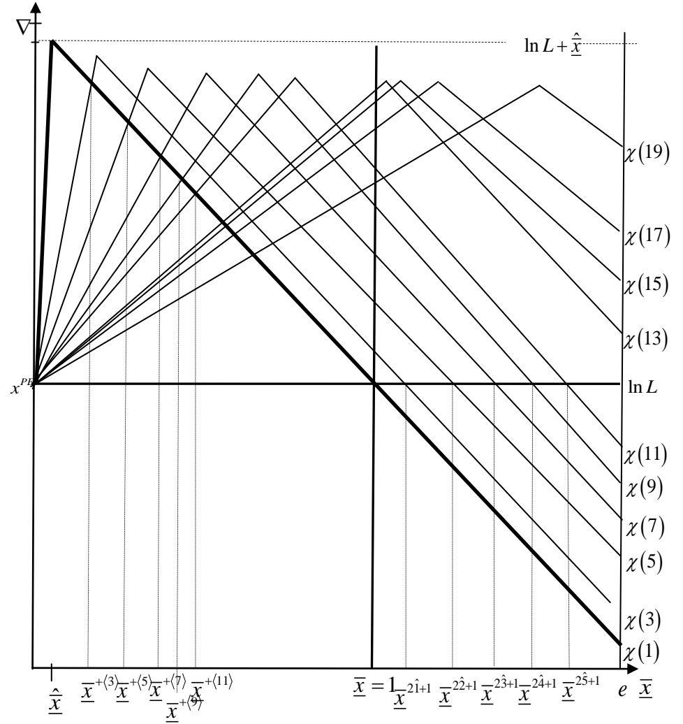
Figure 5.4 Equilibrium structure under uniform distributions, m \leq 9
