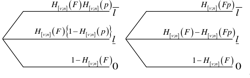
Figure 5.2 Transformed reduced norms from bifurcated trials (left node) and unitary trials (right node), L=2 , F=F(x_s) , p=p(x_l)
