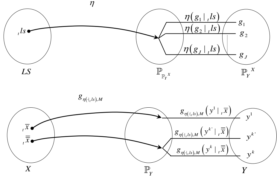
Figure 1.1 The process generating formally enforceable norms and judgments (node g_{\eta(\cdot|ls), M}(y^1 | {}_t \bar{x}) is degenerate)
