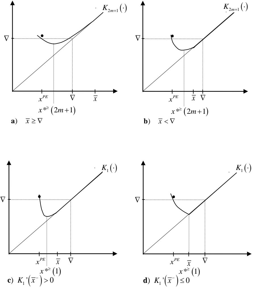
Figure 4.2 Overcomplying solution candidates ( K_{2m+1}'(x^{PE}) < 0 ). a) and b):
