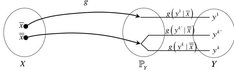
Figure 2.2 Global representation of g
