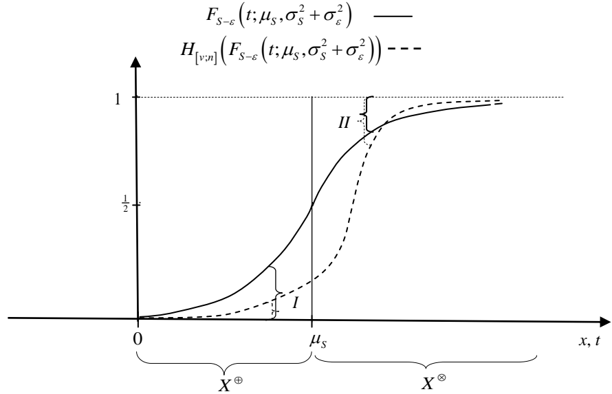
Figure 4.1 Type I and II error probabilities generated by M_1 and M_{[v,n]} (legal and epistemic uncertainty from normal distributions)
