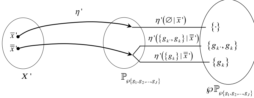
Figure 2.1 Global representation of power-conferring norms (node \eta'(\cdot | \bar{x}') degenerate)
