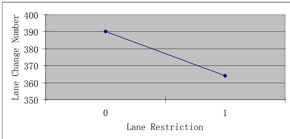
Figure 78 Restrictions to Truck Sensitivity on Lane Change Number within FA
