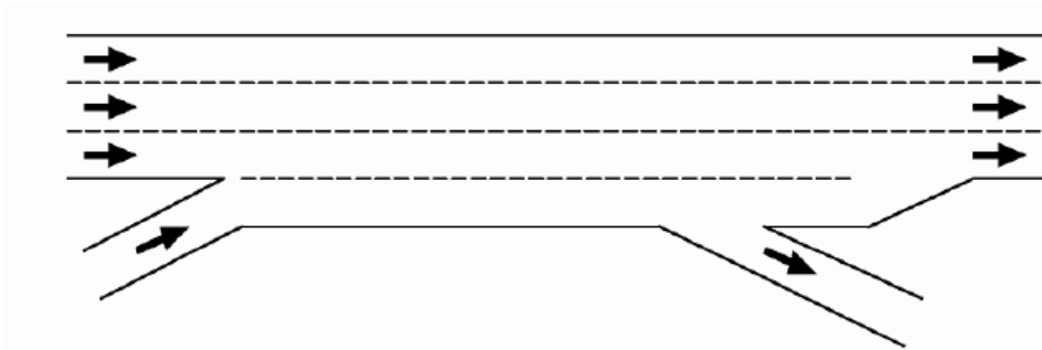
Figure 9 Auxiliary Lanes Terminated with Downstream Taper
