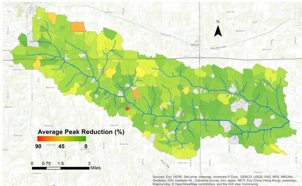
Figure 6.4: Headwaters North English River Peak Reduction with Full WASCOB Implementation. Average peak discharge reduction (in %) for each subbasin in Headwaters North English River between the baseline simulation and the complete WASCOB implementation scenario.
