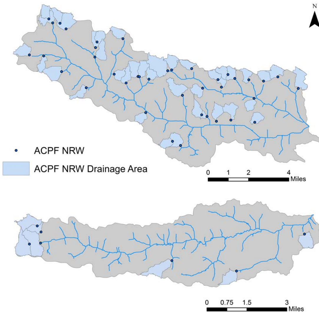
Figure 3.2: ACPF Sited Nutrient Removal Wetlands. ACPF Sited 39 nutrient removal wetlands in Headwaters North English River (top) and 7 in Gritter Creek (bottom).
