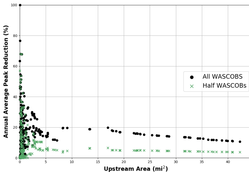
Figure 6.7: Headwaters North English River Peak Reduction with WASCORB Implementation. Average peak reduction in Headwaters North English River for each subbasin downstream of a WASCORB for the two simulations. The first is a full implementation of WASCORBs and the second is a random selection of half the WASCORBs.
