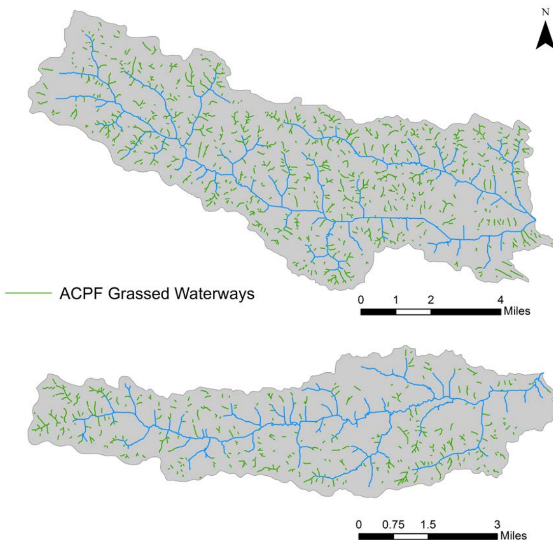
Figure 3.4: ACPF Sited Grassed Waterways. ACPF sited 99 miles of grassed waterways in Headwaters North English River (top) and 35 miles of grassed waterways in Gritter Creek (bottom).
