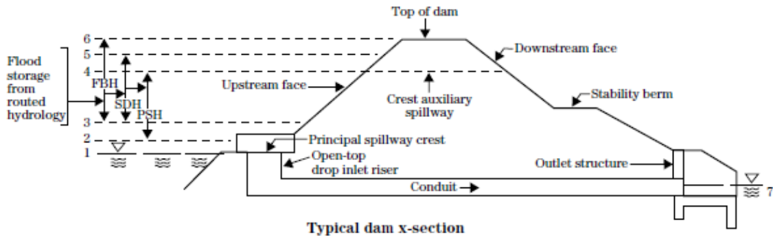
Figure 5.1: SITES Pond Diagram. Diagram of typical SITES pond ( National Resources Conservation Service, 2007b ).
