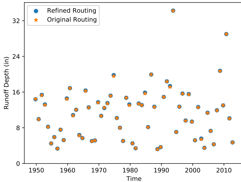
Figure 4.4: Annual Runoff Depth of Original and Refined Headwaters North English River Routing
