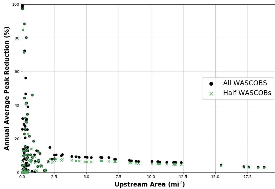
Figure 6.8: Gritter Creek Peak Reduction with WASCOS Implementation. Average peak reduction in Gritter Creek for each subbasin downstream of a WASCOS for the two simulations. The first is a full implementation of WASCOSs and the second is a random selection of half the WASCOSs.
