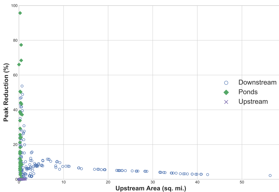
Figure 5.11: Headwaters North English River Peak Reduction with ACPF NRW. Average peak reduction for each subbasin in Headwaters North English River. The points are labeled by whether they are upstream of ponds, at the site of a pond, or downstream of ponds.
