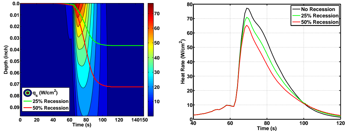
(a) Estimated heat rate map for varying surface (b) Surface heat rate profile for pre-defined recession profiles
