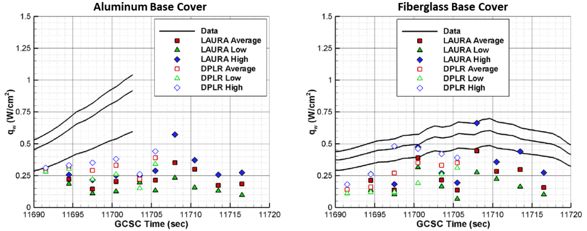
Figure 10: Computed Viking I aftbody heat flux compared to flight-derived values.
