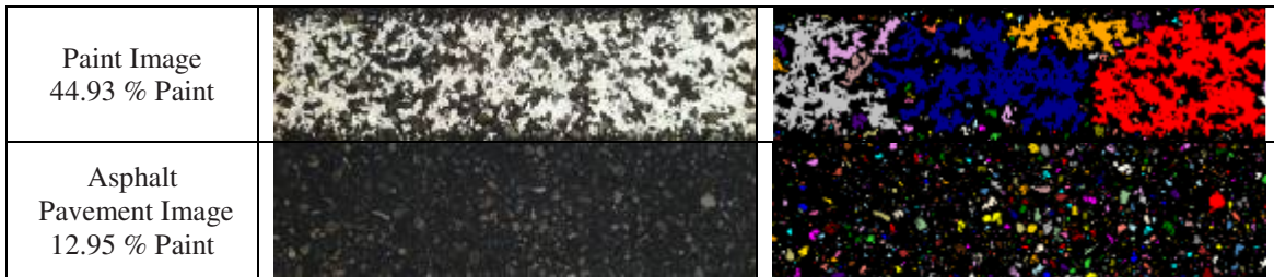
Figure 2.7: Asphalt pavement images used in test calibration procedure.
