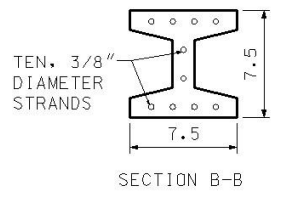
c) CROSS-SECTION DETAILS
