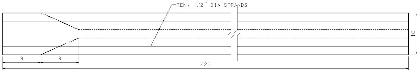
a) TOP VIEW
