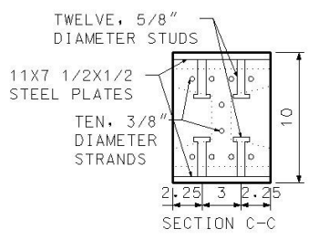
c) CROSS-SECTION DETAILS
