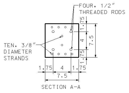
Figure 4.2. Dimensions and reinforcement details of the 8-ft (2.4-m) long UHPC pile units for laboratory tests
