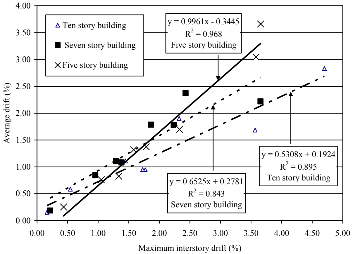
Figure 6.7. Correlation between the average and maximum interstory drifts obtained for the five, seven and ten story hybrid frame buildings based on the responses to long-duration ground motions
