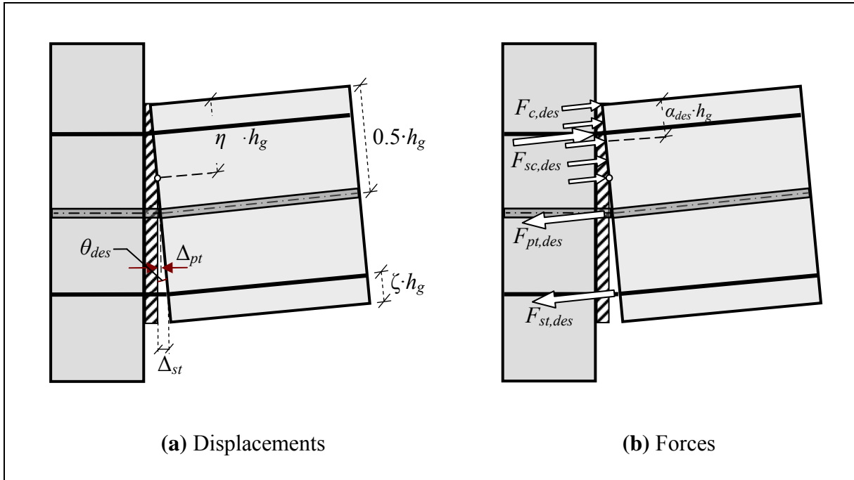
Figure 2.10. A hybrid frame system at the design limit state [2.13]
