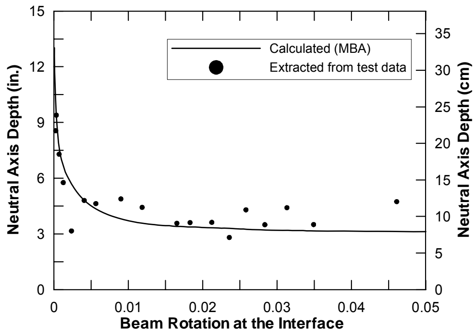
Figure 2.11. Comparison of the neutral axis depth as a function of the interface rotation for the PRESSS first floor hybrid connection test results and calculated values according to Monolithic Beam Analogy (MBA) method [2.10]
