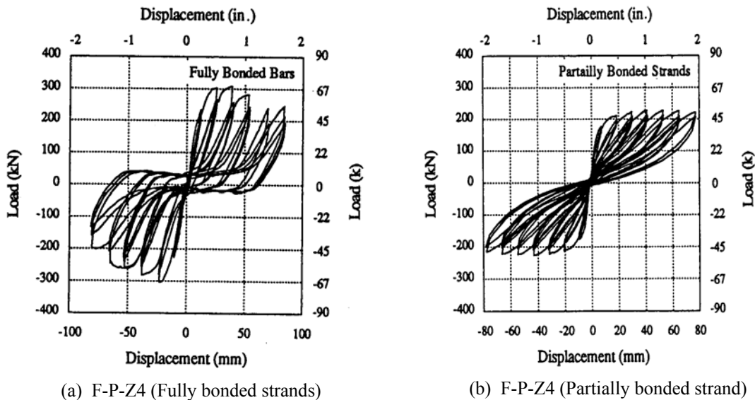
Figure 2.5. Lateral load-displacement behavior of precast frames with connections utilizing fully and partially bonded prestressing stands [2.4]
