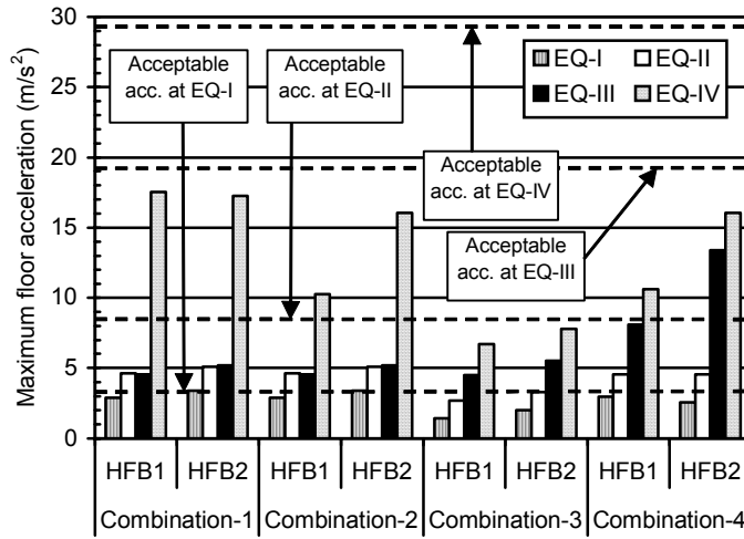
Figure 3.12. The maximum floor accelerations obtained for HFB1 (DBD) and HFB2 (FBD) when subjected to various combinations of short-duration ground motions summarized in Table 3.3
