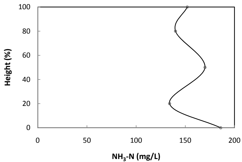
Figure 39. \text{NH}_3\text{-N} variation in the SGBR (sample 2).
