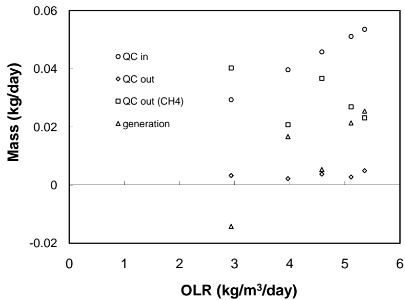
Figure 33. Mass balance in the SGBR (sample 1).
