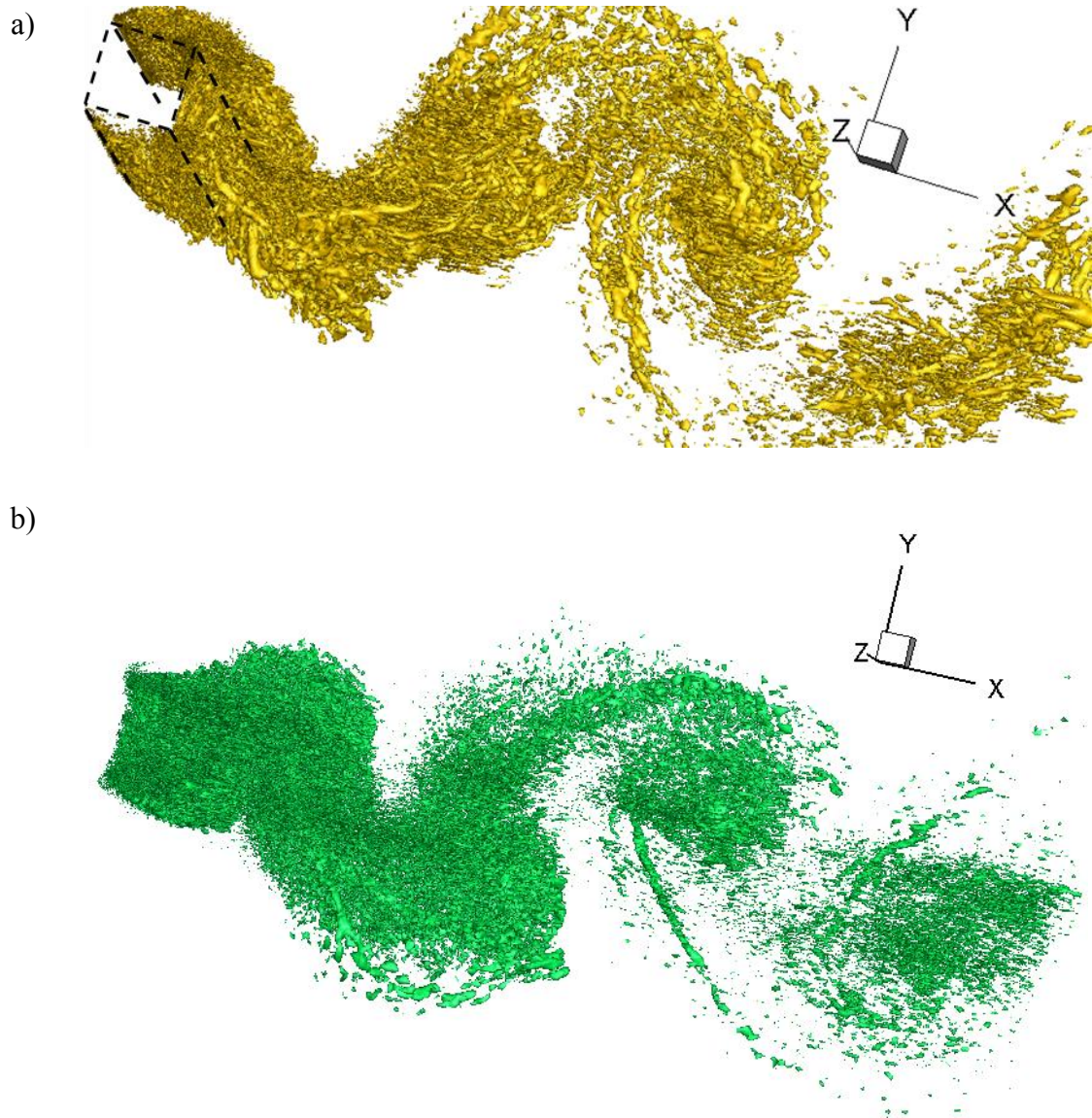
Figure 4.12 Visualization of 3D instantaneous vortical structures using the Q-criterion: a) square cylinder; b) vertical plate.
