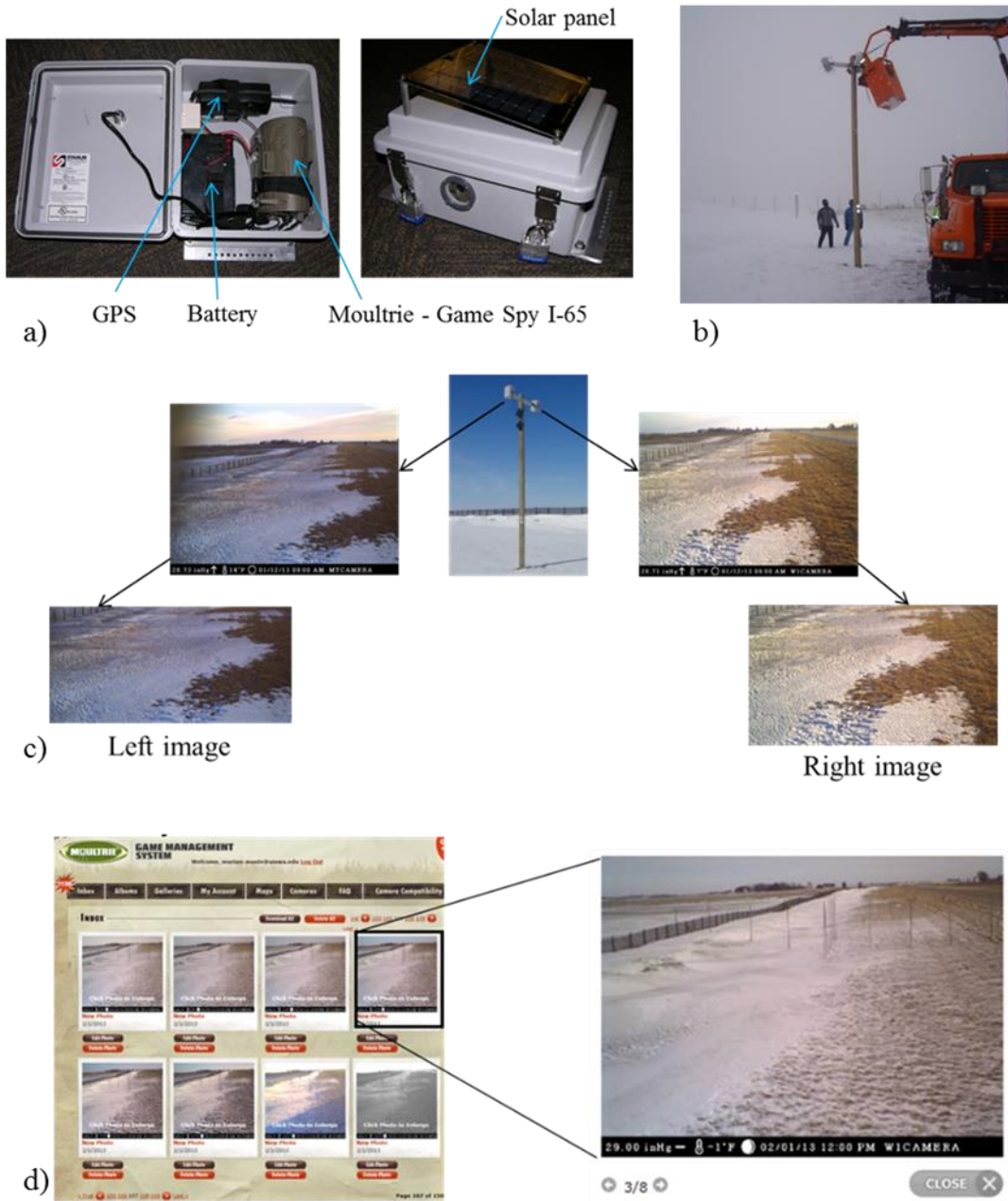
Figure 11.4 The image-based system used for site monitoring: a) the camera assembly; b) camera installation in the pole; c) raw images acquired for CRP processing; d) the real-time, web-based image-management platform.
