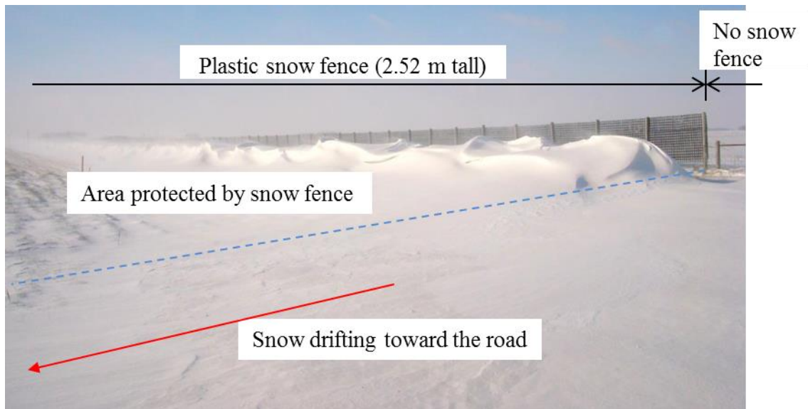
Figure 1.8 Picture illustrating the effect of placing a snow fence close to a road on snow drifting. The unfenced area on the right is subject to significant snow blowing and drifting toward and over the road, leading to the development of a significant snow deposit on the roadway. On the left side, which is protected by a structural snow fence, snow accumulates on the downwind side of the fence but the snow deposit close to the roadway is negligible. The picture was taken on a road near Williams, Iowa, U.S.
