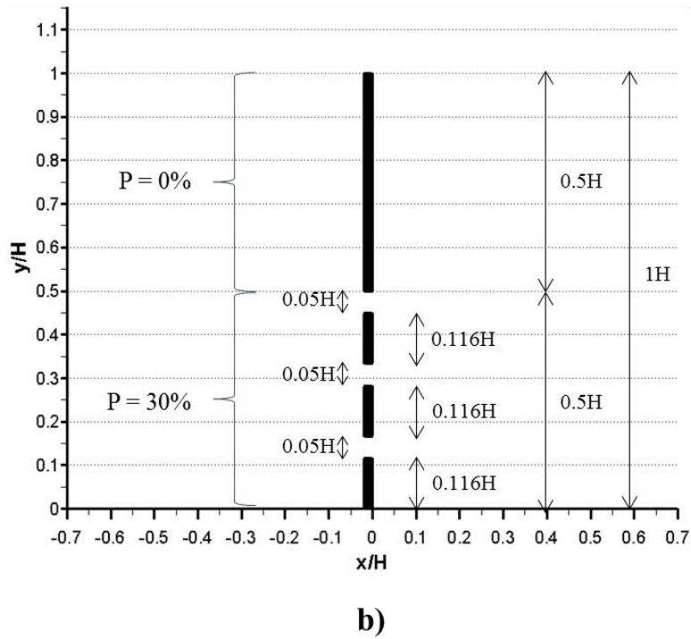
Figure 4.26 Computational domain (a) and main geometrical dimensions of the porous plate (b) used to simulate flow past a porous plate mounted on a flat bed.
