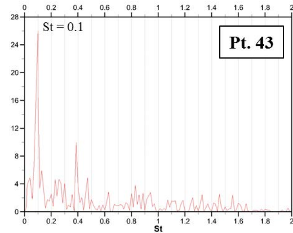
Figure 7.8 Power spectra of vertical velocity for G=0.2H case at: point 10 ( x=0.5H , y=1.3H ), point 28 ( x=18H , y=1.76H ) and point 43 ( x=22.5H , y=1.76H ). Location of points is shown in Figure 7.4c.
