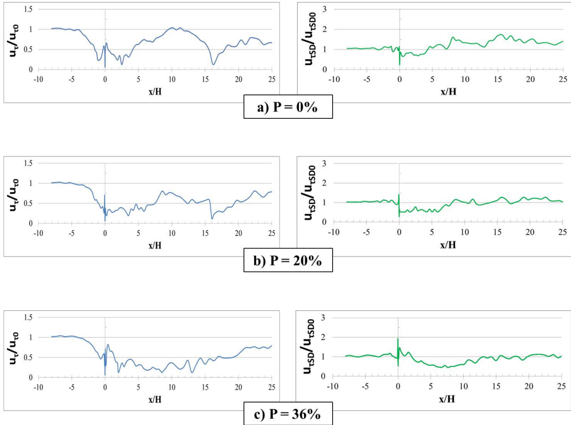
Figure 5.22 Nondimensional spanwise-averaged mean bed friction velocity, u_\tau/u_{\tau 0} , where u_{\tau 0}=0.04U_0 is the mean bed shear stress in the incoming fully developed turbulent channel flow. Also shown is the nondimensional spanwise-averaged rms of the bed friction velocity fluctuations where u_{\tau SD0}=0.025U_0 is the mean rms of the bed shear stress in the incoming fully developed turbulent channel flow.
