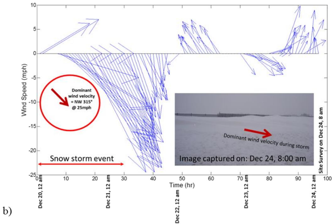
Figure 11.3 Wind characteristics for the observation site during the December 20-24, 2012 snowstorm: a) comparison of areal wind velocity with local data; b) wind variation at one of the stations for the duration of the storm.
