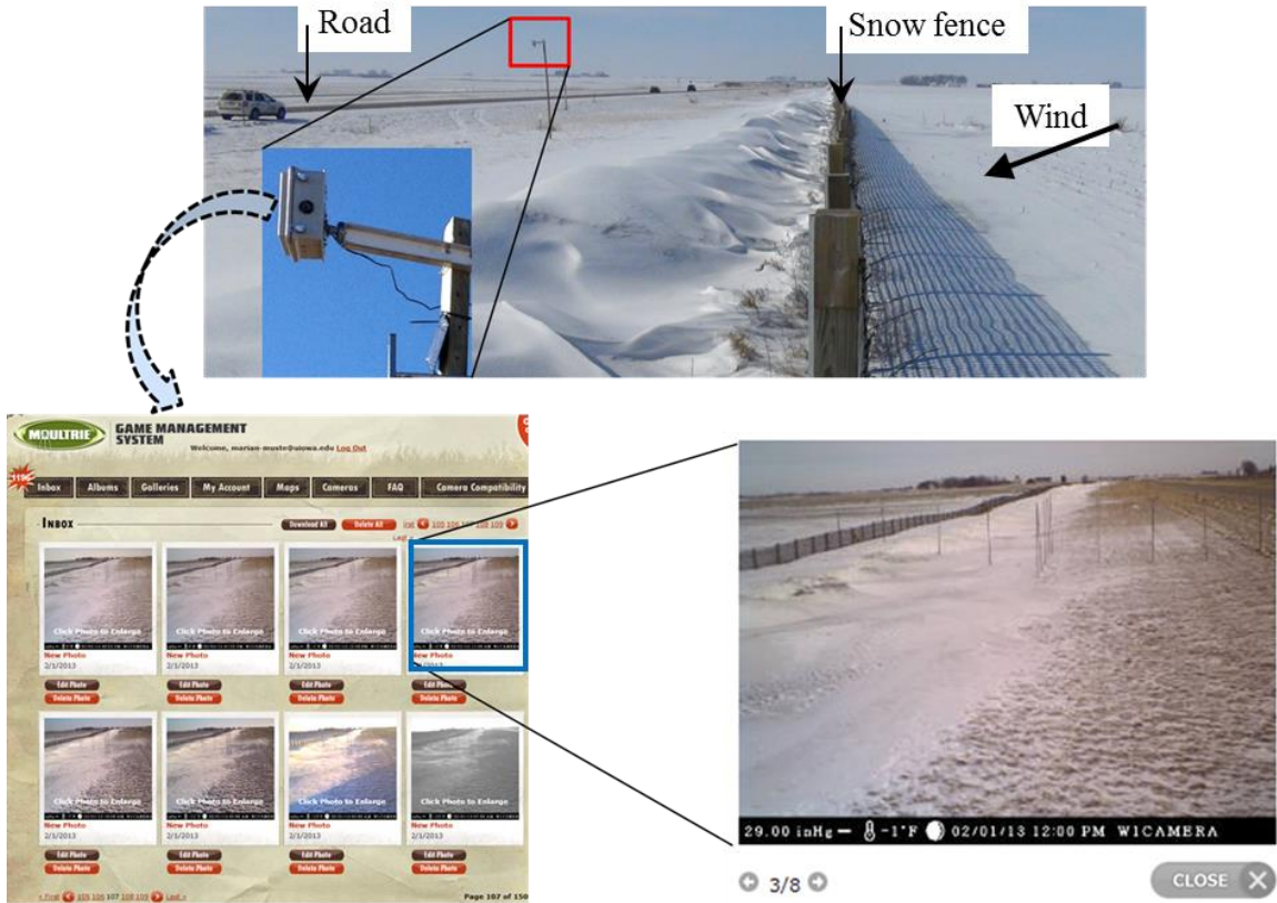
Figure 10.4 Field set-up and information provided by the real-time monitoring system.
