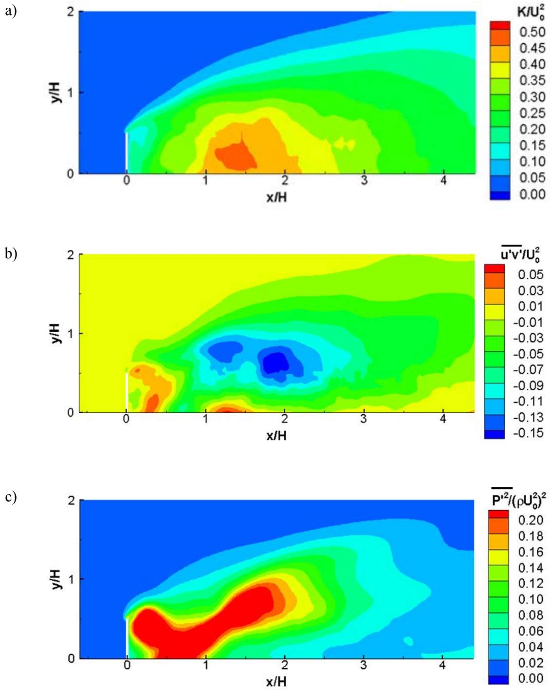
Figure 4.25 Nondimensional turbulence statistics for flow past a vertical plate: a) turbulent kinetic energy; b) primary Reynolds shear stress; c) mean pressure fluctuations.
