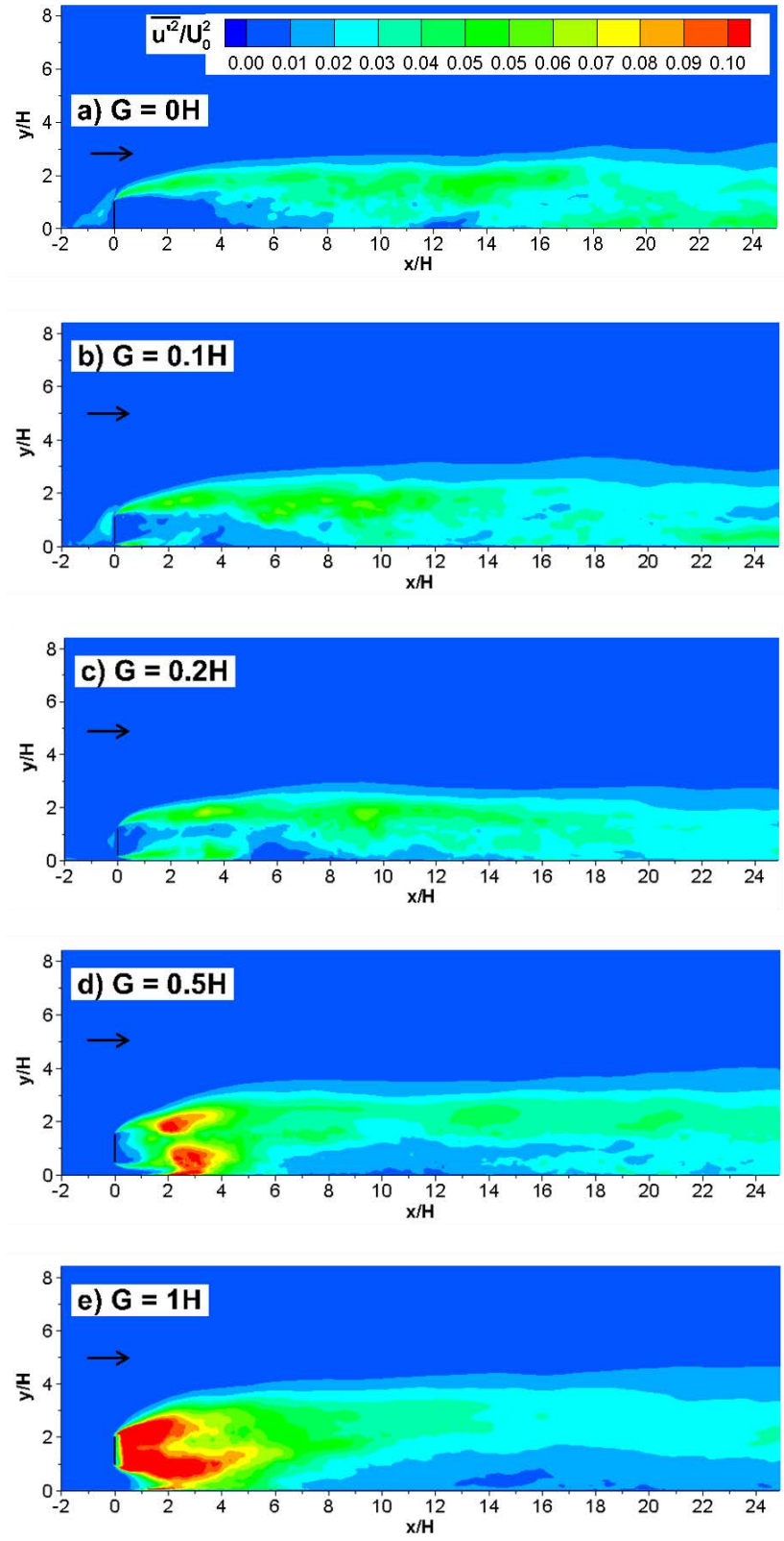
Figure 6.19 Mean streamwise velocity fluctuations, \overline{u'^2}/U_0^2 , in an x-y plane.
