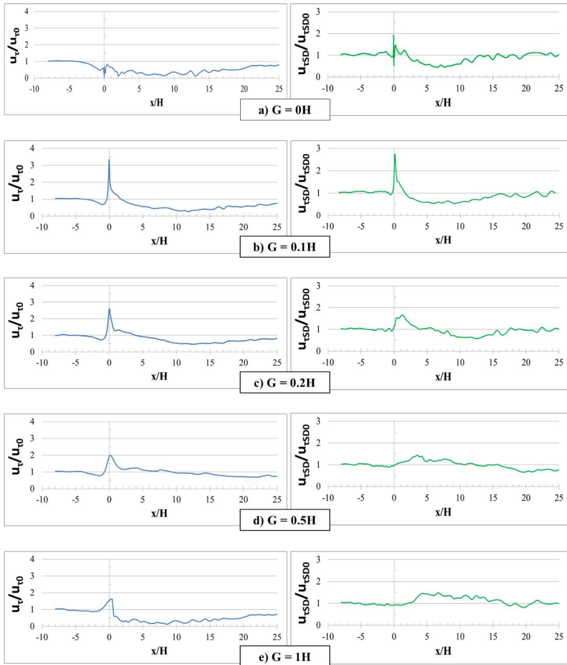
Figure 7.19 Nondimensional spanwise-averaged mean bed friction velocity, u_\tau / u_{\tau 0} , where u_{\tau 0} = 0.04U_0 is the mean bed shear stress in the incoming fully developed turbulent channel flow. Also shown is the nondimensional spanwise-averaged rms of the bed friction velocity fluctuations where u_{\tau SD 0} = 0.025U_0 is the mean rms of the bed shear stress in the incoming fully developed turbulent channel flow.
