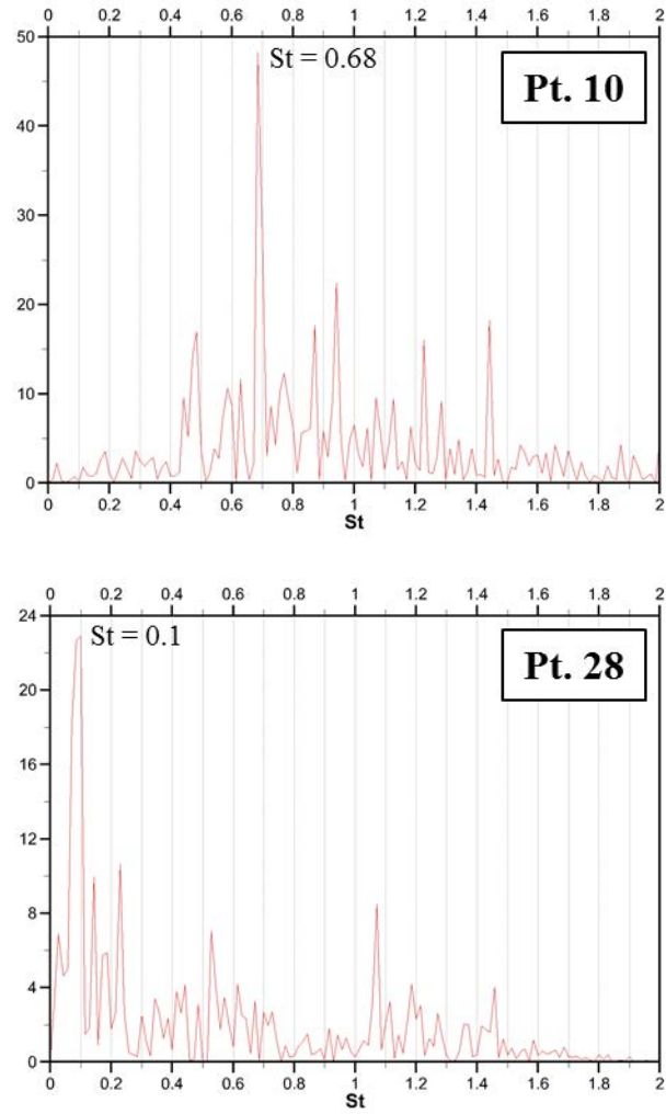
Figure 9.9 Power spectra of vertical velocity for the P=36% rough-bed case at: point 10 ( x=0.5H , y=1.3H ) and point 28 ( x=18H , y=1.76H ). Location of points is shown in Figure 9.5d.
