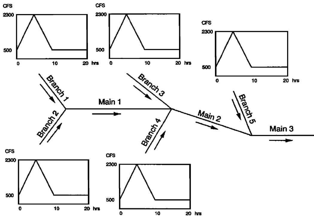
Figure 3.11. Eight-branch river network test case with five triangular inflow hydrographs
