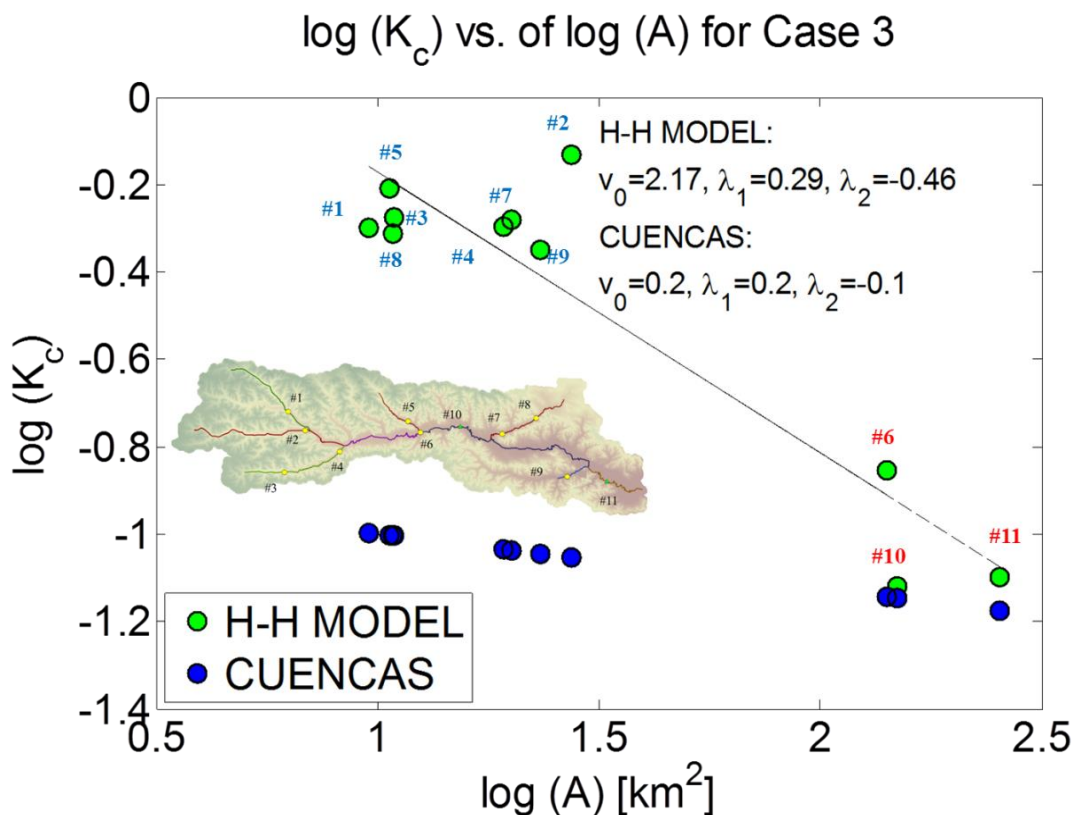
Figure 4.27. Log-log plot of K_c versus upstream drainage area, A from H-H model and CUENCAS for 11 gauging station in Clear Creek Watershed for case #3
