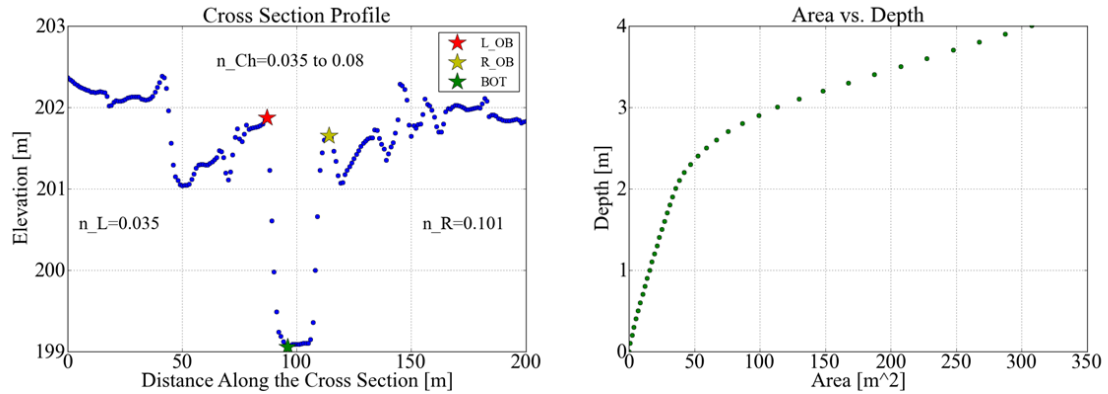
Figure 3.9. Computation of area (A) as a function of storage level based on the cross section profile
