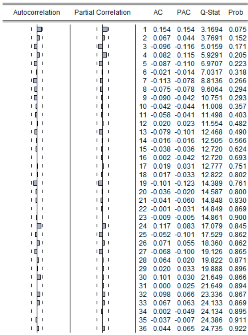
Figure B.1 Correlogram of residuals for log transformed spam rate model
