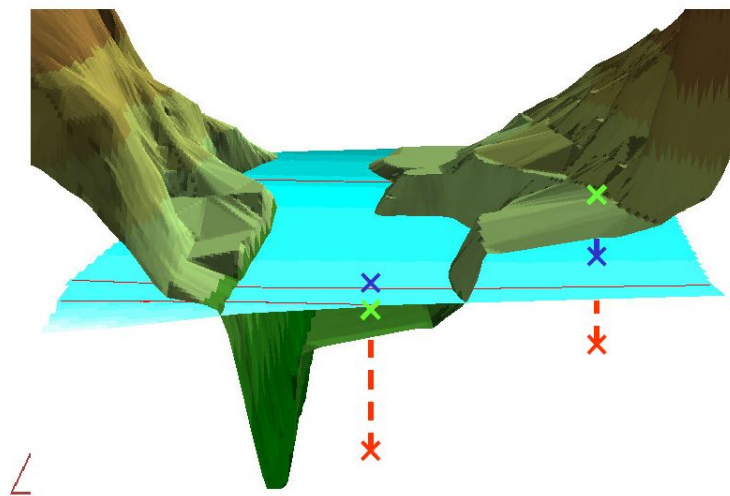
Figure 4.4: Determination of flood depth grid (FEMA, 2012)
