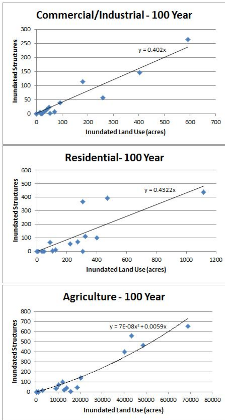
Figure B.3: Regressions for data reconstruction – 100 year event
