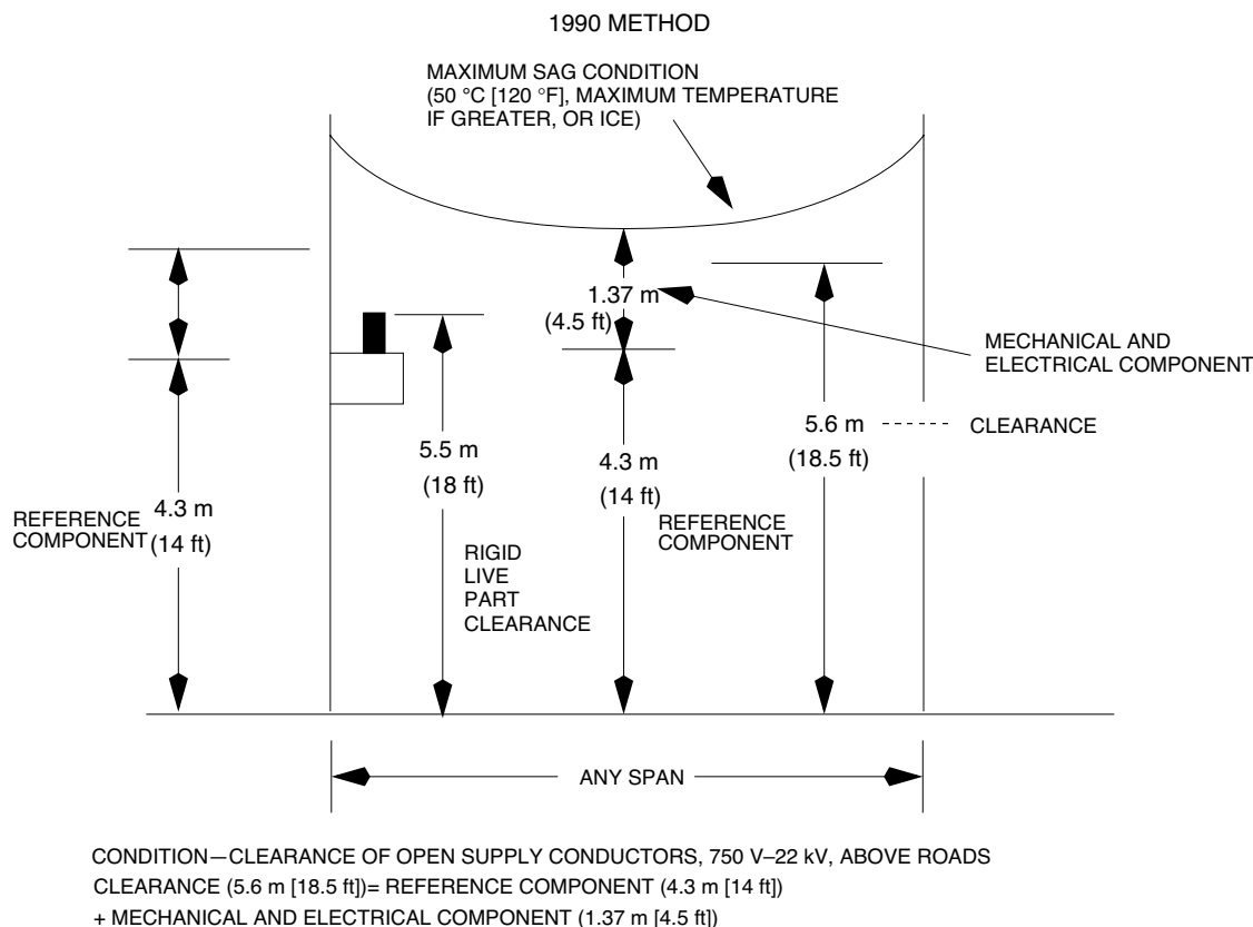
Fig A-1 Clearance at Maximum Sag
