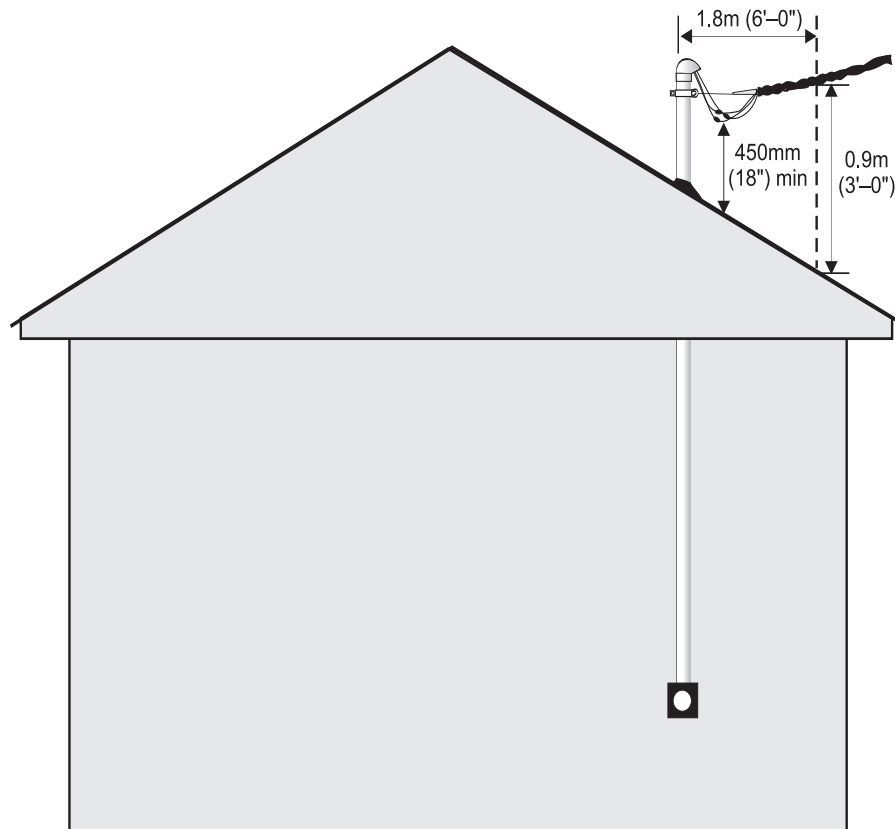
Elevation View
