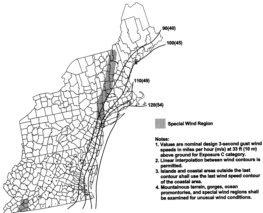
Fig 250-2(e) Mid and Northern Atlantic Hurricane Coastline*
