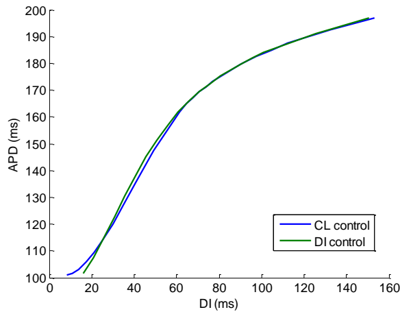
Figure 11, continued. Restitution curves computed using DI control and CL control when (A) no electro-physiological alterations were performed and (B) when I_{kr} was decreased by 62%. Notice that (A) shows minimal difference between restitution curves computed from DI and CL control, while (B) shows that APD was higher (as much as 4 ms) during DI control than during CL control for DIs between 30 ms and 60 ms when I_{kr} was decreased by 62%.
