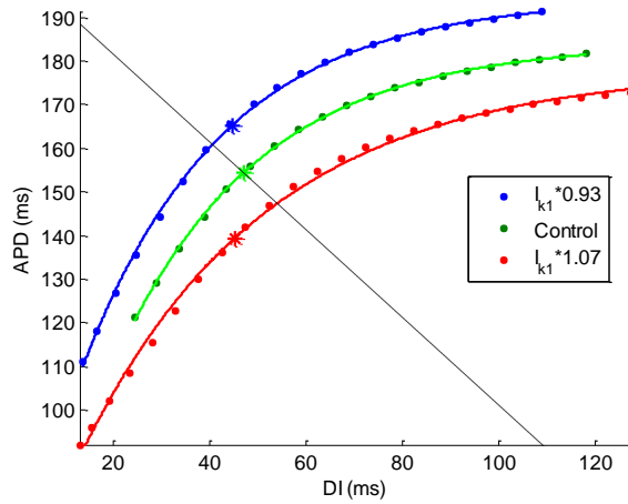
Figure 19, continued. Altering I_{k1} by \pm 7\% for (A) the SGA, (B) dynamic restitution, and (C) standard restitution.
