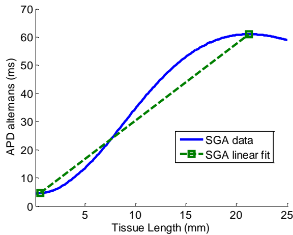
Figure 6, continued. Development of the SGA. (A) Simulated transmembrane potentials (TMPs) of the pacing site, where DI is held constant, and a site in the middle of the tissue where DI is not constant. (B) A space-time plot of simulated TMPs for the last four beats of the protocol. More positive TMPs are in lighter color and more negative TMPs are in darker color - see color key. (C) The spatial distribution of APD for the last two beats. (D) The absolute difference of APD alternans for the last two beats at each cell. The index used to predict stability for the SGA method is the slope of the linear fit.
