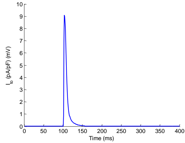
Figure 3, continued. The (A) simulated action potential and underlying ionic currents: (B) I_{kr} , (C) I_{k1} , (D) I_{to} , (E) I_{CaL} , and (F) I_{NaCa} , which among other ionic currents sum to produce the simulated action potential.
