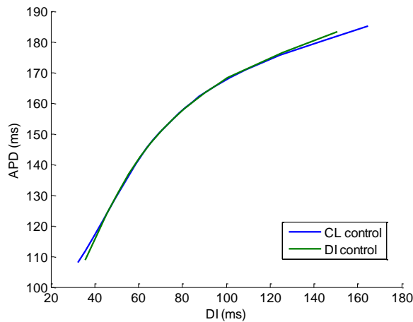
Figure 11, Restitution curves computed using DI control and CL control when (A) no electro-physiological alterations were performed and (B) when I_{kr} was decreased by 62%. Notice that (A) shows minimal difference between restitution curves computed from DI and CL control, while (B) shows that APD was higher (as much as 4 ms) during DI control than during CL control for DIs between 30 ms and 60 ms when I_{kr} was decreased by 62%.
