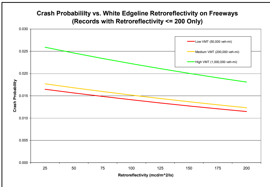
Figure 31: Crash Probability vs. WEL Retroreflectivity on Freeways (Records with Retroreflectivity ≤ 200)
