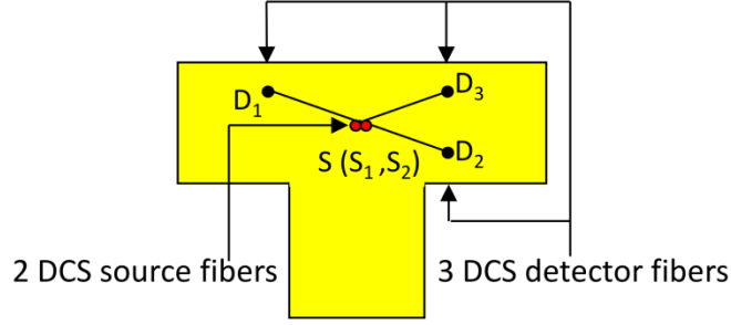
Figure 6.1: A fiber-optic probe consisting of two source fibers ( S_1 = 785 nm and S_2 = 853 nm) and three detector fibers ( D_1 to D_3 ). Multi-mode fiber (1mm) locates in D_1 , single-mode fiber (SM600) locates in D_2 , and few-mode fiber (SM980) locates in D_3 . The separations between the sources and detector fibers are equal (i.e., SD_1 = SD_2 = SD_3 = 2.5 cm). The separations between detector fibers are D_1D_2 = 4.6 cm, D_1D_3 = 4.3 cm and D_2D_3 = 0.8 cm, respectively.
