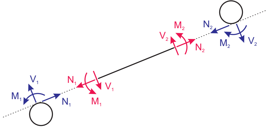
Figure 70: Non-central forces applied to circular nodes of a chiral structure
