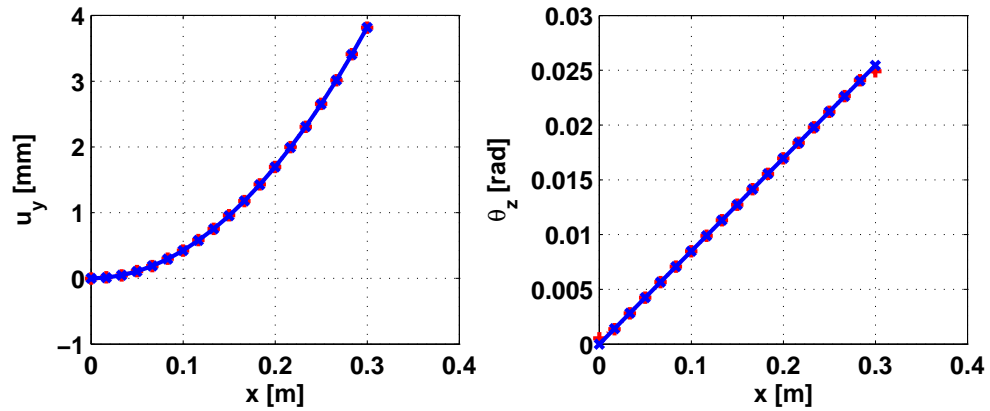
Figure 91: Deflection and angle of the reference line (chiral +, beam \times ), when subjected to a unit tip moment, for the case N_h = 4
