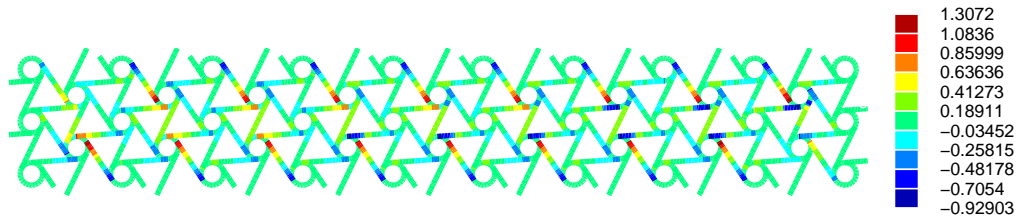
Figure 84: Direct axial strain (in \mu -strain) due to unit tip moment
