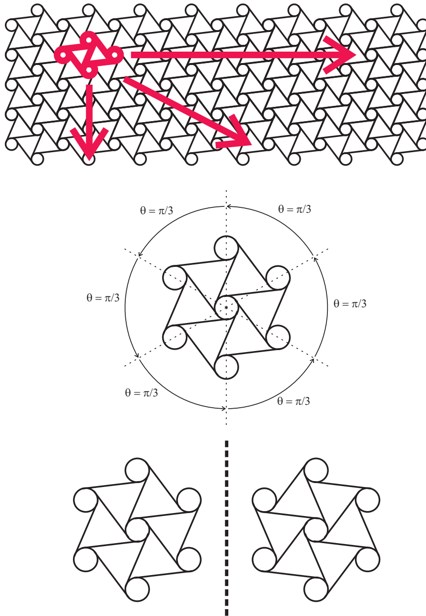
Figure 69: Three fundamental aspects of hexagonal chiral structures: periodicity, invariance through a 60^\circ rotation, and chirality
