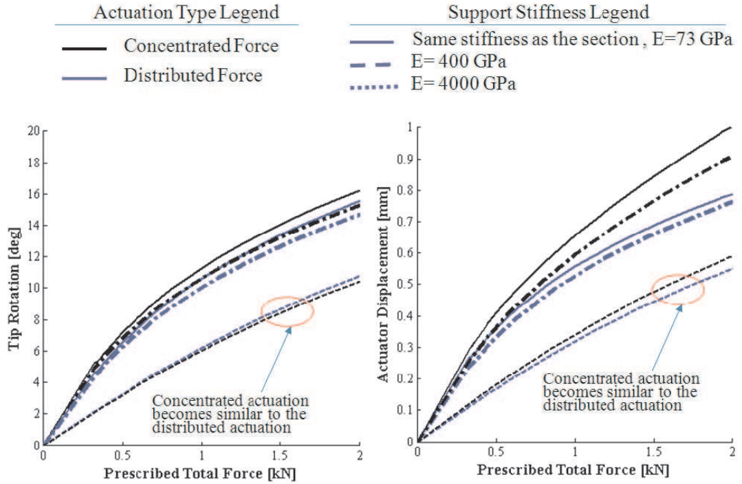
Figure 29: Concentrated and distributed actuation for different values of the support stiffness
