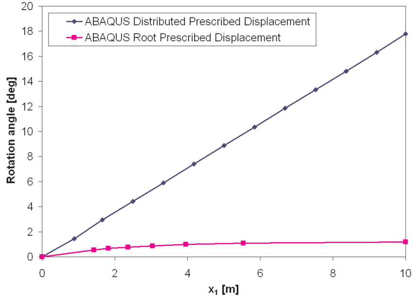
Figure 53: Spanwise variations of the rotation angle in different cases of prescribed axial displacements
