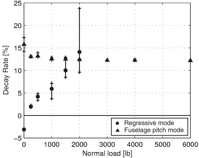
Figure 6: Decay rate for several normal force levels, for a helicopter in ground resonance with a rotor speed of 150 RPM
