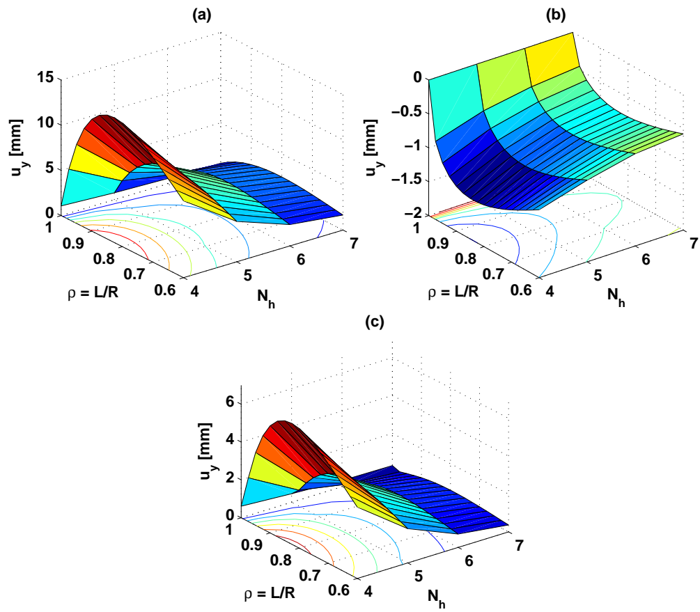
Figure 108: Tip deflection under estimated aerodynamic loads with varying number of cells and varying \rho , in the case t = 1 mm and t_p = 0.5 mm: (a) passively loaded structure; (b) double bending actuation only; (c) airloads and actuation
