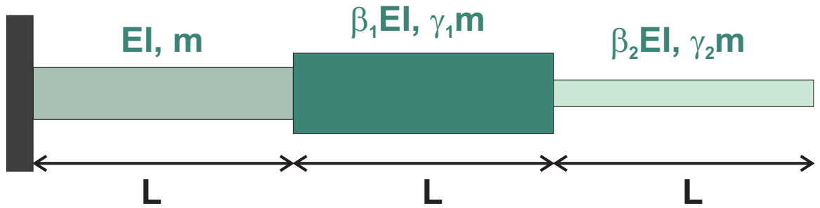
Figure 141: Regular beam with three different sections of constant properties
