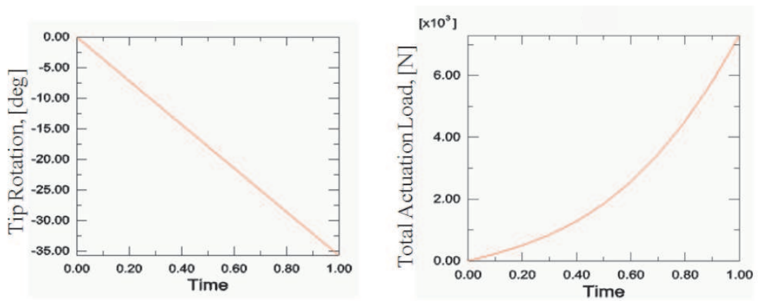
Figure 39: Tip rotation and total actuation load under prescribed warping displacement
