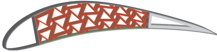
Figure 66: Deformable airfoil with chiral core
