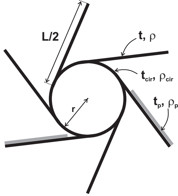
Figure 132: Geometry of an inertia element
