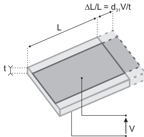
Figure 75: Two actuator designs using piezoelectric materials: linear piezo-stack and laminar piezo-bender
