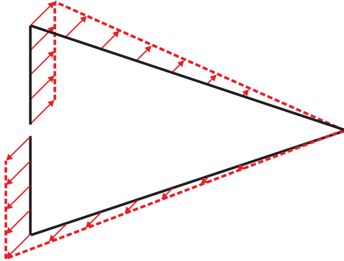
Figure 154: Modified warping function for open triangular section with constrained center of rotation
