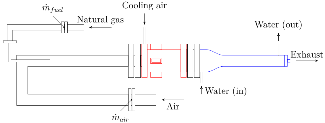
Figure 3.1: A schematic of the high pressure testing facility where Configuration A is operated is shown. The pressure vessel is outlined in red , while the water-cooled exhaust section is outlined in blue . The locations of the orifice flow meters used to measure the mass flow rates of the preheated air and natural gas fuel are indicated.
