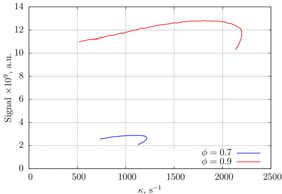
Figure 4.19: The plot shows the calculated CH LIF signal from a strained, laminar, methane-air flame at atmospheric pressure. The signal is calculated from Chemkin simulations using the Opposed flow flame reactor model.
