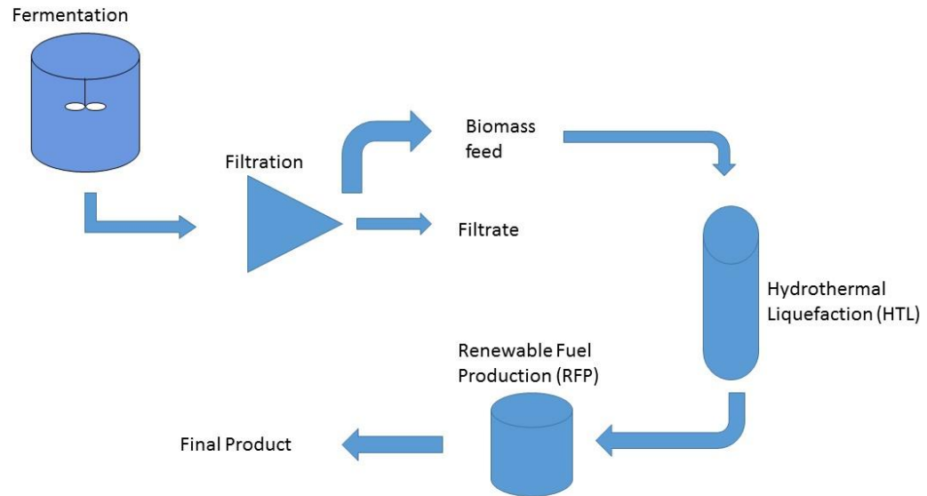
Figure 1: Generalized process flow diagram
