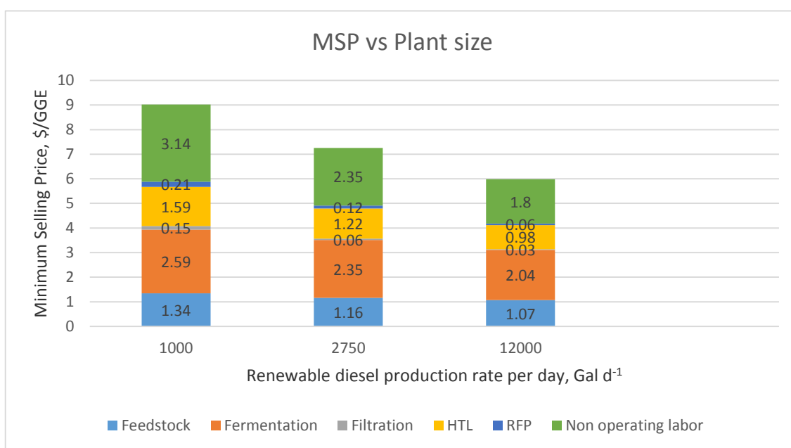
Figure 5: Cost contribution of various components for MSP for different production scales in practical scenario
