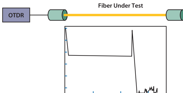
Acceptance testing without the use of launch and receive cables
