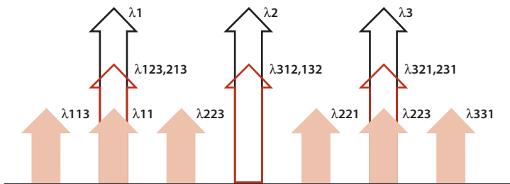
Four wave mixing of a signal on a fiber
