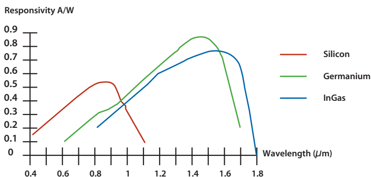
Responsivity of the three typical detector types
