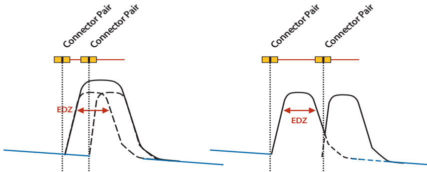
Two reflective events are closer than the EDZ. The OTDR is not able to separate the two events.
