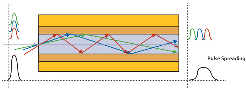
Modal dispersion in step-index multimode fiber
