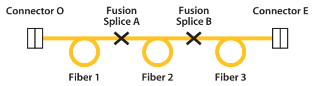
The span architecture
