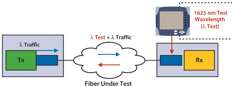
In-service testing at 1625 nm using the contra-propagation method
