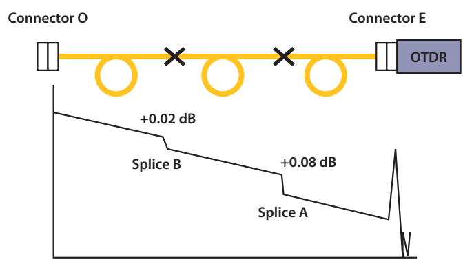
OTDR measurement from connector E to connector O (E -> O)
