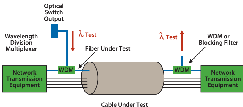
In-service monitoring of a link
