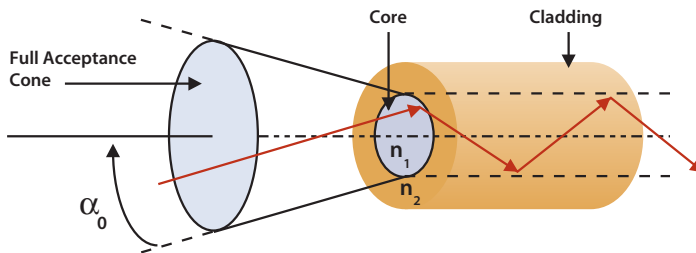
The injection of light into a fiber
