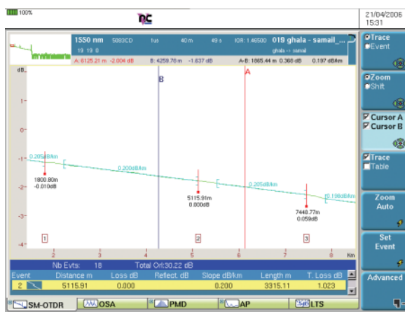
Semi-automatic measurement of a 0 dB splice loss
