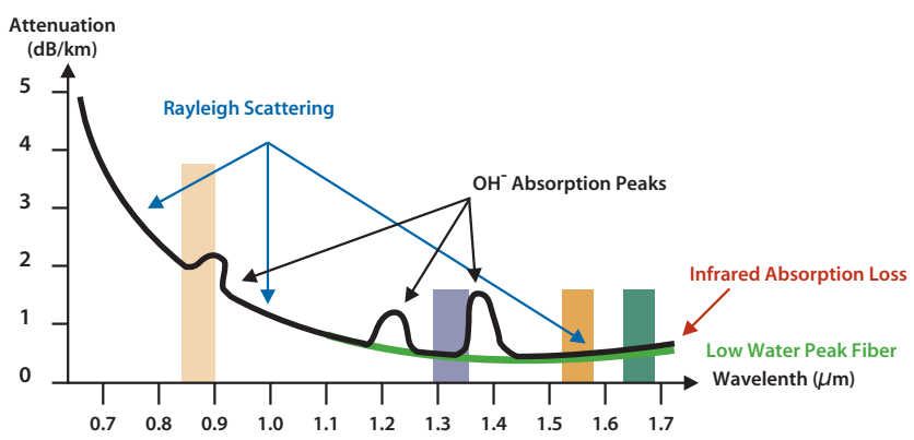
Fiber attenuation as a function of wavelength
