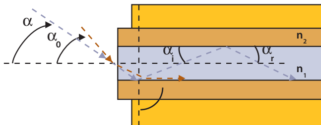
Reflection of light
