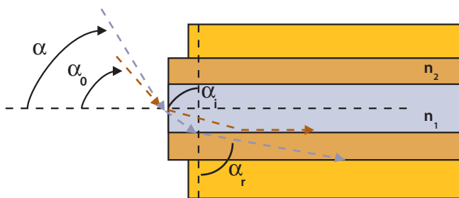
Refraction of light
