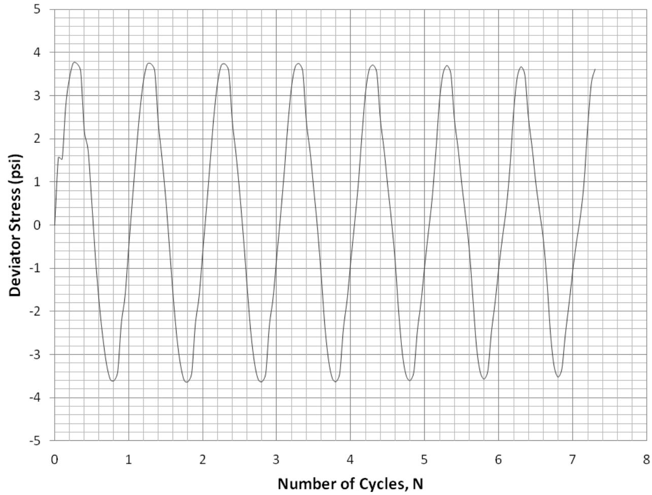
Figure A.57: Specimen F95C5 CSR 0.30 Deviator Stress Versus Number of Cycles Graph
