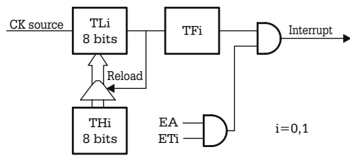
Fig. 6.4. The 8051 timer operating in mode 2
