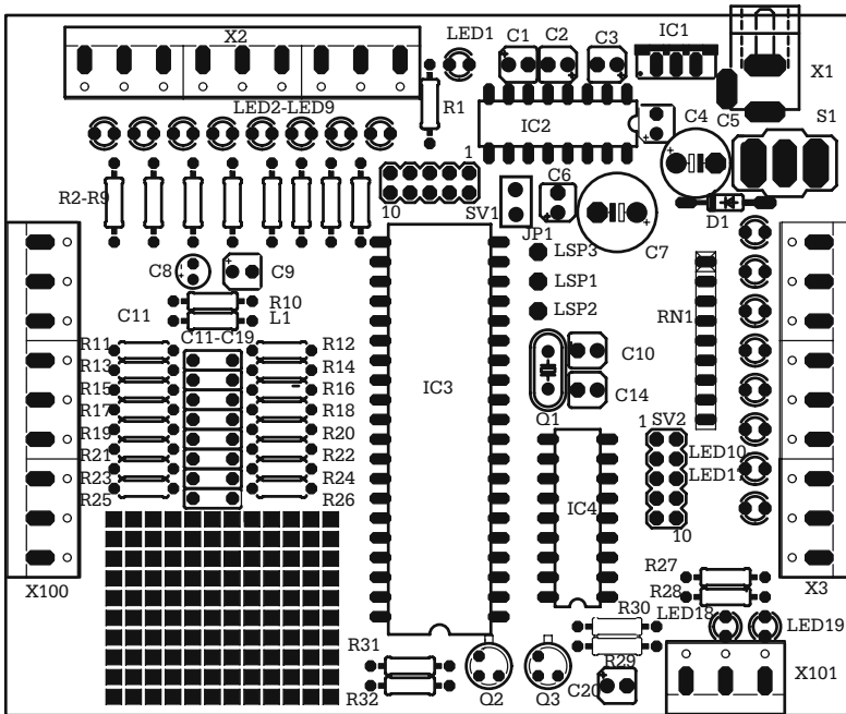
Fig. 10.2. PCB layout of the AVR development board
