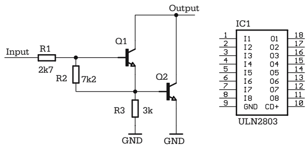
Fig. 2.5. ULN 2803 typical Darlington transistor interface for output lines
