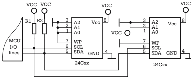
Fig. 5.4. Connecting I2C memory devices to a microcontroller
