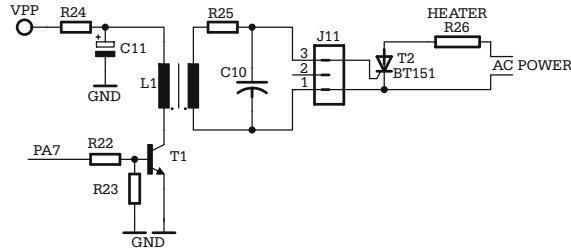
Fig. 14.12. The gate control circuit of the triac
