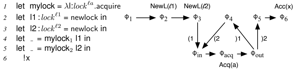
(a) Source program
