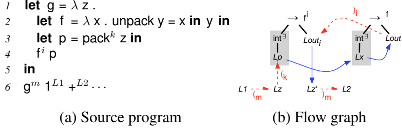
Figure 4.11: Example with Mismatched Flow
