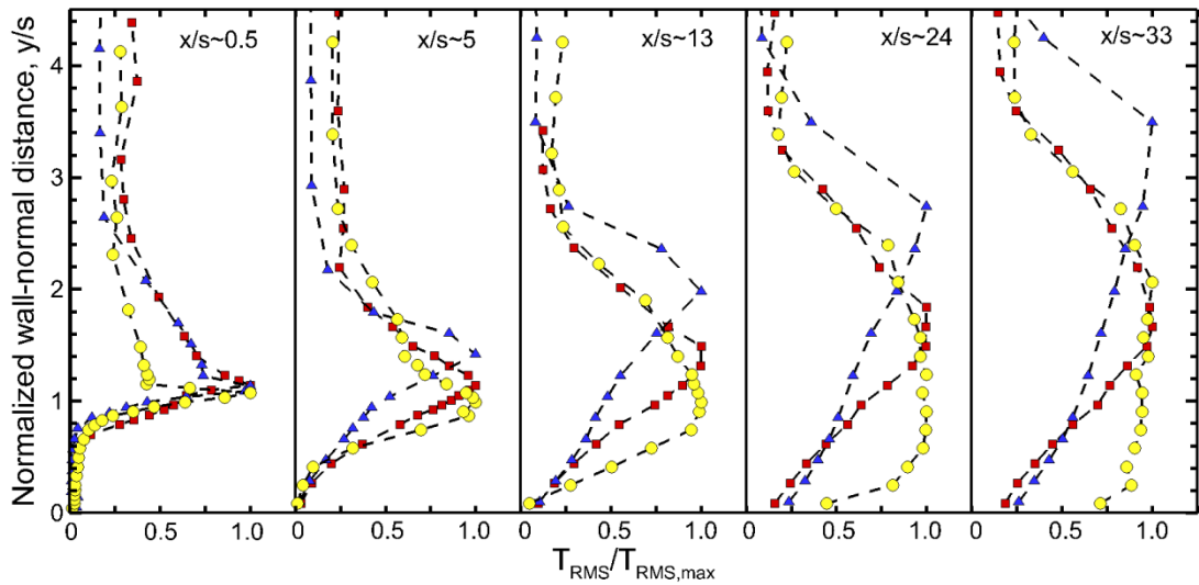
Figure 53. Normalized T_{RMS} profiles for the non-adiabatic flowfield (NA profiles exhibit similar behavior). ● wall-wake, ■ min-shear, ▲ wall-jet
