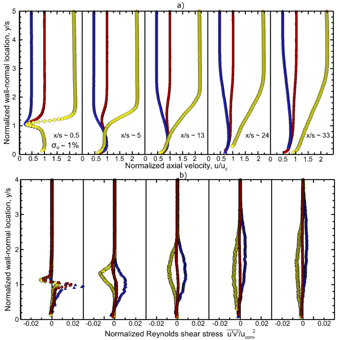
Figure 40. a) Mean axial velocity profile development, b) Reynolds shear stress profile development. \bullet wall-wake, \blacksquare min-shear, \blacktriangle wall-jet (adiabatic cases).
