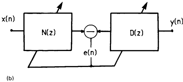
FIG. 4.12 Simplified gradient IIR adaptive filters: (a) Parallel type (output error); (b) series-parallel type (equation error).
