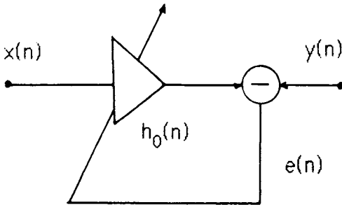
FIG. 6.1 Adaptive filter with a single coefficient.
