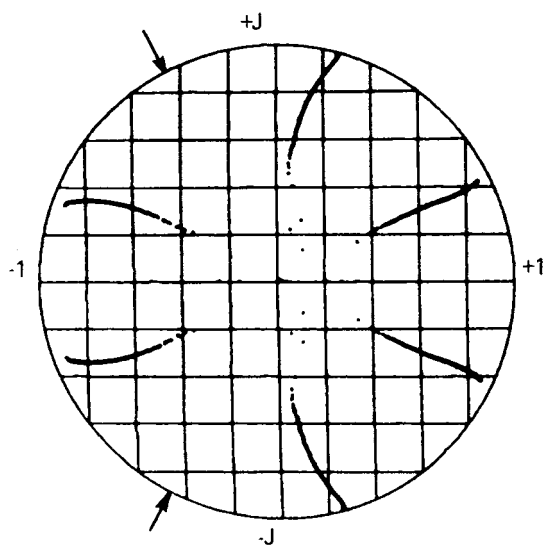
FIG. 5.10 Pole trajectories of a gradient adaptive IIR predictor applied to a sinusoid at frequency 2\pi/3 .
