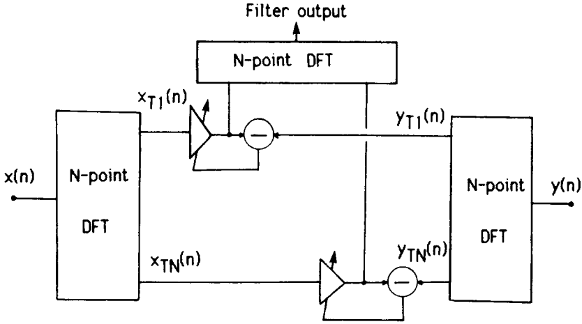
FIG. 7.14 FDAF structure.
