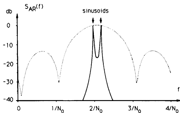
FIG. 10.4 AR spectral estimation of two sinusoids.
