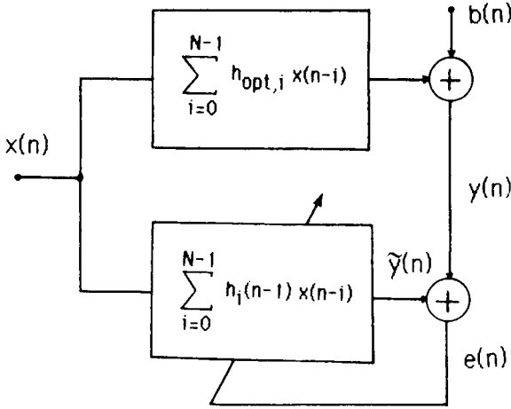
FIG. 6.8 Adaptive system identification.
