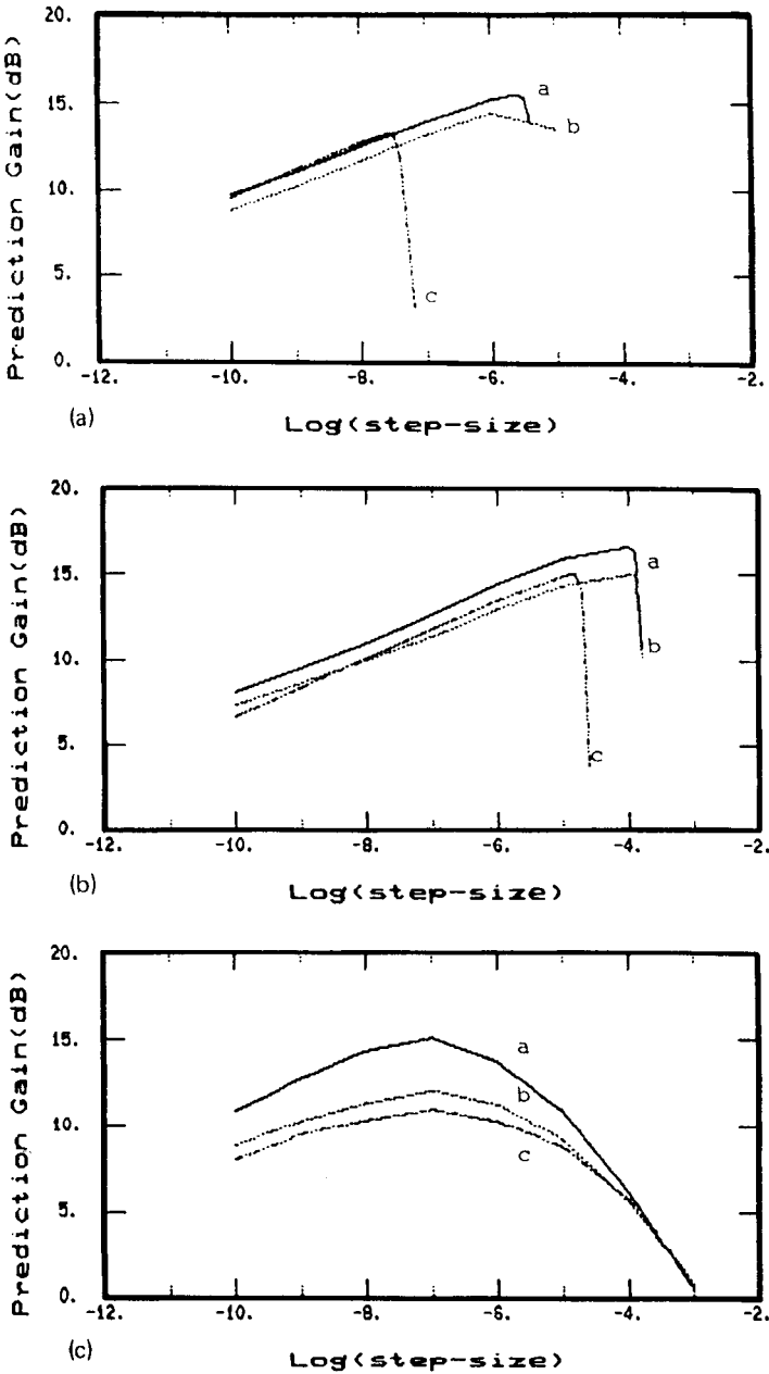
FIG. 4.8 Prediction gain vs. adaptation step size for three speech signals: (a) LMS with fixed step; (b) normalized LMS; (c) sign algorithm.
