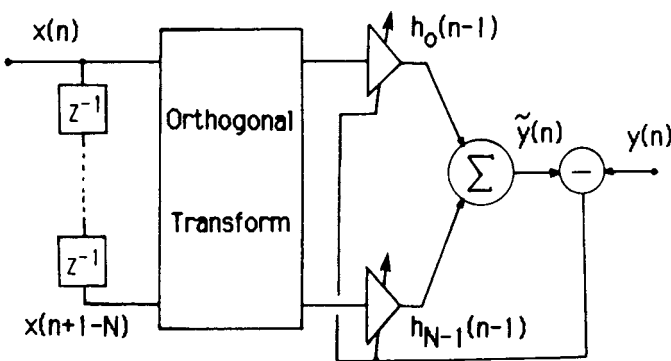
FIG. 7.15 FDAF with a single orthogonal transform.
