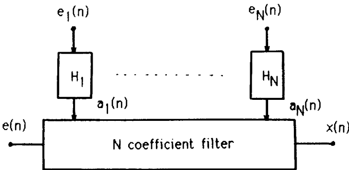
FIG. 2.11 Generation of a nonstationary signal.
