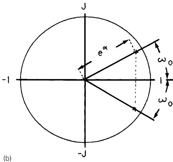
FIG. 2.1 (a) Waveform of a damped sinusoid. (b) Poles of the z -transform of the damped sinusoid.
