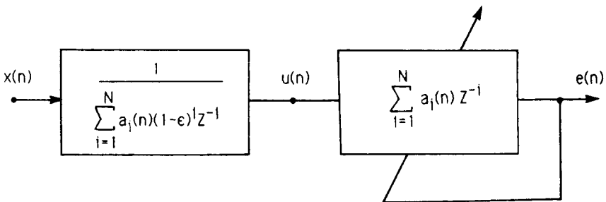
FIG. 10.5 FLS adaptive notch filter.
