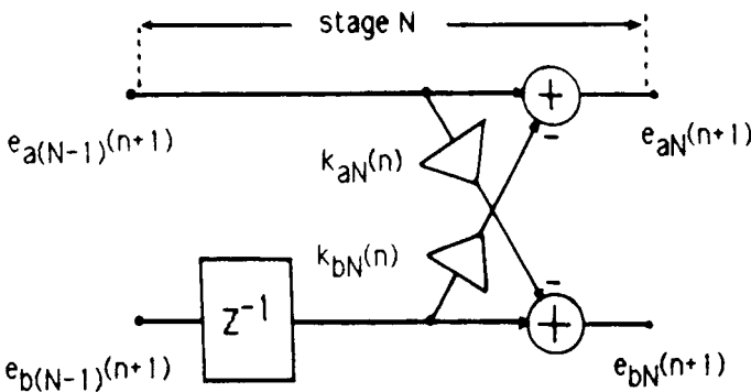
FIG. 8.1 Adaptive lattice prediction error filter section.
