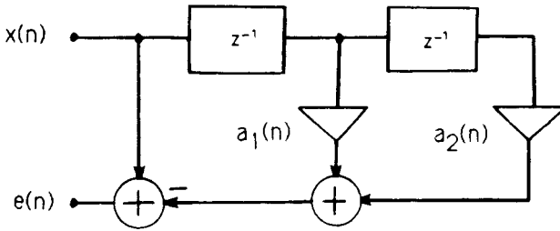
FIG. 4.3 Second-order prediction filter.
