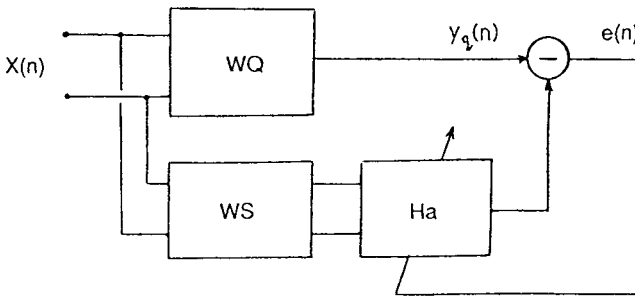
FIG. 4.10 Constrained adaptive filter.
