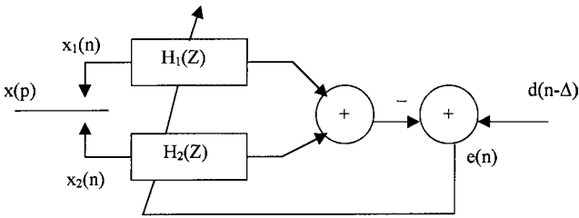
FIG. 12.8 Double sampling equalizer.
