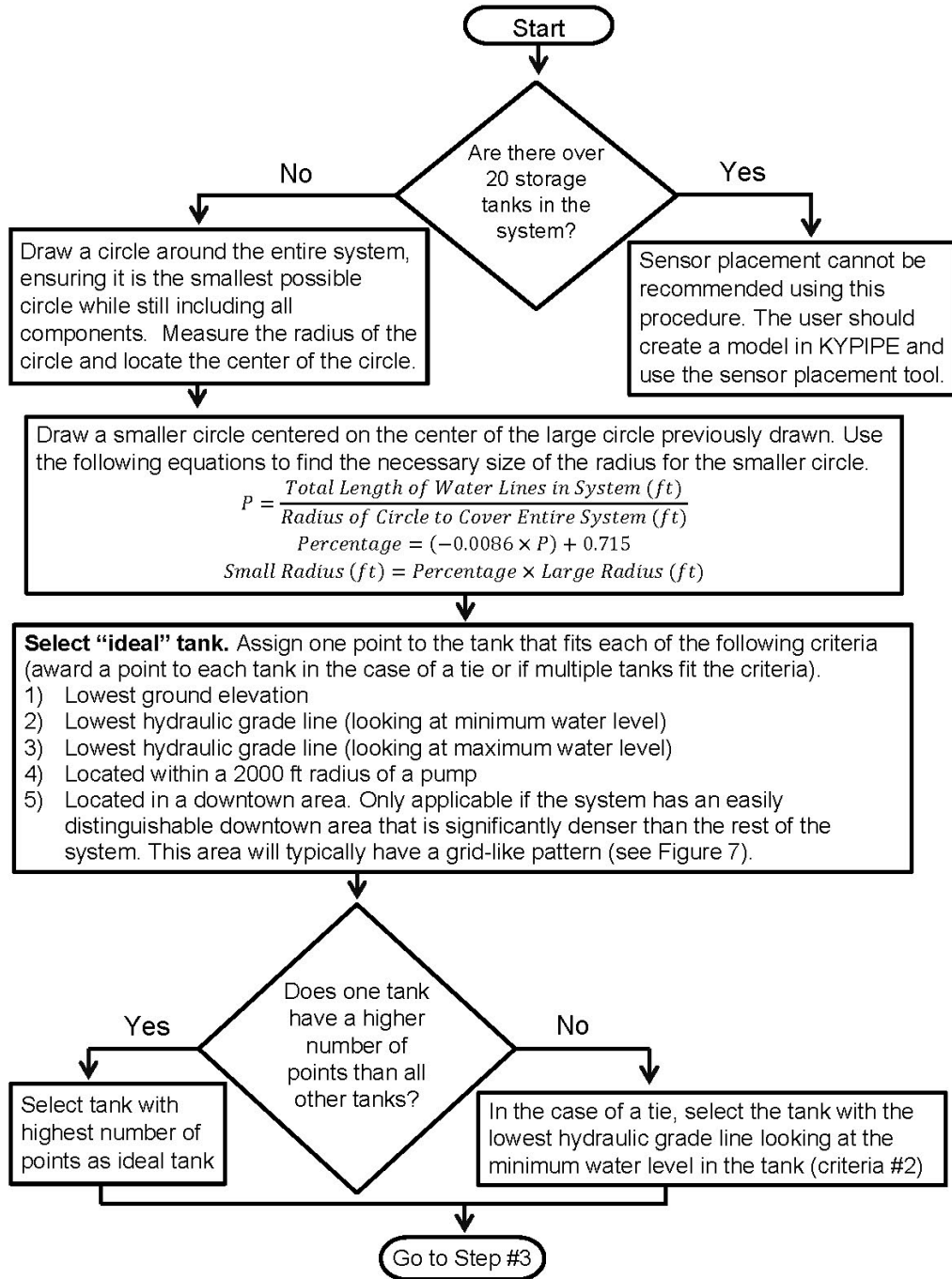
Figure 5.6: Step 2: Ideal Tank Selection (Branch Systems).
