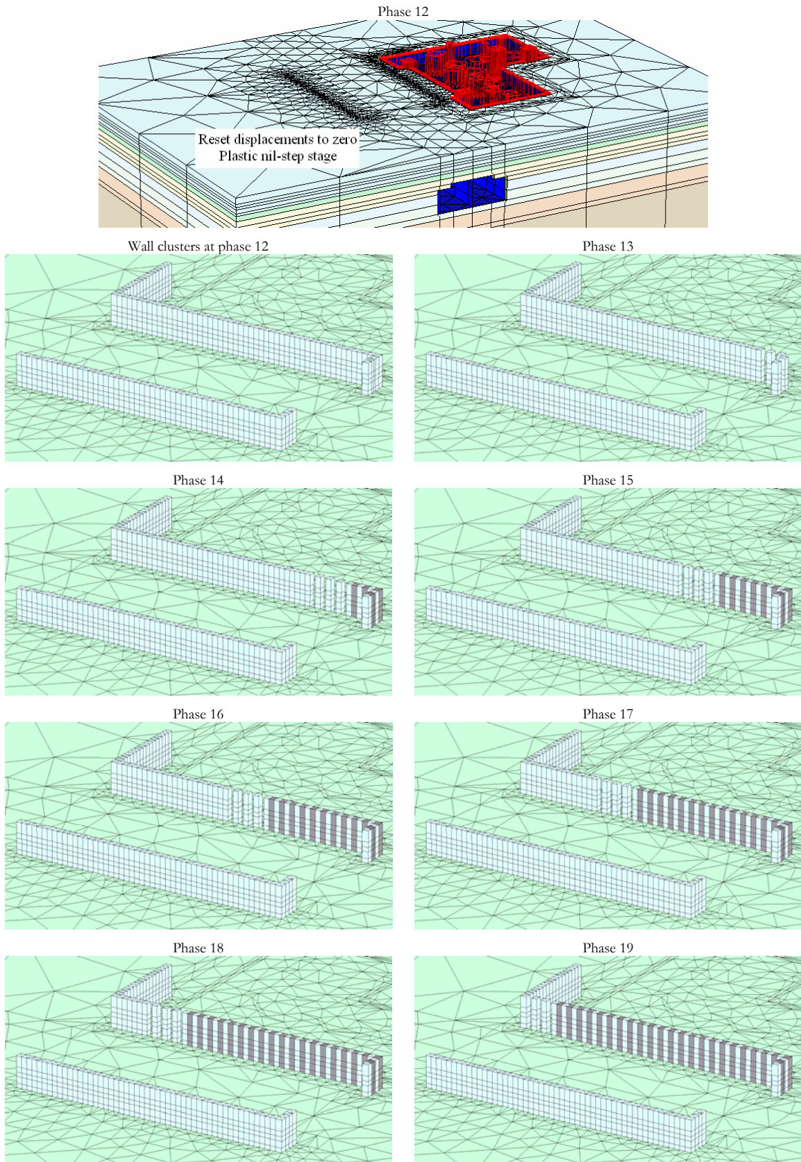
Figure A.8 - Modeling the Wall Installation in PLAXIS 3D FOUNDATION.
