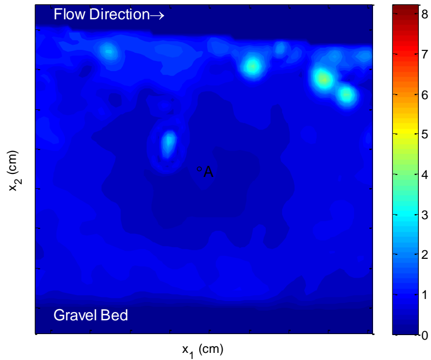
Figure 27. Test 1 Average Root-Mean-Square Velocity Fluctuations
