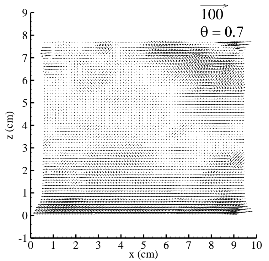
Figure 45. Galilean Transformation
