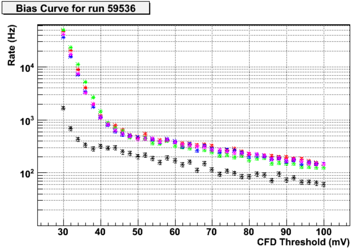
Figure 3.28 A bias curve taken on December 29, 2011, after the commissioning of the ANL/ISU pattern trigger, and prior to the VERITAS II camera upgrade. The L2 rates for T1 (red), T2 (green), T3 (blue), and T4 (purple) are shown, as well as the array trigger rate (black). The inflection point in the array rate indicates the minimum allowable CFD threshold that can be set for observations. Standard observations during this array configuration were taken with a CFD threshold of 50 mV.
