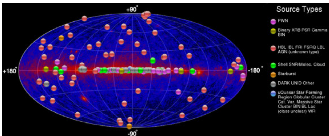
Figure 1.2 Skymap of resolved sources of VHE \gamma -rays, superimposed over the diffuse HE \gamma -ray background as seen by the Fermi Gamma-Ray Space Telescope. From: http://tevcap.uchicago.edu .
