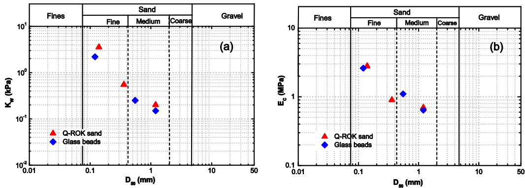
Figure 3.8: Grain size effect on the value of (a) air-entry parameter K_w and (b) critical breakage energy E_c .
