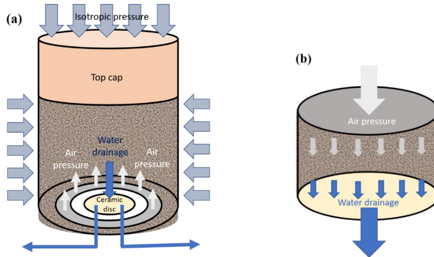
Figure 5.4: A schematic view of flow direction of air pressure and water drainage: (a) HPIC; (b) Tempe cell
