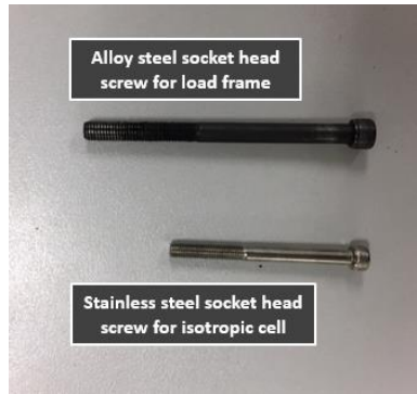
Figure 5.14: Socket head screws for load frame (above) and for isotropic cell (below)
