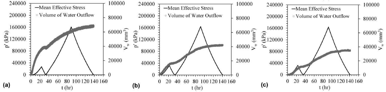
Figure 2.6: Change of mean effective stress and water outflow in time of clay specimen with different initial degree of saturation during drained compression: (a) S_r = 1.0 ; (b) S_r = 0.9 ; (c) S_r = 0.8
