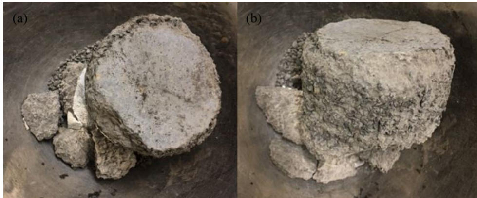
Figure 6.9: Picture of shale sand specimen after high pressure compression under 160 MPa: (a) Dried specimen; (b) Saturated specimen
