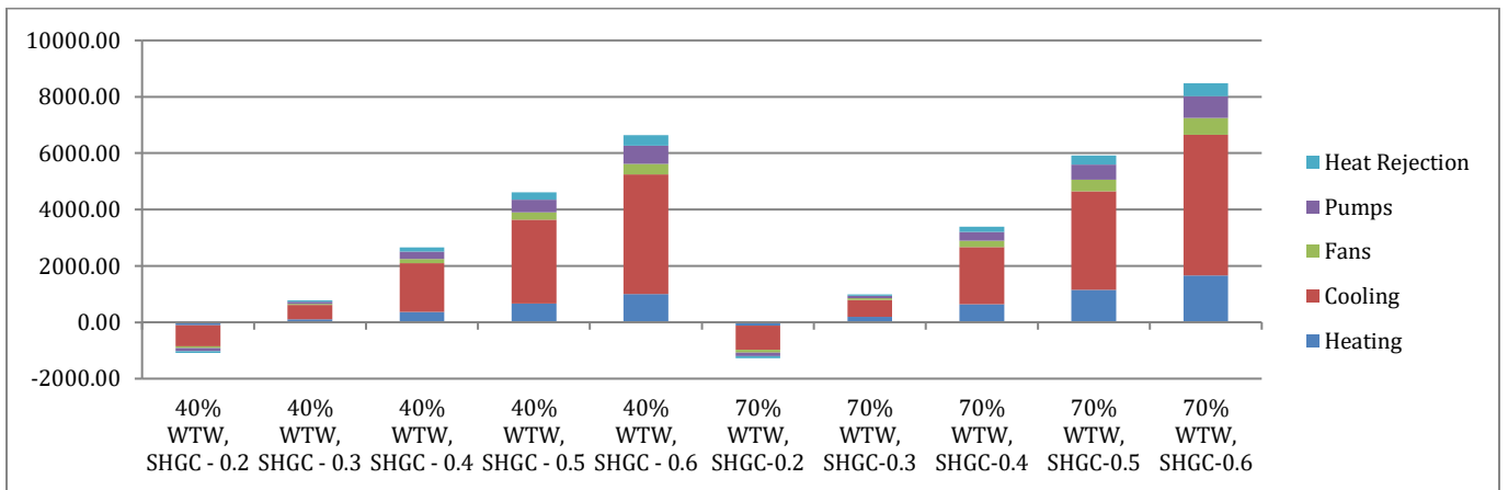
Figure 173: SHGC - Energy Consumption Difference from Baseline - Houston, TX
