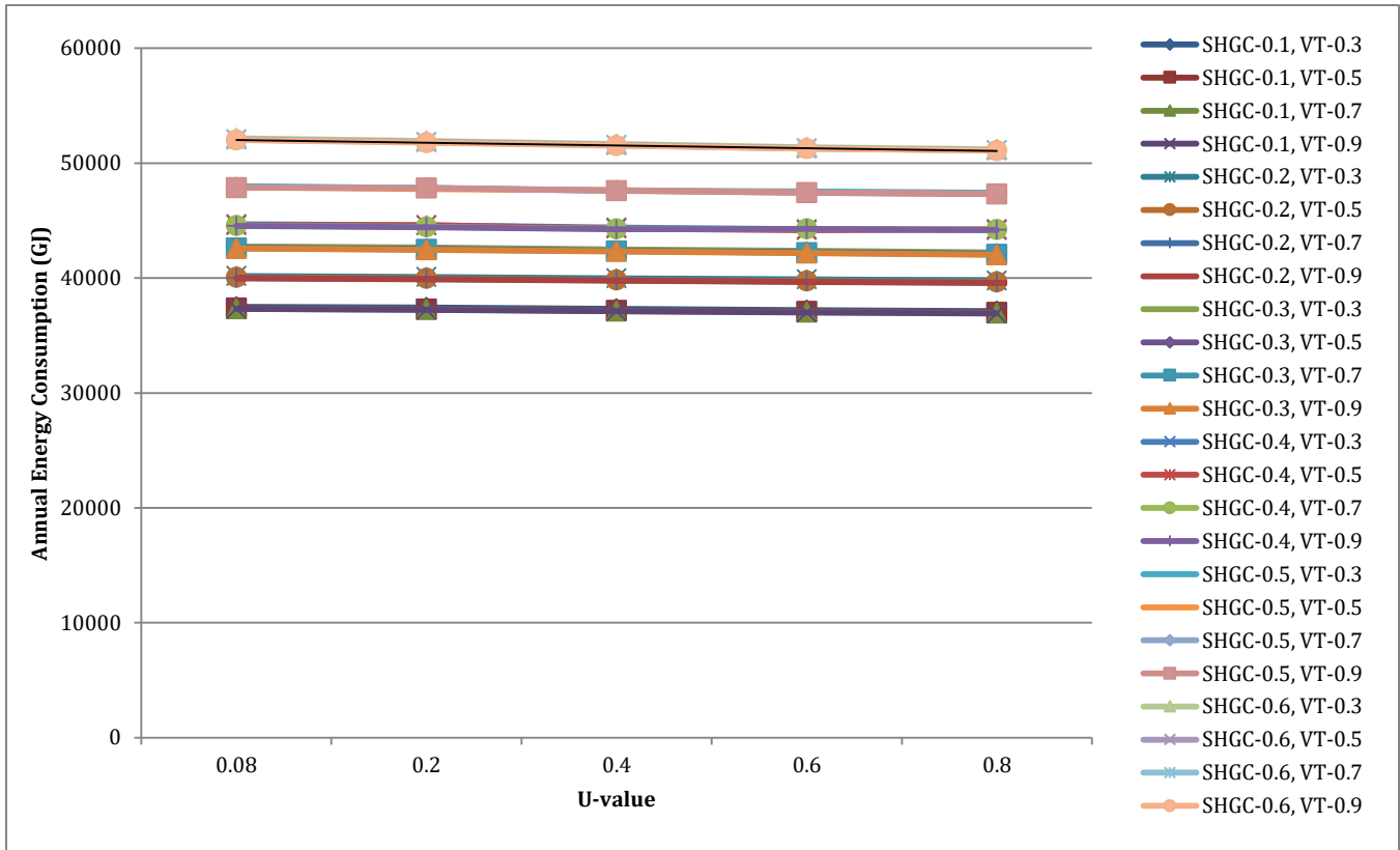
Figure 66: Annual Energy Consumption vs. U-value - Miami, FL
