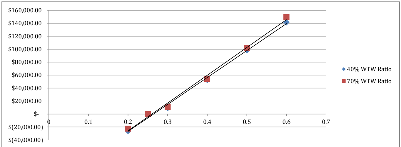
Figure 179: SHGC - Energy Cost Savings from Baseline - Phoenix, AZ
