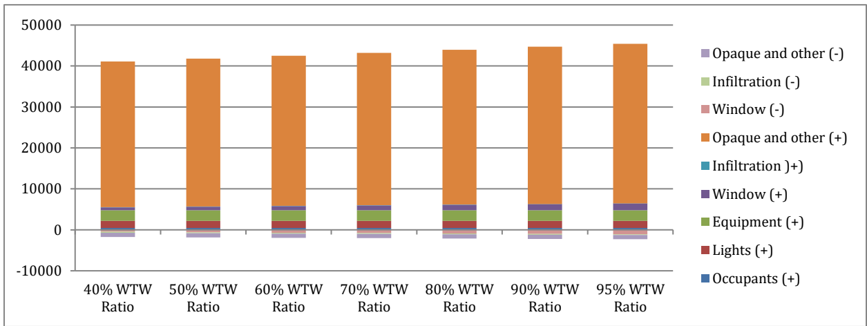
Figure 84: WTW Ratio - Sensible Gains - Houston, TX
