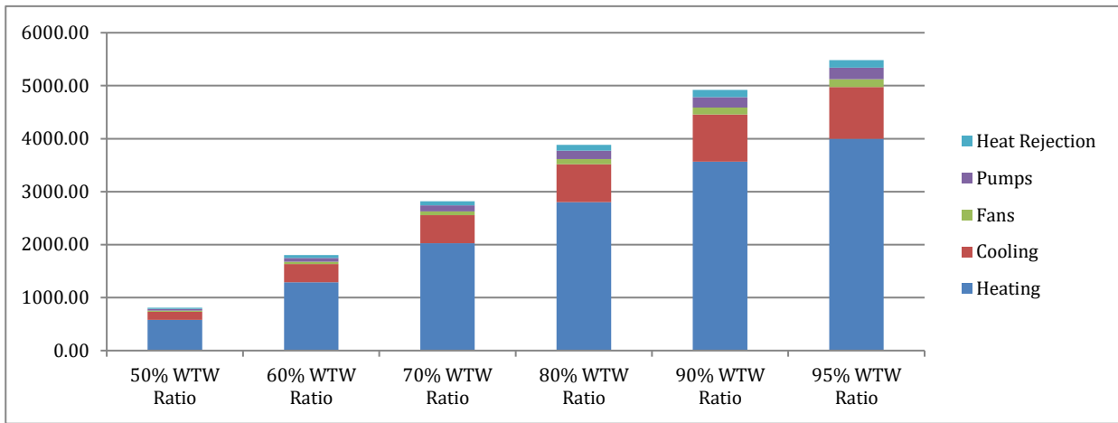
Figure 98: WTW Ratio - Energy Consumption Difference from Baseline - San Francisco, CA
