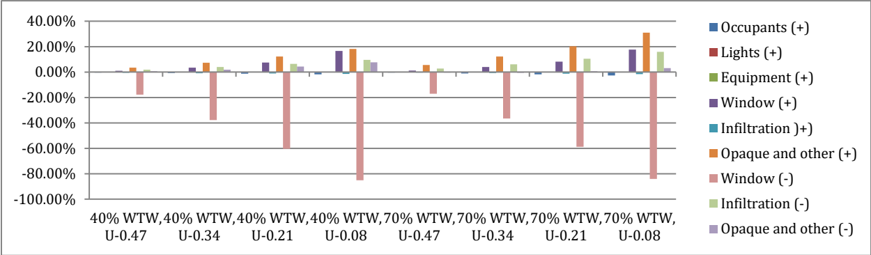
Figure 136: Window U-value - Sensible Gains % Difference from Baseline -Atlanta, GA
