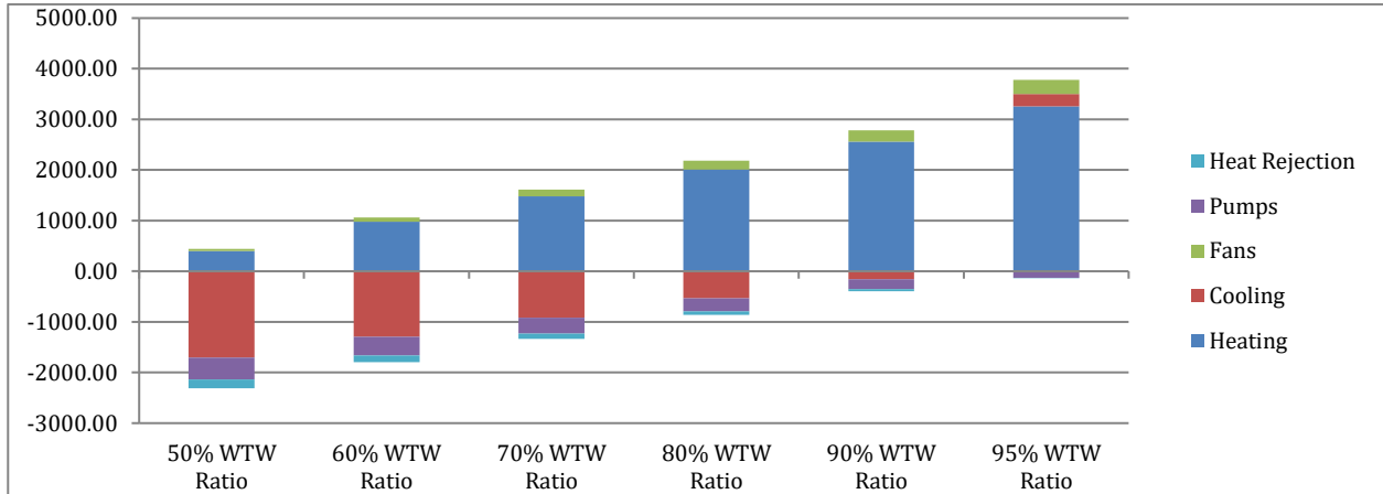
Figure 86: WTW Ratio - Energy Consumption Difference from Baseline - Houston, TX
