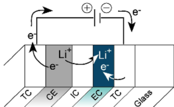
Figure 7: Cross-section of a SAGE Electrochromic window [20]
