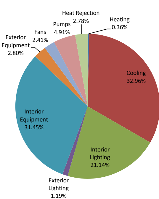
Figure 23: Miami Annual End Use Energy
