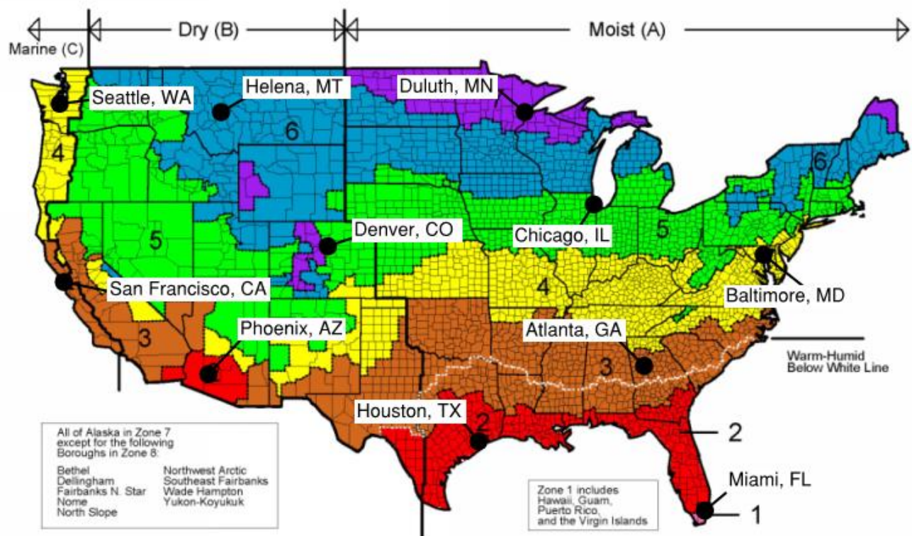
Figure 19: ASHRAE Climate Zone classifications and representative cities [84]
