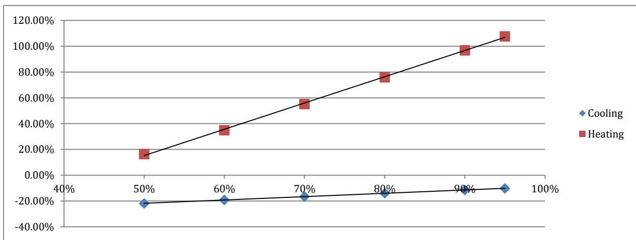
Figure 103: WTW Ratio - Heating and Cooling Energy % Difference from Baseline - Baltimore, MD
