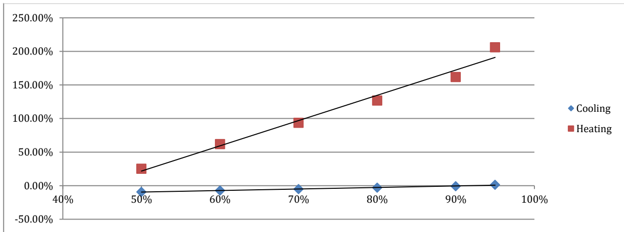
Figure 87: WTW Ratio - Heating and Cooling Energy % Difference from Baseline - Houston, TX
