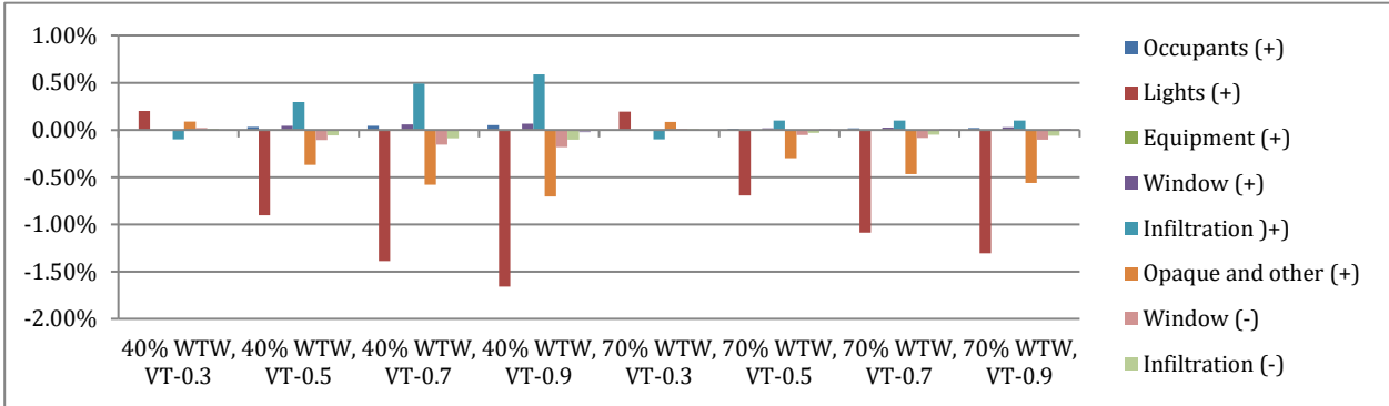
Figure 148: Window U-value - Sensible Gains % Difference from Baseline - Seattle, WA
