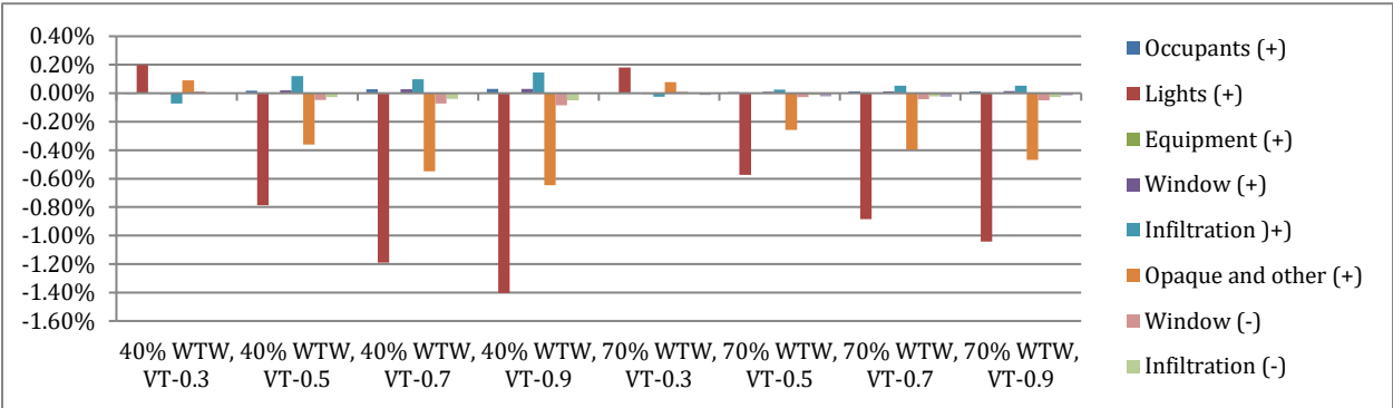
Figure 160: Window U-value - Sensible Gains % Difference from Baseline - Helena, MT
