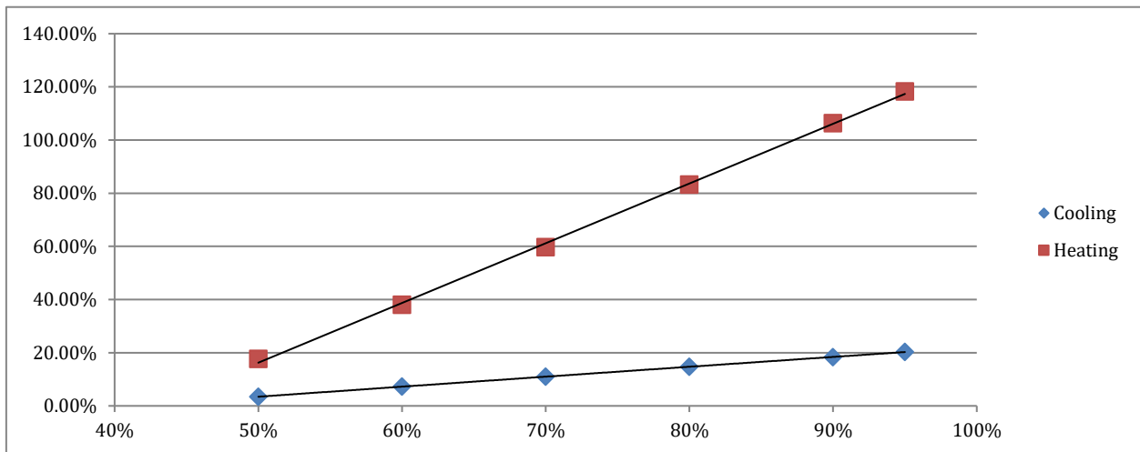
Figure 115: WTW Ratio - Heating and Cooling Energy % Difference from Baseline - Denver, CO
