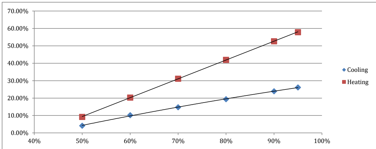
Figure 123: WTW Ratio - Heating and Cooling Energy % Difference from Baseline - Duluth, MN
