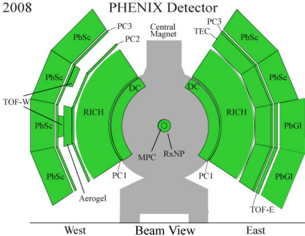
Figure 4.1 A view along the beam pipe for PHENIX central arm detectors in Run8.
