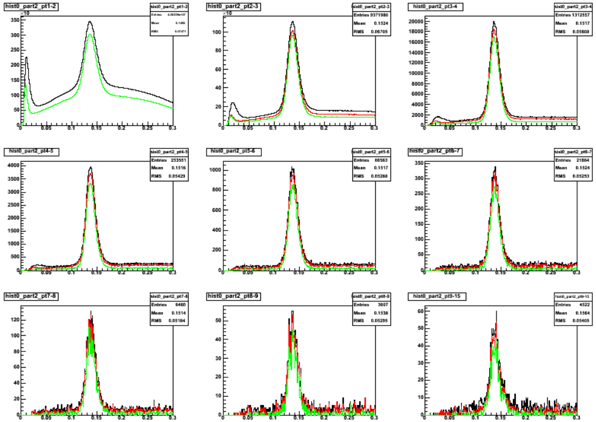
Figure 7.4 Photon pair invariant mass spectra of PbPb at east arm with p_T in various range in the order of left to right and top to bottom. Black lines indicate the spectra by applying minimum photon energy cut in all reconstructed \pi^0 . Red lines indicate the spectra by applying additional photon-prob cut based on black lines. Green lines indicates the spectra by applying additional di-photon energy asymmetry cut based on red lines.
