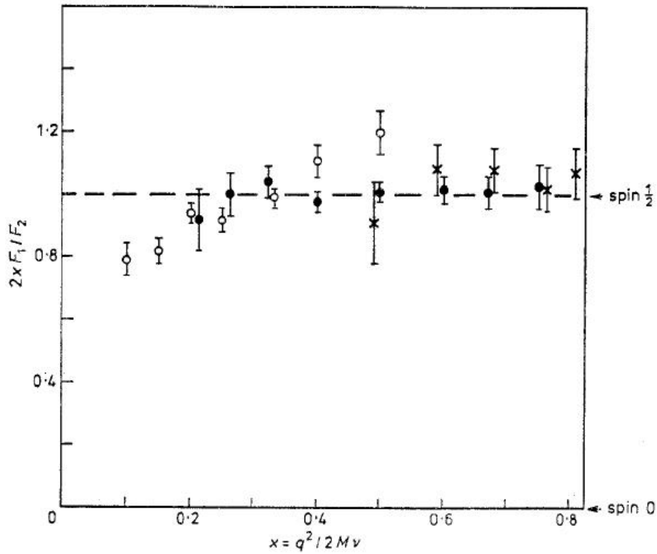
Figure 1.2 The ratio \frac{2xF_1}{F_2} as a function of x for three ranges of q^2 (from Riordan et. al. 1975). For point-like asymptotic region ( q^2 \rightarrow \infty ). \circ , q^2 = 1 - 3\text{GeV} ; \bullet , q^2 = 4 - 10\text{GeV} ; \times , q^2 = 12 - 16\text{GeV} ; --- , Callan-Gross as q^2 \rightarrow \infty .
