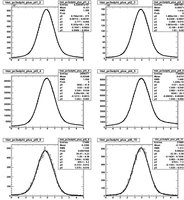
Figure 7.6 The pc3sdphi distribution by using double Gaussian fitting for positive charged tracks in p_T range of 1–2, 2–3, 3–4, 4–5, 5–6 and 6–15GeV in order of left to right and top to bottom, where parameters p1, p2 are mean and width of wide (background) Gaussian, p4 and p5 are mean and sigma of narrow (signal) Gaussian.
