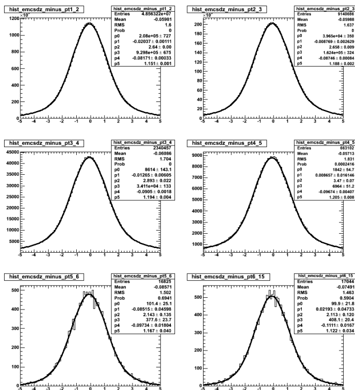
Figure 7.13 The emcsdz distribution by using double Gaussian fitting for negative charged tracks in p_T range of 1 – 2, 2 – 3, 3 – 4, 4 – 5, 5 – 6 and 6 – 15GeV in order of left to right and top to bottom, where parameters p1, p2 are mean and width of wide (background) Gaussian, p4 and p5 are mean and sigma of narrow (signal) Gaussian.
