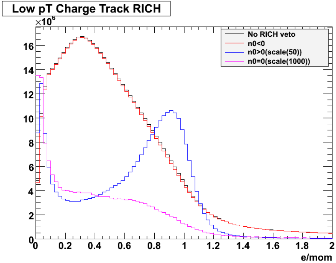
Figure 7.14 e/mom spectra for low p_T ( p_T < 4.7\text{GeV} ) charged tracks for various RICH cuts. The blue line shows e/mom has a peak near 1 when using the RICH cut n_0 > 0 , which essentially indicate electron signal. The spectra by using n_0 < 0 and n_0 = 0 cut do not show the electron signal.
