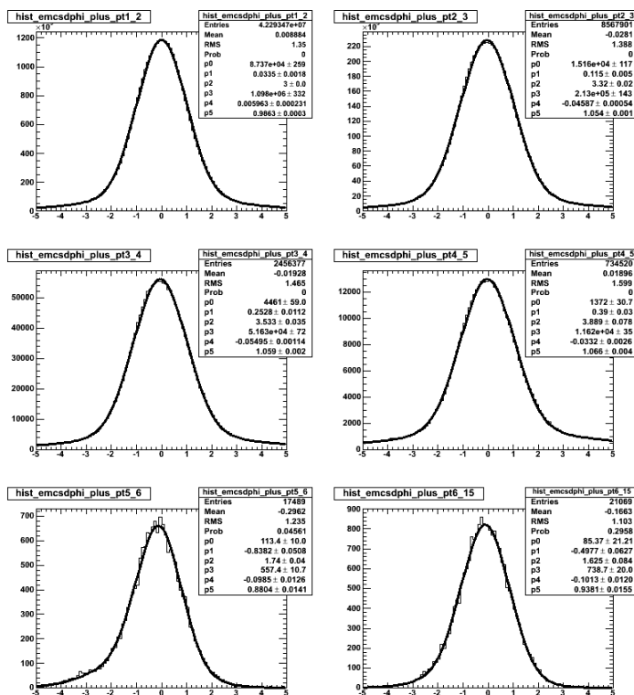
Figure 7.10 The emcsdphi distribution by using double Gaussian fitting for positive charged tracks in p_T range of 1 – 2, 2 – 3, 3 – 4, 4 – 5, 5 – 6 and 6 – 15GeV in order of left to right and top to bottom, where parameters p1, p2 are mean and width of wide (background) Gaussian, p4 and p5 are mean and sigma of narrow (signal) Gaussian.
