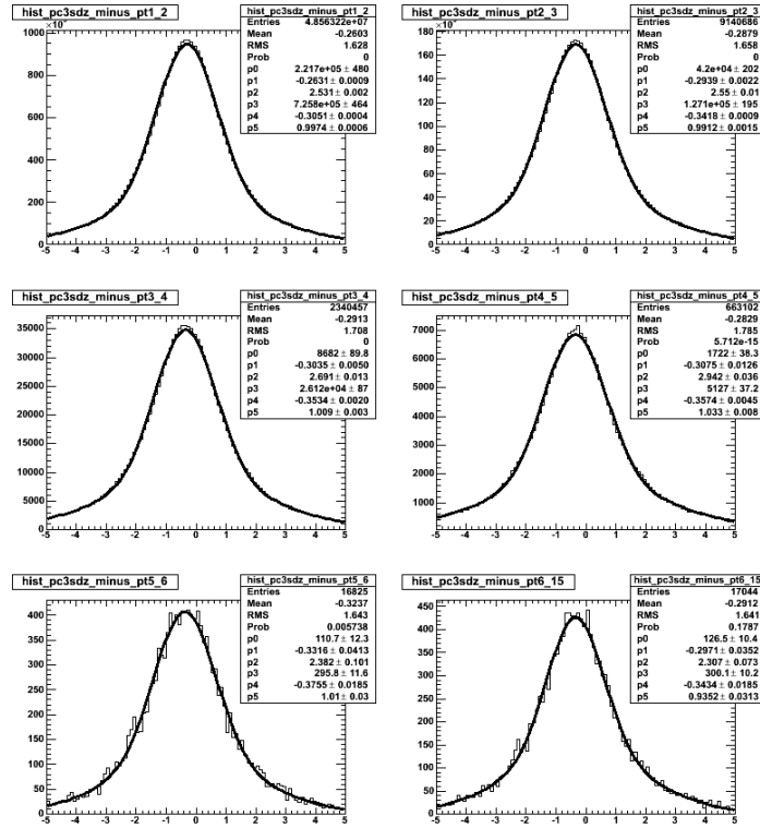
Figure 7.9 The pc3sdz distribution by using double Gaussian fitting for negative charged tracks in p_T range of 1 – 2, 2 – 3, 3 – 4, 4 – 5, 5 – 6 and 6 – 15GeV in order of left to right and top to bottom, where parameters p1, p2 are mean and width of wide (background) Gaussian, p4 and p5 are mean and sigma of narrow (signal) Gaussian.
