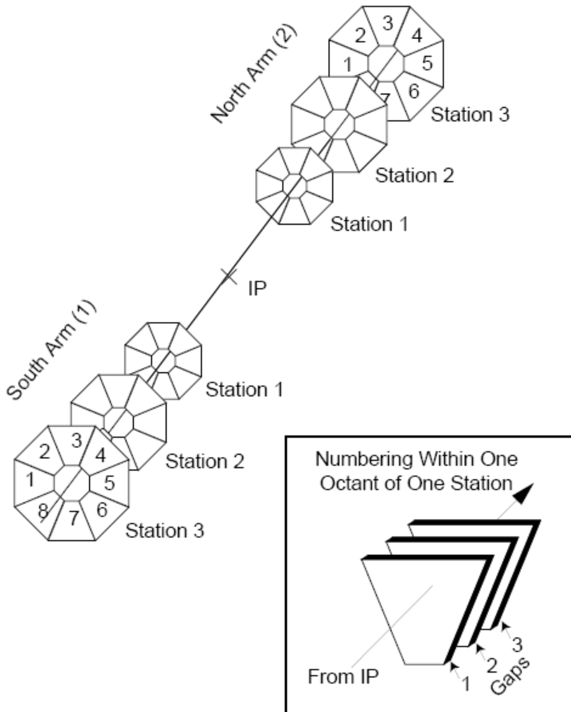
Figure 4.4 MuTR chamber description. Each MuTr station octant is actually instrumented in half octants (not depicted).
