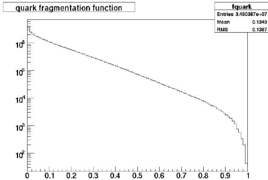
Figure 7.19 The quark fragmentation function used in the toy MC. The horizontal axis is partonix x , while the vertical axis is dN/dx .
