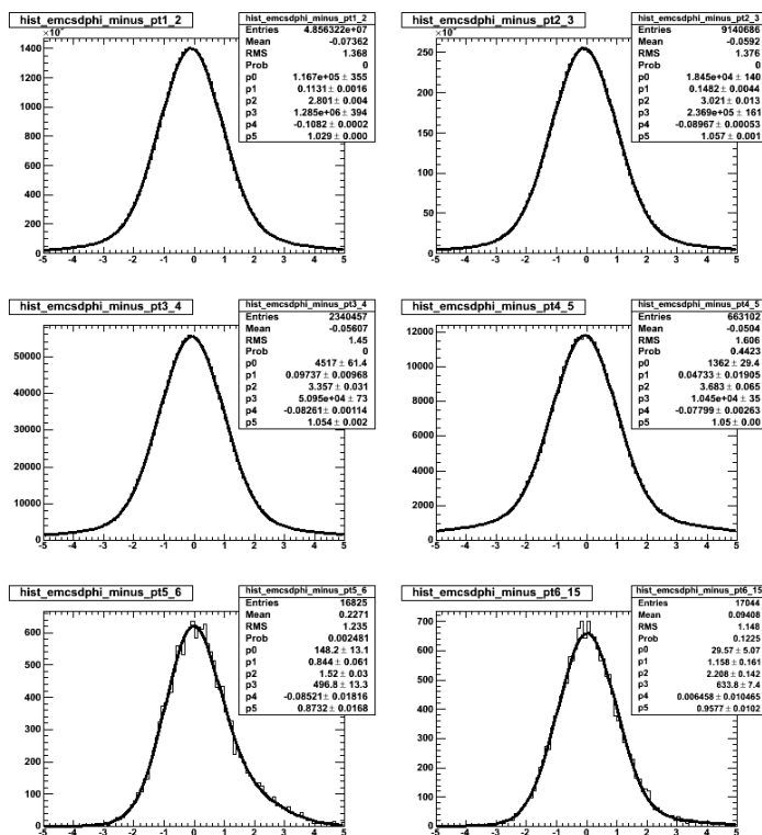
Figure 7.11 The emcsdphi distribution by using double Gaussian fitting for negative charged tracks in p_T range of 1 – 2, 2 – 3, 3 – 4, 4 – 5, 5 – 6 and 6 – 15 GeV in order of left to right and top to bottom, where parameters p1, p2 are mean and width of wide (background) Gaussian, p4 and p5 are mean and sigma of narrow (signal) Gaussian.
