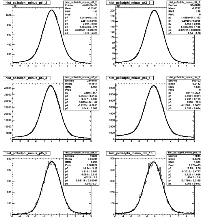
Figure 7.7 The pc3sdphi distribution by using double Gaussian fitting for negative charged tracks in p_T range of 1 – 2, 2 – 3, 3 – 4, 4 – 5, 5 – 6 and 6 – 15GeV in order of left to right and top to bottom, where parameters p1, p2 are mean and width of wide (background) Gaussian, p4 and p5 are mean and sigma of narrow (signal) Gaussian.
