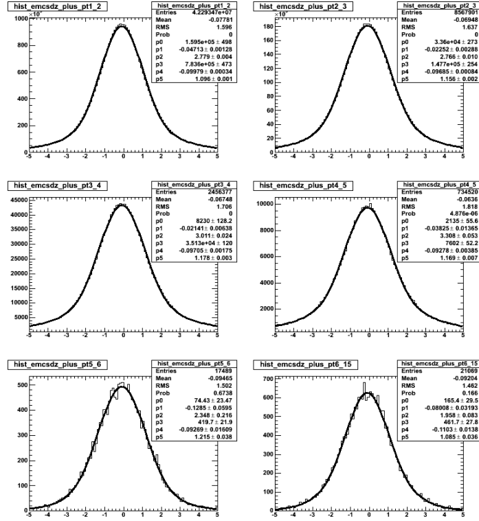
Figure 7.12 The emcsdz distribution by using double Gaussian fitting for positive charged tracks in p_T range of 1 – 2, 2 – 3, 3 – 4, 4 – 5, 5 – 6 and 6 – 15GeV in order of left to right and top to bottom, where parameters p1, p2 are mean and width of wide (background) Gaussian, p4 and p5 are mean and sigma of narrow (signal) Gaussian.
