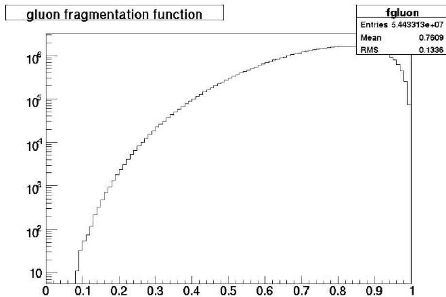
Figure 7.20 The gluon fragmentation function used in the toy MC. The horizontal axis is partonix x , while the vertical axis is dN/dx .
