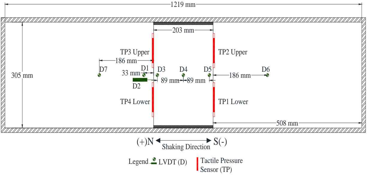
Figure 3-28. Plan view of Test 7.
