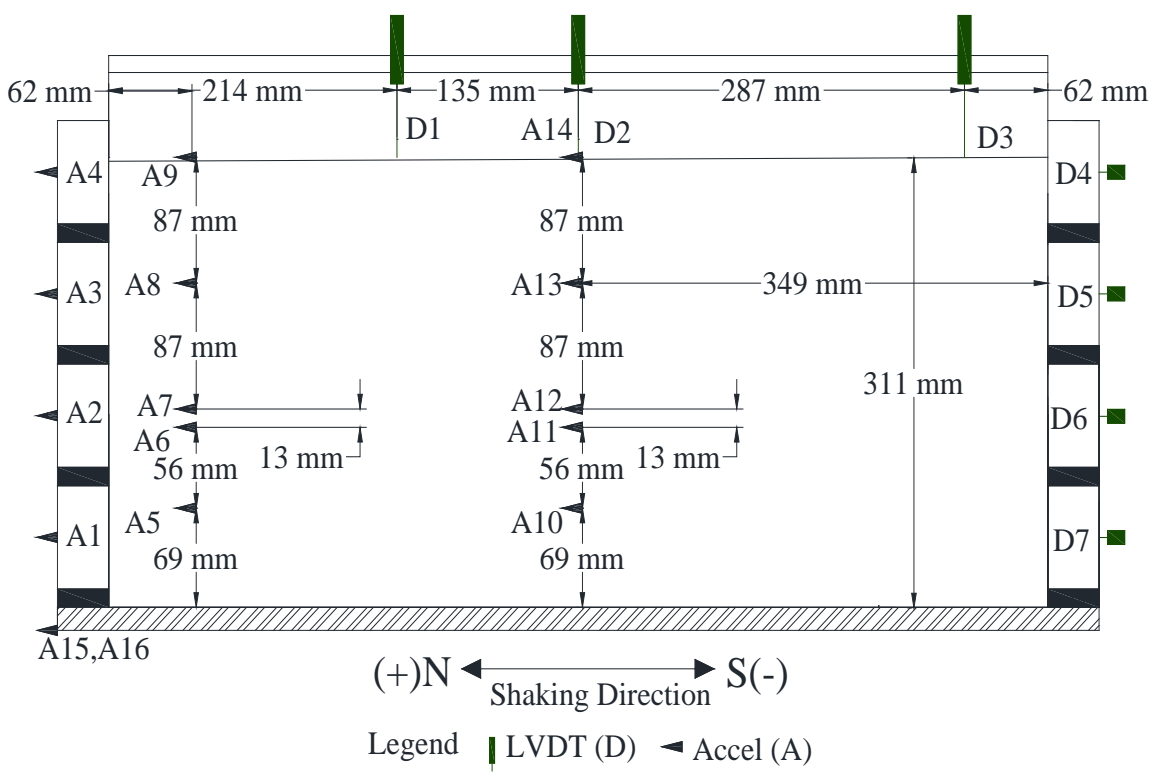
Figure 3-29. Elevation view of Free Field test.
