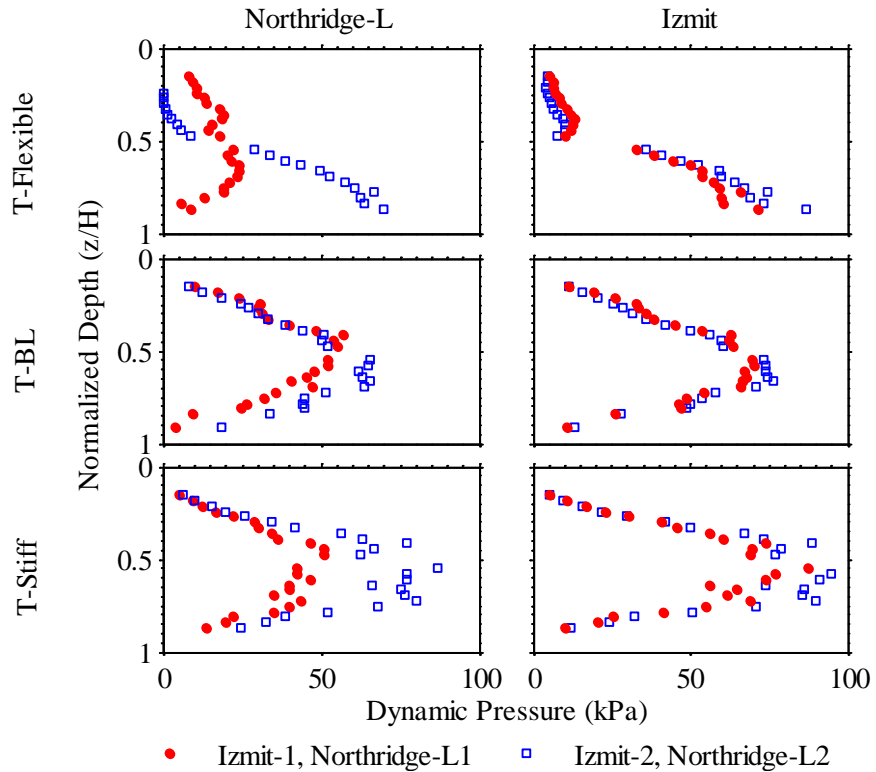
Figure 4-40. Dynamic increment of earth pressures ( \Delta\sigma_E ) at time of maximum thrust during the two sets of Northridge-L and Izmit motions in T-Flexible, T-BL, and T-Stiff.
