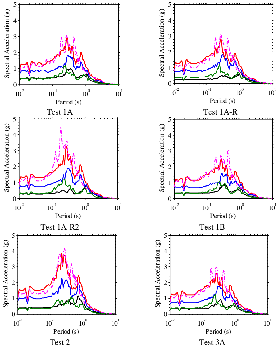
Figure 3-56. Acceleration response spectra (5%-damped) of the recorded base motions in Tests 1A, 1A-R, 1A-R2, 1B, 2, and 3A.
