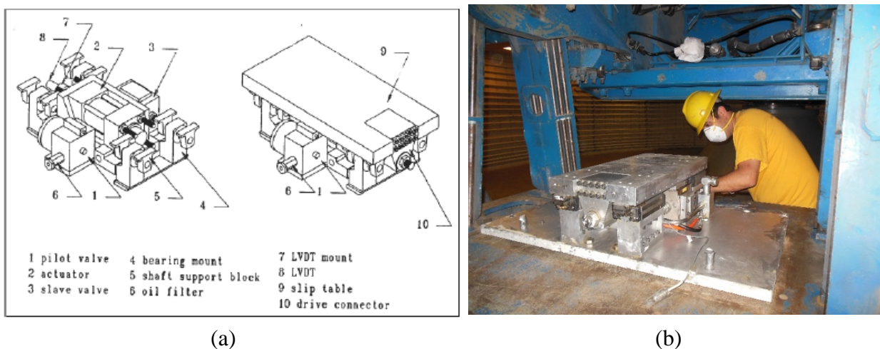
Figure 3-2. (a) Schematic (Ketchum 1989) and (b) picture of installation of shake table.
