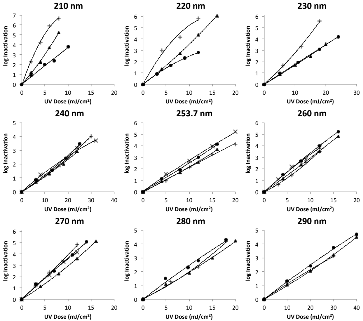
Figure C.1. Dose response of T1UV Coliphage to wavelength-specific UV irradiation from the tunable laser. Note different x- and y-axis values. Symbols represent data from four separate trials: R1 (●) and R2 (▲) from one laboratory and R3 (+) and R4 (×) from two additional laboratories. Average standard deviation from replicate platings = 5.5 pfu/mL.
