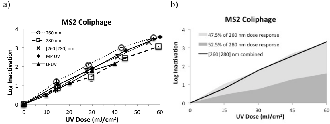
Figure 6.3. a) Dose response of MS2 coliphage to UV irradiation from UV LEDs emitting at 260 nm, 280 nm, 260/280 nm combined, compared with its dose response to MP and LP UV light. b) Dose response of a 260|280 nm combined LED unit on inactivating MS2 coliphage compared with the sum of its dose response from separate LED exposures.
