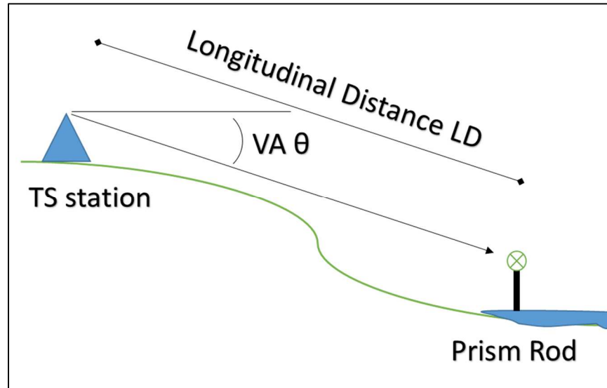
FIGURE 3-2 SIDWAYS VIEW OF TOTAL STATION SETUP. THE TOTAL STATION IDEALLY IS ABOVE THE STREAM ON A HIGH BANK WITH VIEWS OF THE ENTIRE CHANNEL AND POINTS WORTH RECORDING. THE VERTICAL ANGLE AND LONGITUDINAL DISTANCE ARE GATHERED IN THIS SHOT.
