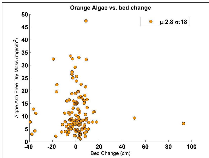
FIGURE 4-44 ORANGE MICROBIAL MAT AFDM VS OVERALL BED CHANGE. ORANGE MATS ARE PRIMARILY LOCATED IN THE THALWEG OR DEEPEST PART OF A STREAM CHANNEL. THESE FILAMENTOUS ALGAE ARE ABLE TO WITHSTAND LARGE FLUCTUATIONS IN FLOW WHILST REMAINING UNSCOURED. THE FIGURE ABOVE SHOWS ORANGE MATS BEING CAPABLE OF WITHSTANDING LARGE BED CHANGES UP TO 90 CM IN DEPOSITION AND 40 CM OF SCOURING.
