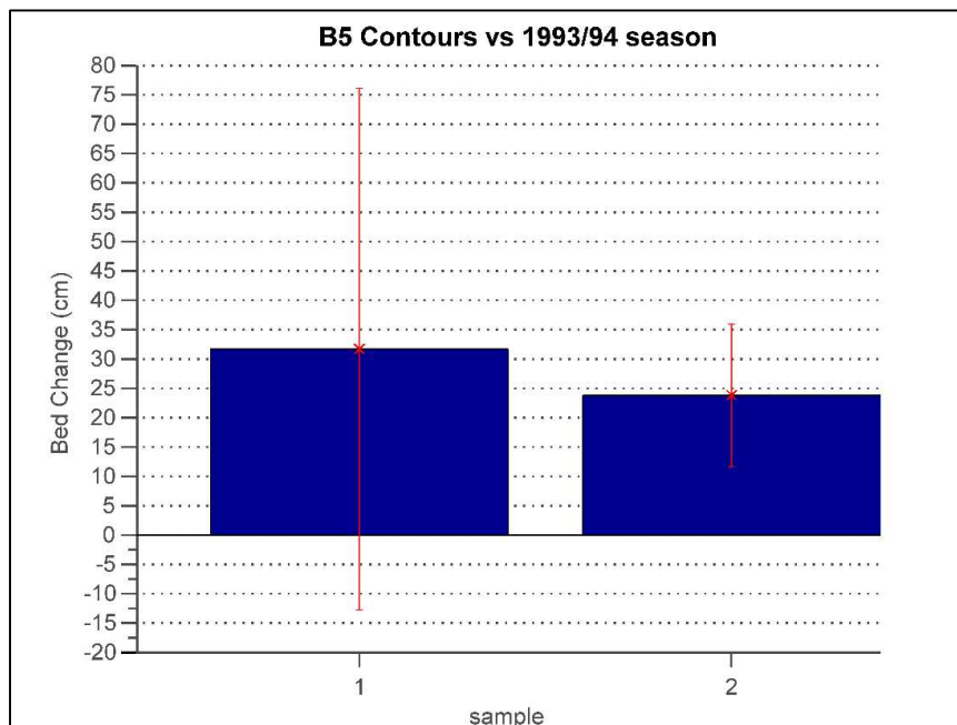
FIGURE 4-37 CONTOUR CHANGE DETECTION FOR BOHNER CREEK. SIMILAR TO FIGURE 4-36, THERE IS LARGE STANDARD ERROR ASSOCIATED WITH THE LEFT BAR WHICH DESCRIBES AVERAGE RELATIVE BED CHANGE DERIVED FROM A DRAWN CONTOUR PLOT. ON THE RIGHT IS THE DATA FROM THE 1993/94 SURVEY AND CONTAINS MUCH LESS STANDARD ERROR.
