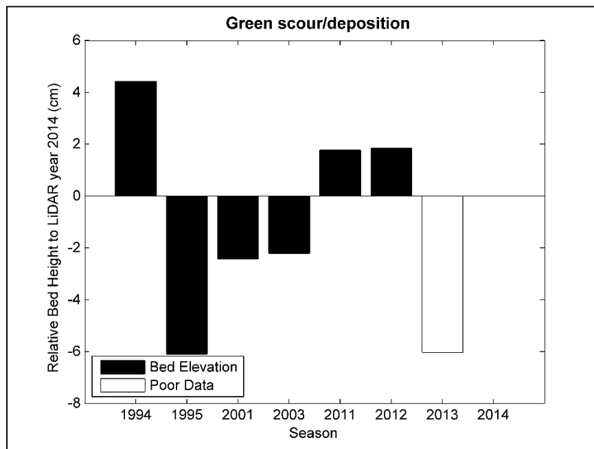
FIGURE 4-9 AVERAGE RELATIVE ELEVATION CHANGE FOR GREEN CREEK. THE 2012/13 SEASON DID NOT HAVE ENOUGH POINTS OUTSIDE OF STREAM CHANNEL TO SIGNIFICANTLY REPRESENT AREA WITHIN STREAM CHANNEL.
