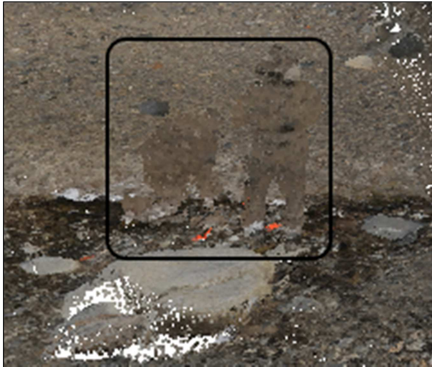
FIGURE 3-6 ELEVATION RELICT 1. LOOKING NORTH, A FIELD TEAM SAMPLING MICROBIAL MATS IS CAUGHT IN THE LIDAR SCAN AFFECTING THE LONGITUDINAL DISTANCE OF THE RETURN BEAM. ON LEFT, TEAM MEMBER ON KNEES SAMPLING MATS WHILE ON RIGHT THE OTHER MEMBER IS TAKING NOTES.
