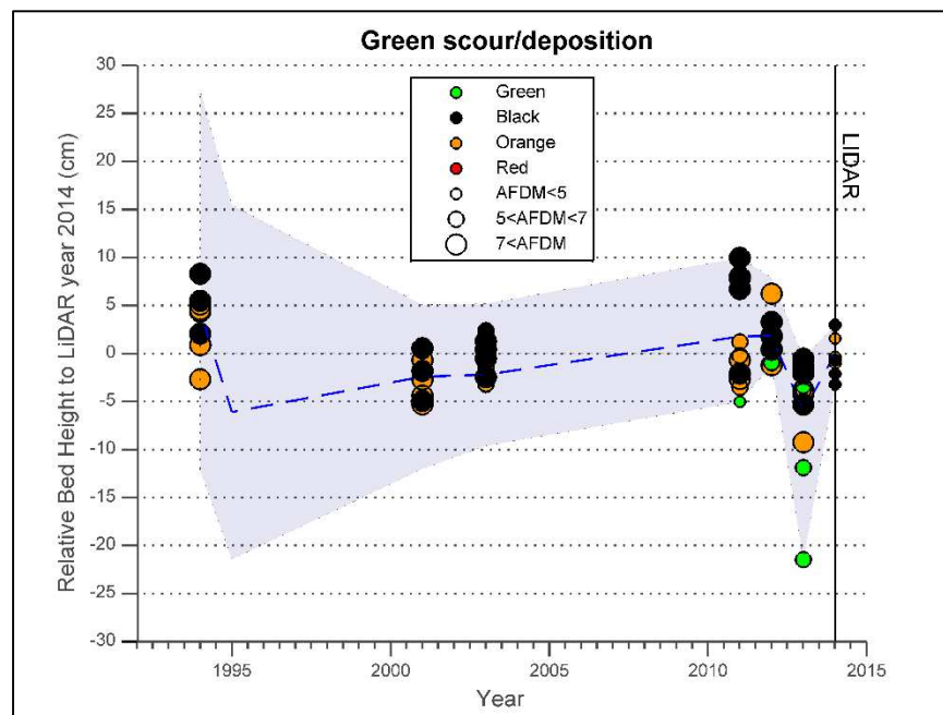
FIGURE 4-7 RELATIVE BED CHANGE PROFILE FOR GREEN CREEK. ALL TYPES OF MICROBIAL MATS ARE FOUND HERE WITH THE EXCEPTION OF RED ALGAE. THE ORIGINAL SURVEY SAW AN AVERAGE BED ELEVATION APPROXIMATELY THE SAME AS DURING THE LIDAR SCAN, BUT VARIATION IN THE SURVEYED POINTS EXCEEDS 25 CM DIFFERENCE. GREEN CREEK IS GENERALLY STATIC AND SEES VERY FEW FLOWS ABLE TO CAUSE LARGE CHANGES IN STREAM BED.
