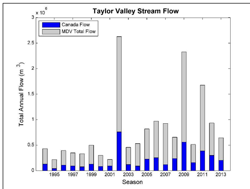
FIGURE 4-3 TOTAL ANNUAL FLOW FOR MDV AND CANADA STREAM. CANADA STREAM IS A MAJOR CONTRIBUTOR OF WATER TO LAKE FRYXELL. OF THE 7 STREAMS ANALYZED, CANADA STREAM HAS THE LARGEST OVERALL VOLUME OF WATER FOR EACH SEASON.
