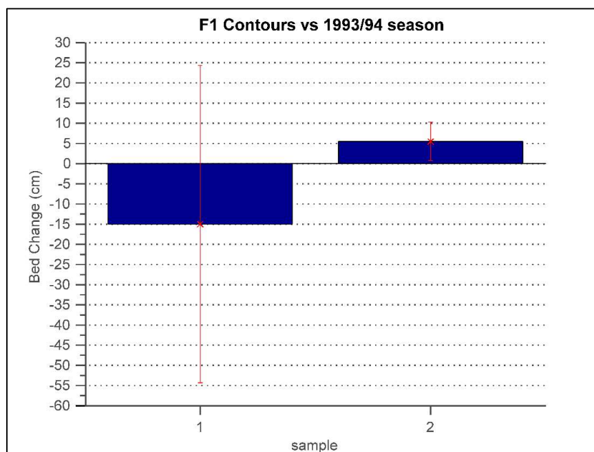
FIGURE 4-36 CONTOUR CHANGE DETECTION FOR CANADA STREAM. ON THE LEFT IS THE DIGITIZED CONTOUR PLOT DESCRIBING AVERAGE RELATIVE BED ELEVATION. THE LARGE STANDARD ERROR IS COMMONLY SEEN ON ALL CONTOUR PLOT DIGITIZED ANALYSES. THE RIGHT BAR DESCRIBES THE RELATIVE BED ELEVATION USING THE 1993/94 SURVEY DATA AND CONTAINS MUCH SMALLER STANDARD ERROR.
