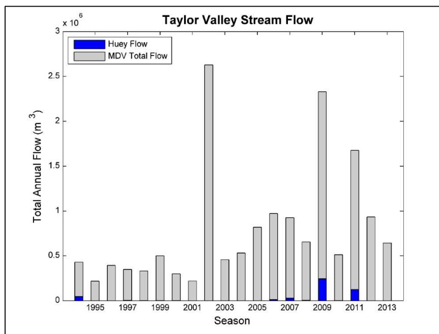
FIGURE 4-28 TOTAL ANNUAL FLOW FOR MDV AND HUEY CREEK. MANY SEASONS HUEY CREEK HAS NOT FLOWED OR THE DATA CORRUPT ENOUGH TO BE UNPUBLISHABLE. HUEY CREEK IS THE SMALLEST CONTRIBUTOR OF WATER IN COMPARISON TO STREAMS IN THIS STUDY.
