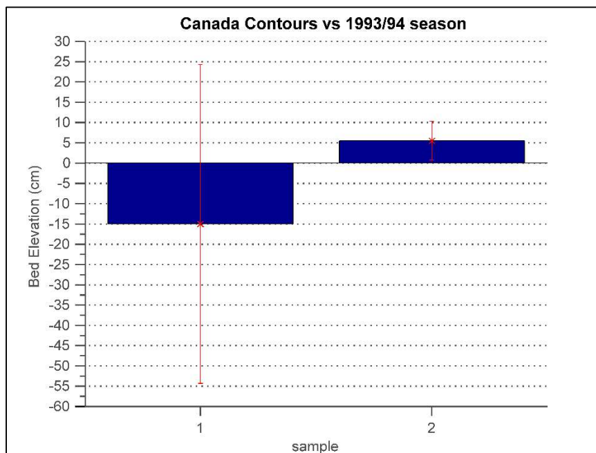
FIGURE 4-5 CANADA TRANSECT CONTOUR PLOT COMPARISON TO 1993/94 SURVEY. ERROR FOR CONTOUR LINES IS VERY LARGE AND THEREFORE NOT CONSIDERED FOR CHANGE DETECTION IN THIS STUDY WHILE SURVEY DATA HAS SMALL ERROR AND SHOWS AN AVERAGE RELATIVE ELEVATION CHANGE OF 6CM.
