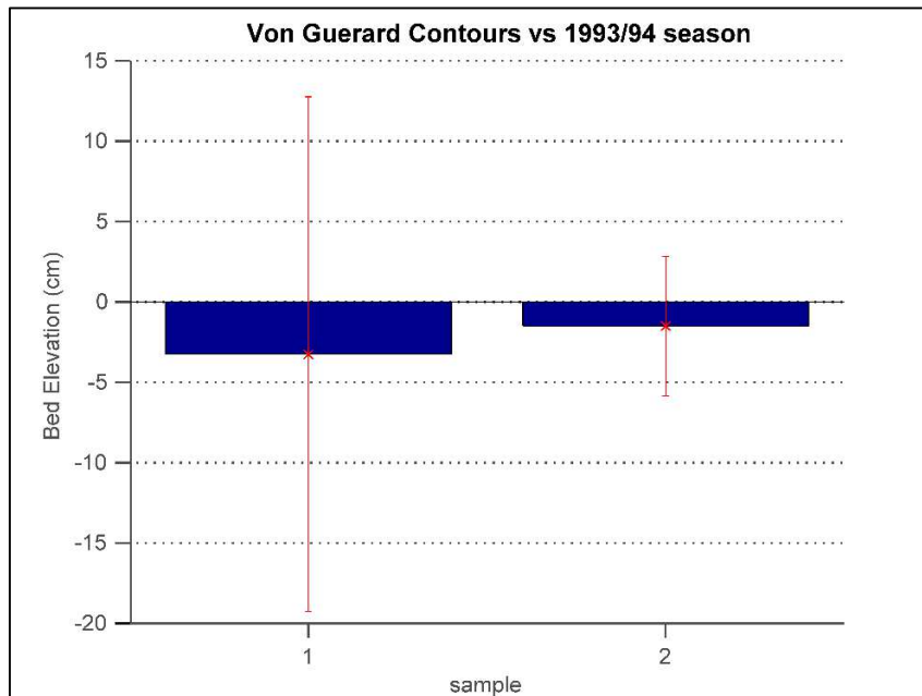
FIGURE 4-25 VON GUERARD TRANSECT CONTOUR PLOT COMPARISON TO 1993/94 SURVEY. SIMILARITIES IN AVERAGE BED ELEVATIONS ARE FOUND IN THE COMPARISON, BUT THE ERROR FOR THE CONTOUR PLOTS IS TOO HIGH TO BE CONSIDERED IN THIS STUDY.
