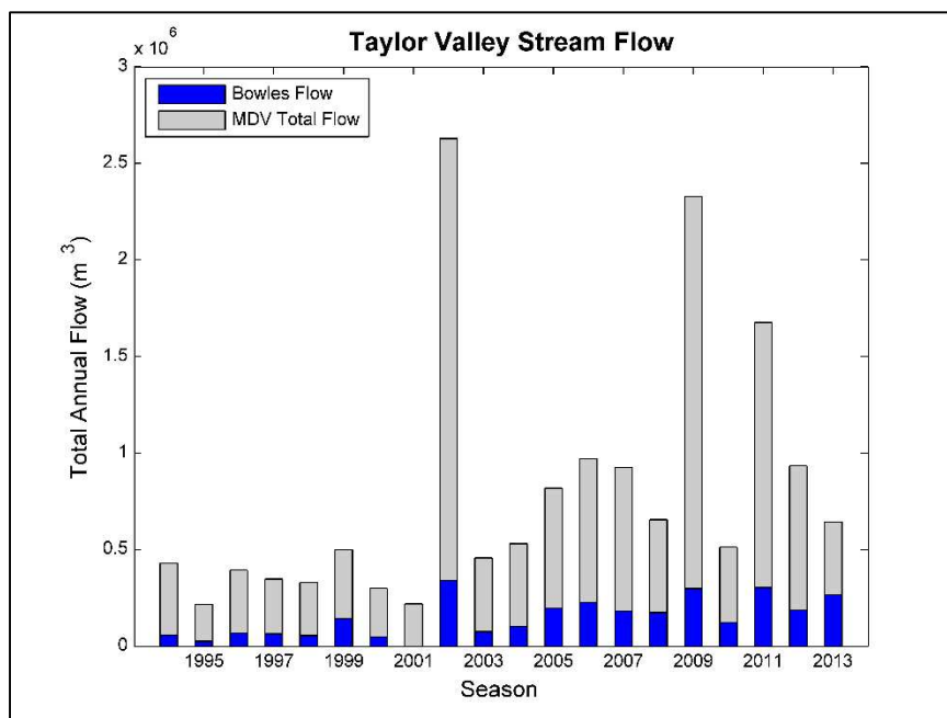
FIGURE 4-13 TOTAL ANNUAL FLOW FOR MDV AND BOWLES CREEK. HERE FLOW IS NOT ACTUALLY BOWLES CREEK DUE TO NO GAGE AT SITE. DATA IN BLUE IS REPRESENTED BY GREEN CREEK AS THEY SHARE SIMILAR FLOW PATTERNS, PEAKS, AND FLUCTUATIONS.
