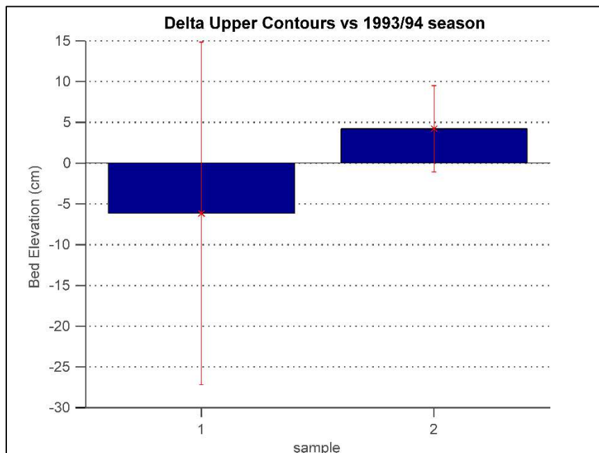
FIGURE 4-20 UPPER DELTA TRANSECT CONTOUR PLOT COMPARISON TO 1993/94 SURVEY. AS TYPICAL WITH CONTOUR PLOTS, AVERAGE BED CHANGE IS WITHIN BOUNDS, BUT STANDARD ERROR IS UNACCEPTABLE FOR USE IN THIS STUDY.
