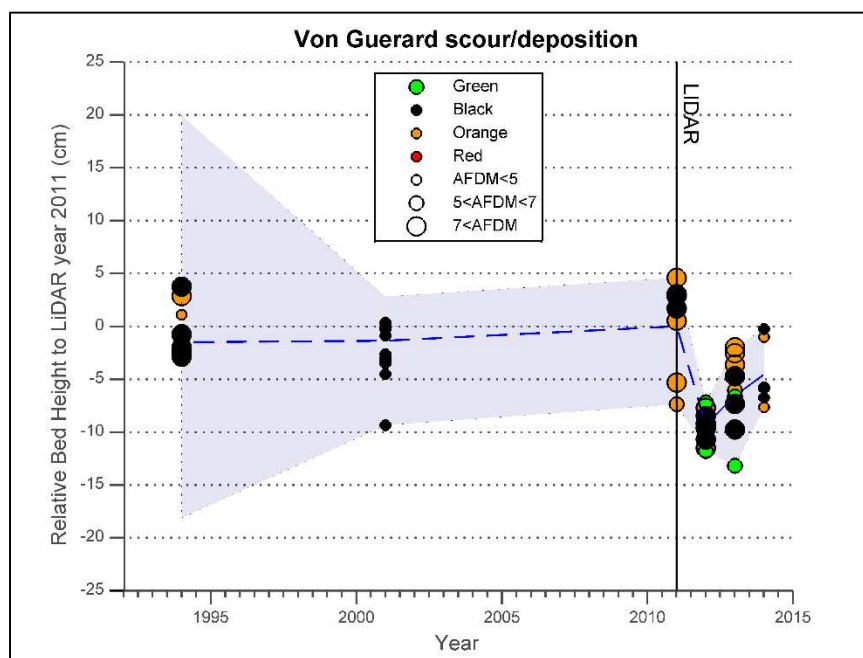
FIGURE 4-22 RELATIVE BED CHANGE PROFILE FOR VON GUERARD STREAM. TYPICAL OF A SHALLOW GRADIENT TRANSECT AND SANDY DELTAIC SUBSTRATE, VON GUERARD STREAM DOES NOT EXPERIENCE MUCH BED CHANGE. THERE IS MOBILITY IN THE SANDY BED, BUT IT IS NOT DEPOSITED AND CONTINUES DOWNSTREAM INTO LAKE FRYXELL.
