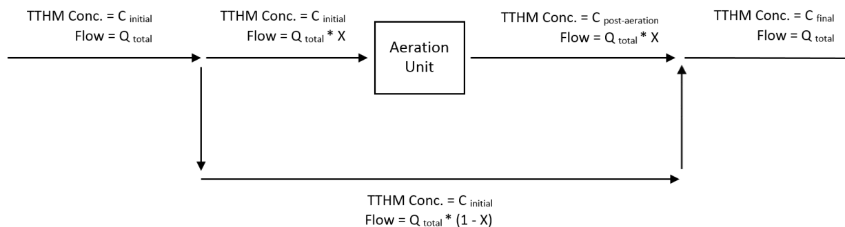
Figure A-2: TTHM mass balance around an aeration unit.
