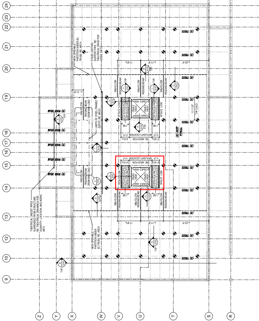
ROOF RECONSTRUCTION PLAN 1/8" = 1'-0"
