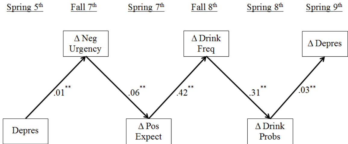
Figure 1. Negative Binomial Model (simplified). ** p < .001 ; Values are unstandardized beta weights; \Delta = prediction above and beyond autoregressive effects; Depres = depression; Neg Urgency = negative urgency; Positive Expect = positive expectancies; Drink Freq = drinking frequency; Drink Probs = problems from drinking.
