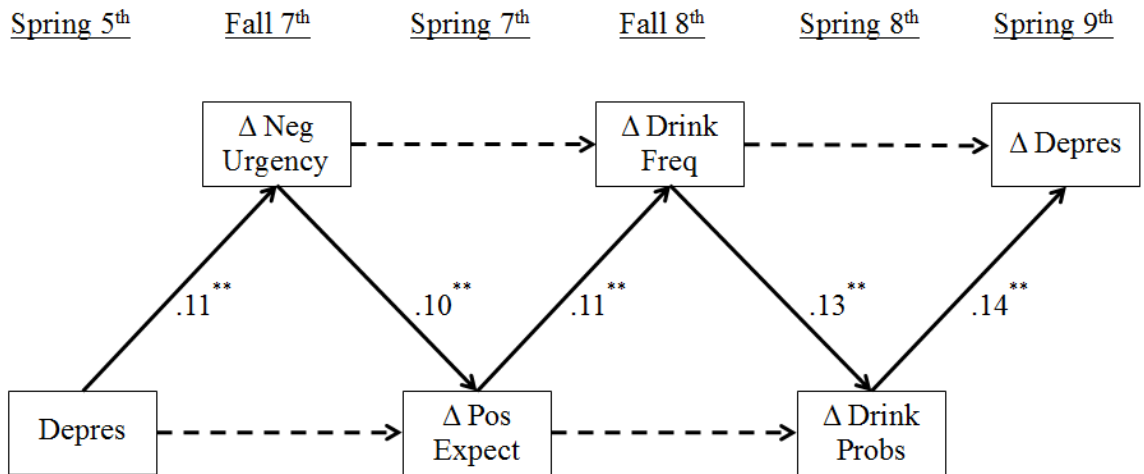
Figure 2. Maximum Likelihood Model (simplified). ** p < .001 ; Values are standardized beta weights; \Delta = prediction above and beyond autoregressive effects; Depres = depression; Neg Urgency = negative urgency; Positive Expect = positive expectancies; Drink Freq = drinking frequency; Drink Probs = problems from drinking; ----► = mediated pathways.
