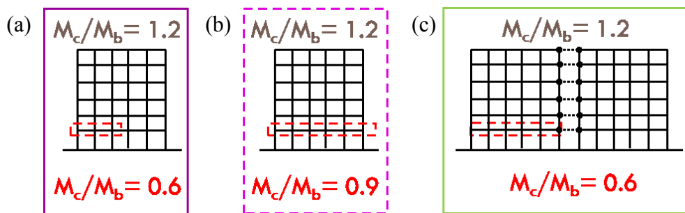
Figure 6-9. Schematic drawing of three cases to study the effect of the number of piers and the extent of deficiency M_c/M_b ratio in the first floor.
