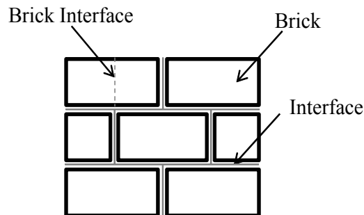
Figure 2-17. Simplified micro-modeling (meso-modeling) approach for masonry or infill walls.
