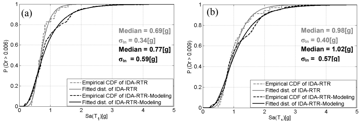
Figure 7-6. Comparison between fragility curves computed considering RTR variability only (gray lines) and RTR and modeling variability (black lines) for the unbiased data. The fragility curves computed represent the probability of drifts exceeding a) 0.006 and b) 0.009.
