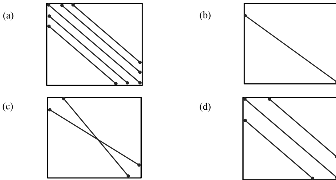
Figure 2-10. Alternative models with off-diagonal struts to model the frame infill interaction proposed by (a) Syrmakezis and Vratsanou (1986), (b) Zarnic and Tomazevic (1988), (c) Schmidt (1989), (d) Chrysostomou (1991). For clarity, struts in only one direction are shown.
