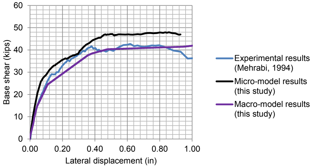
Figure 4-17. Macro-model, micro-model, and experimental results for Specimen 8 . The experiment was carried out to a lateral displacement larger than 1.0 inches. Results are compared here until 1.0 inches, because the micro-model failed to converge before that point.
