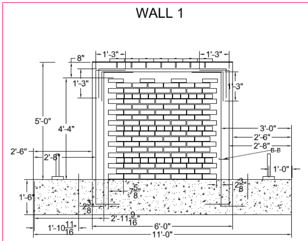
Figure 3-5. CM Wall 1 assembly drawing
