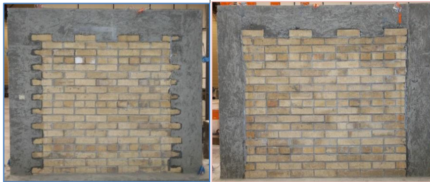
Figure 3-12. Concrete tie elements
