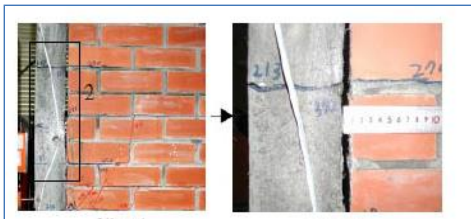
Figure 2-7. In plane flexural failure in CM (EERI, 2010)
