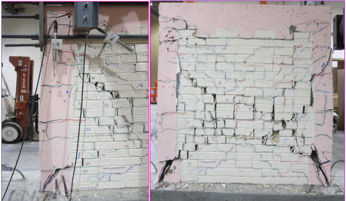
Figure 3-60. CM shear wall 2 failure mechanism
