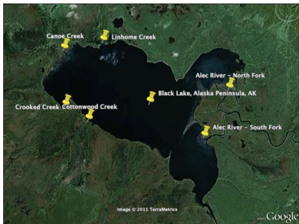
Figure 3.2: Map of Black Lake Depicting Tributaries (Google Earth Pro, 2011)
