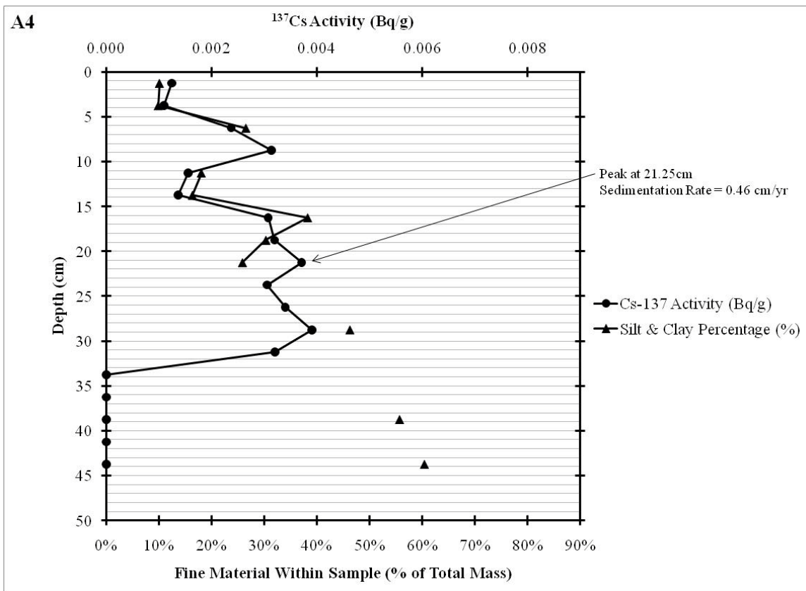
Figure 4.14: A4 137 Cs vs Depth and Fine Material Percentage vs Depth
