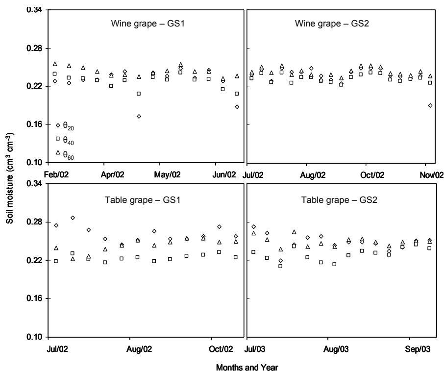
Figure 5.1 Soil moisture ( \theta_i ) at different depths ( i = 20, i = 40 and i = 60\text{cm} ), during the first (GS1) and second (GS2) growing seasons of wine and table grapes.
