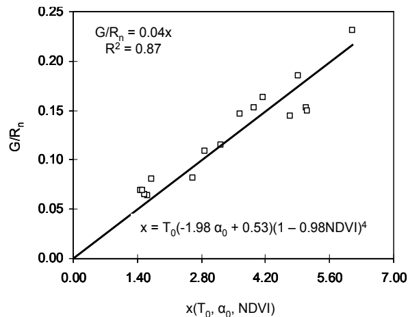
Figure 8.8. Relationship between the ratio of soil heat flux (G) over net radiation ( R_n ); and surface temperature ( T_0 ), surface albedo ( \alpha_0 ) and the Normalized Difference Vegetation Index (NDVI)
