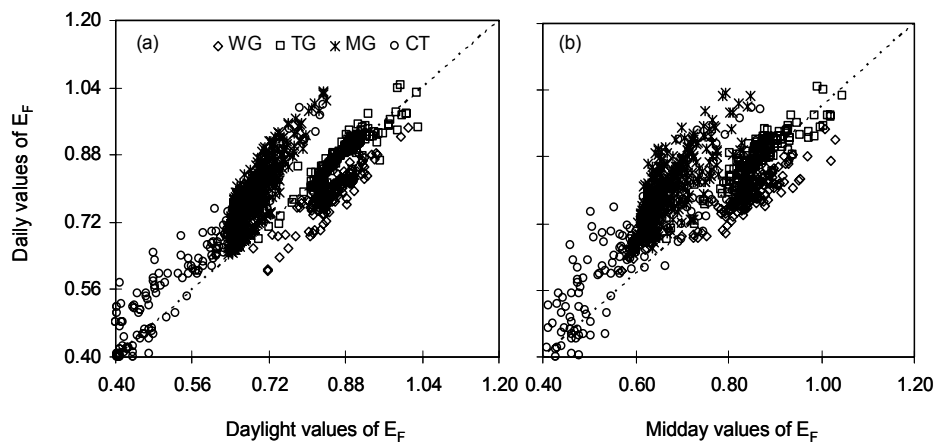
Figure 7.7. Relationships between the values E_{F_{24}} vs. E_{F_{\text{daylight}}} (a) and of E_{F_{24}} vs. E_{F_{12}} values (b) for wine grape (WG), table grape (TG), mango orchard (MG) and caatinga (CT).
