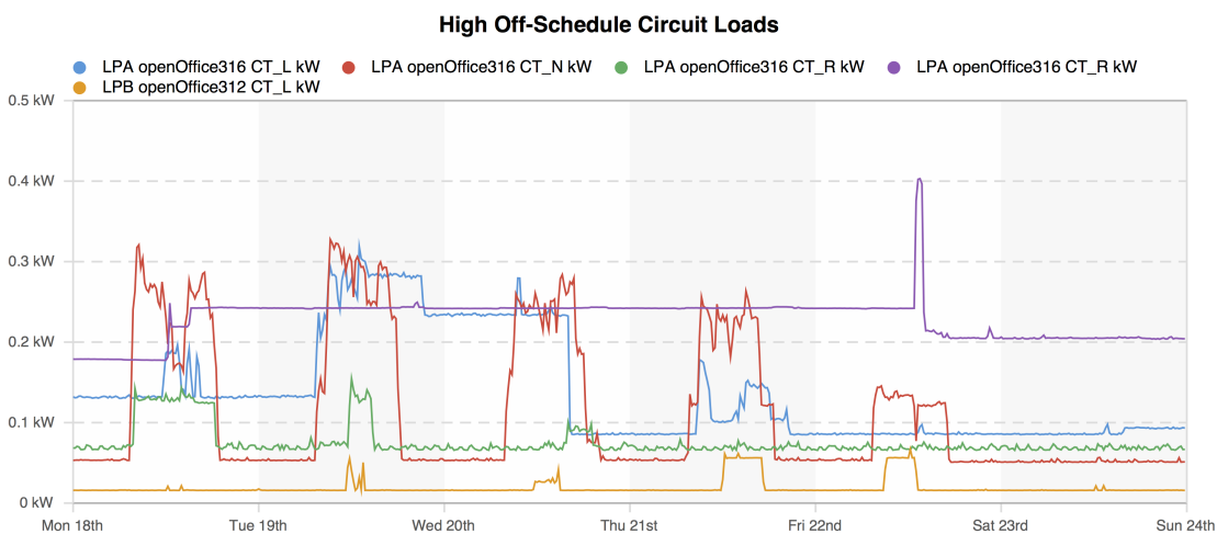
Figure 5.8: Drill down of power intensity for open and private offices
