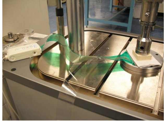
Figure 4.5. Instron loading machine test setup.
