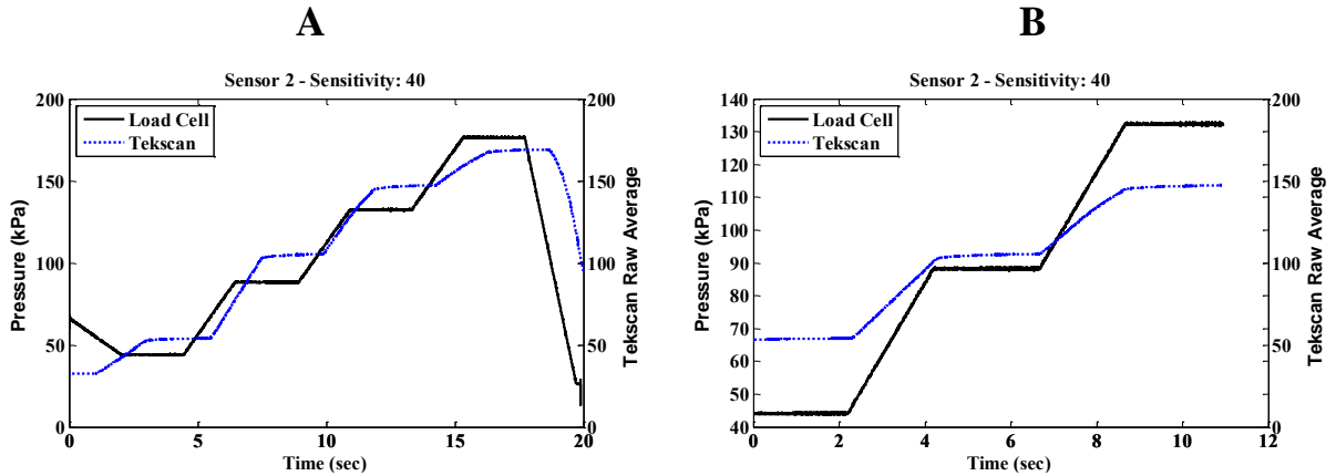
Figure 5.1. Loading machine load cell measurement versus pressure sensor reading during a loading machine test: (a) raw records; (b) data sets aligned and trimmed.
