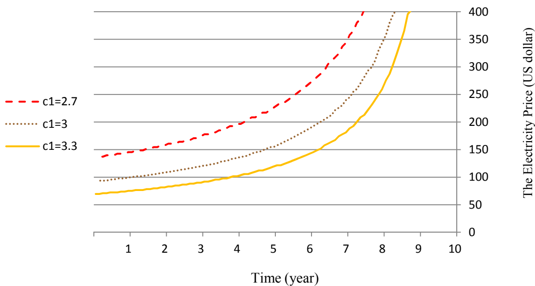
Figure 4.5. Free Boundary for Abandonment with Different c_1
