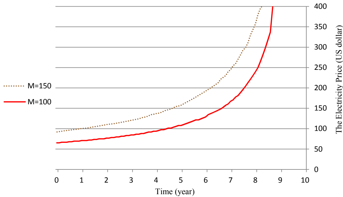
Figure 4.3. Free Boundary for Abandonment with Different M
