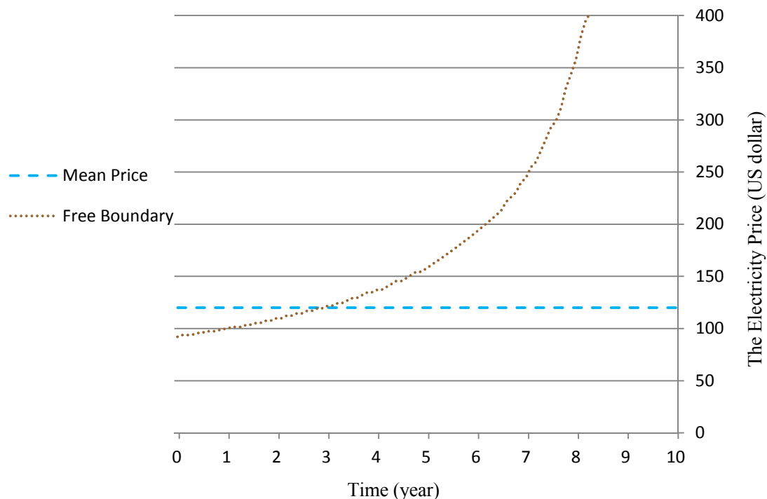
Figure 4.1. Free Boundary for Abandonment
