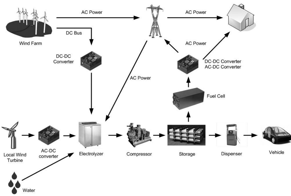
Figure 5.1. Wind-Hydrogen System
